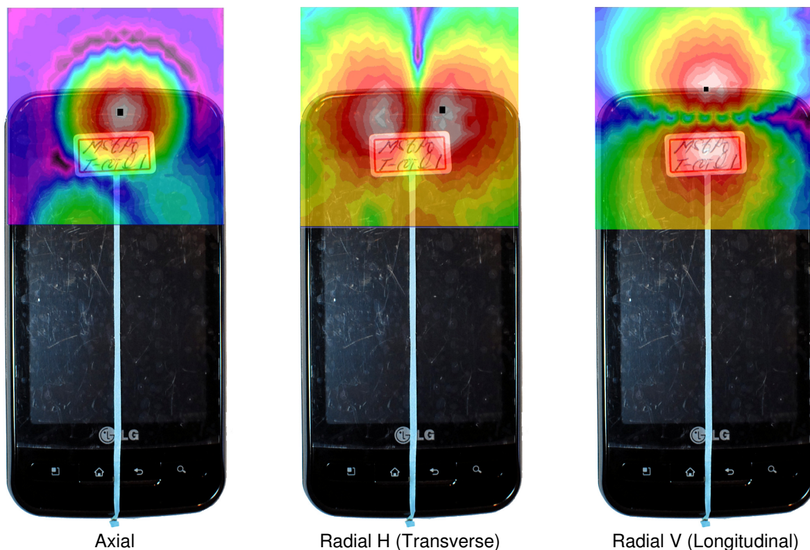
Figure 13-3 T-Coil Scan Overlay Magnetic Field Distributions
