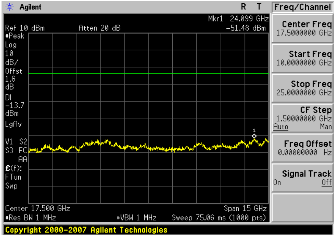
Plot 6-19. Conducted Spurious Plot (Bluetooth, 2Mbps – Ch. 0)
