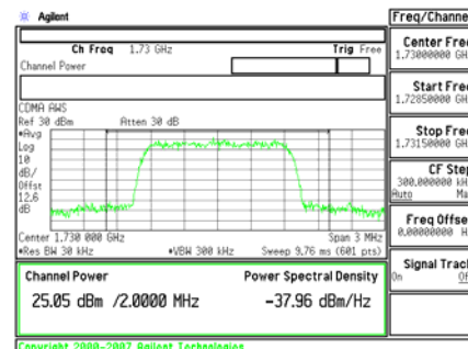
Figure 8-2 Wireless Device Modulated Signal
