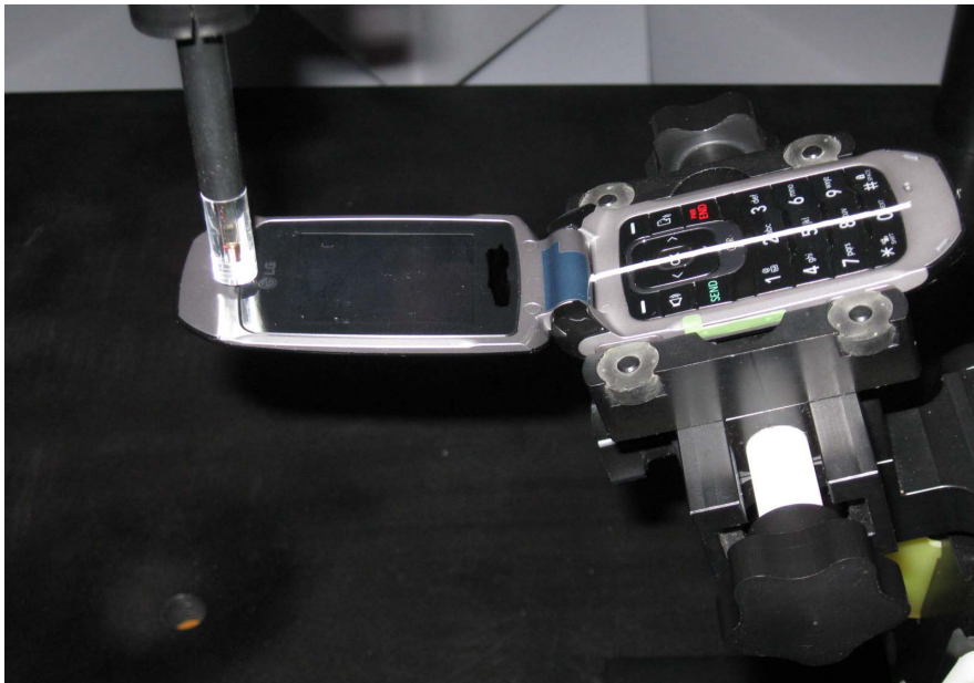
Figure 13-2 Test Setup for Wireless Device
