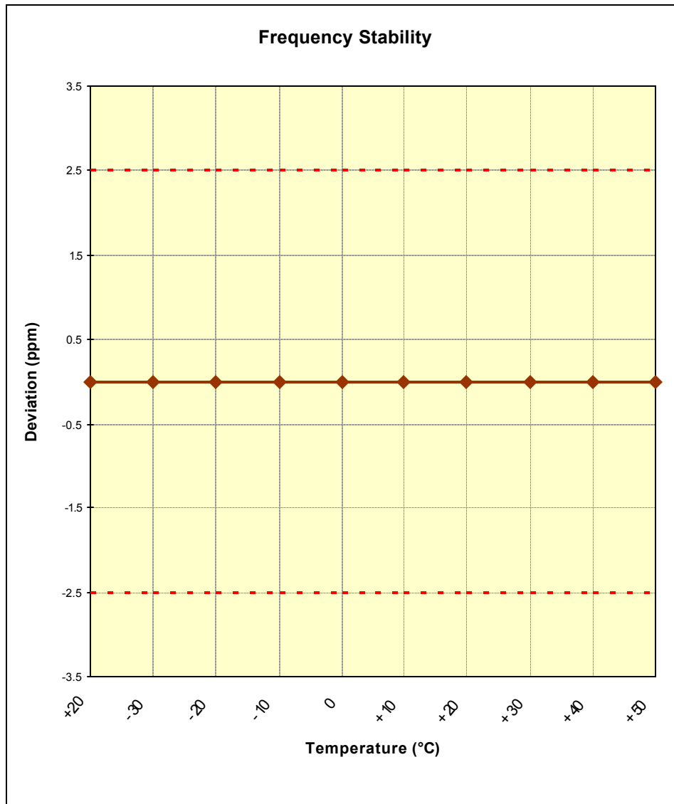
Figure 6-1. Frequency Stability Graph (AWS CDMA Mode – Ch. 450)
