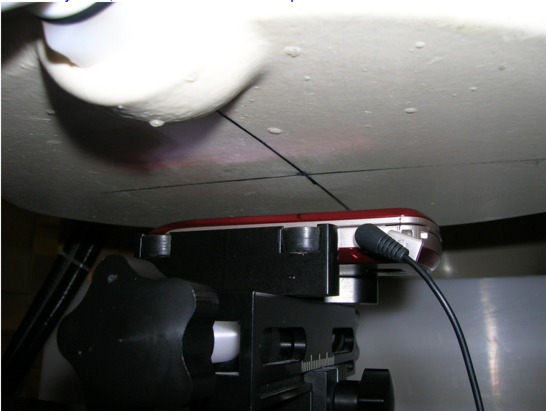
10. Body SAR, Front Side with 2.0 cm Space
