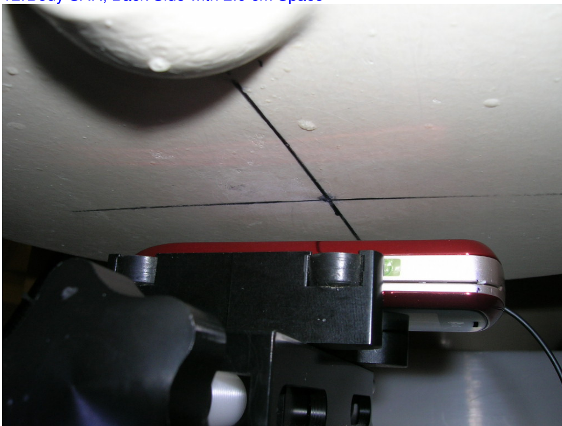
12.Body SAR, Back Side with 2.0 cm Space
