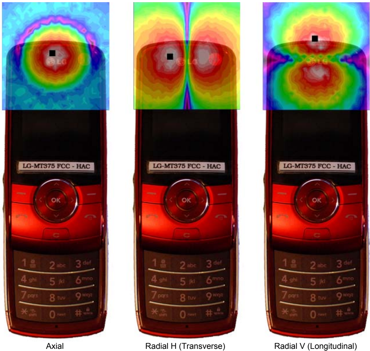
Figure 13-3 T-Coil Scan Overlay Magnetic Field Distributions
