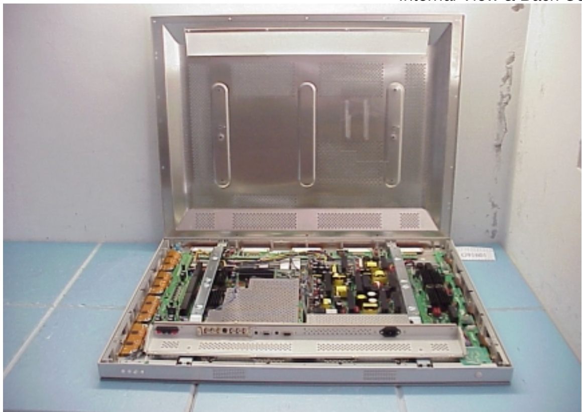
Figure 4 Internal View & Back Cover
