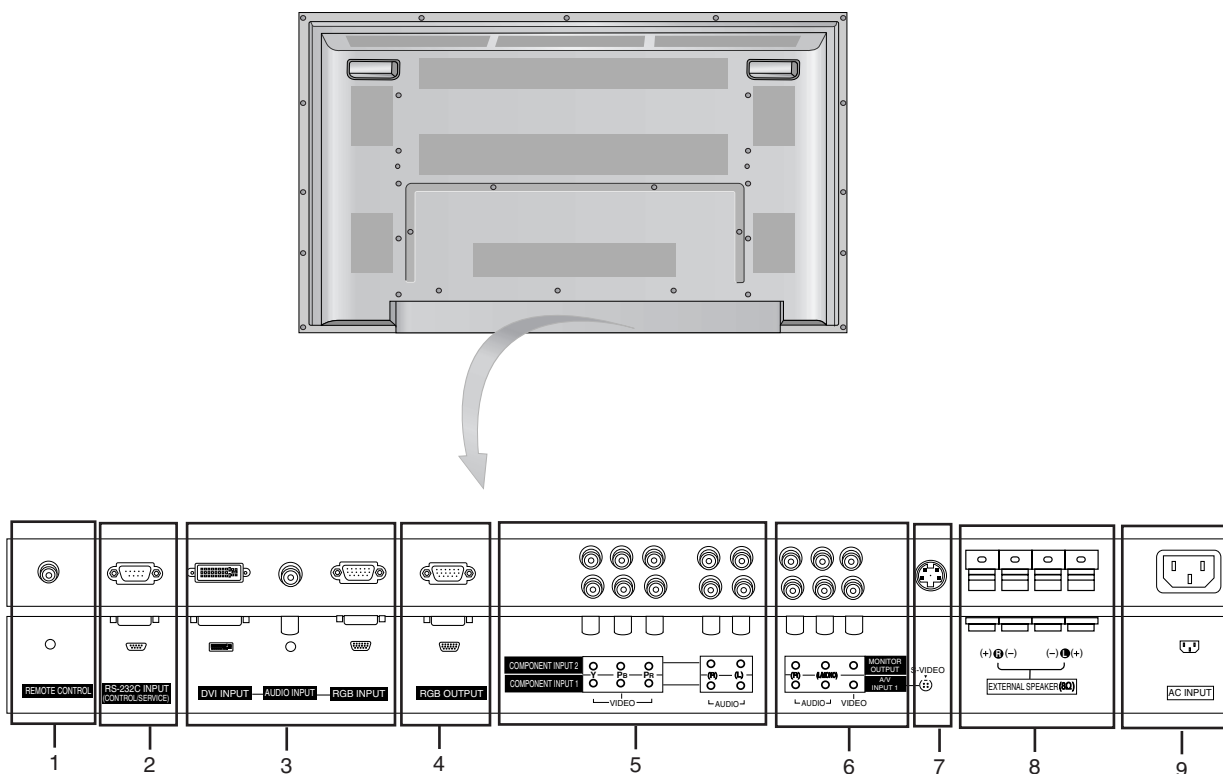
Back Connection Panel
