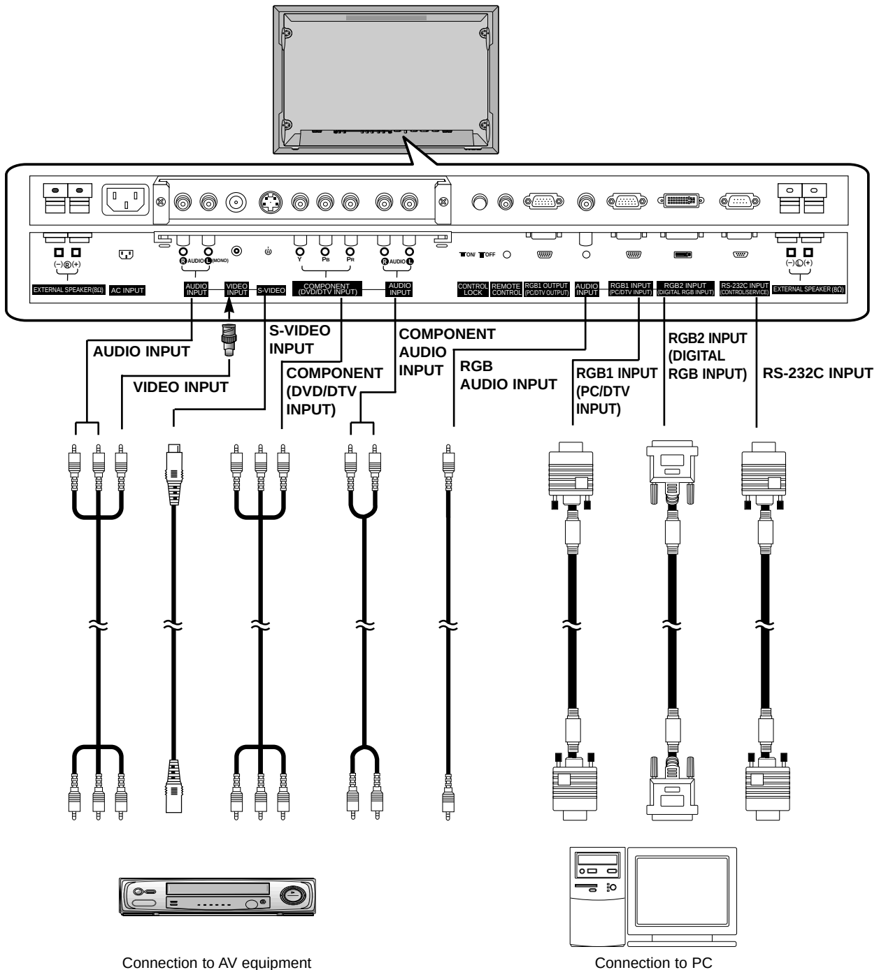
Monitor External Equipment Connection Panel
