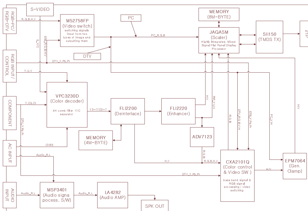
VSC board Block Diagram
