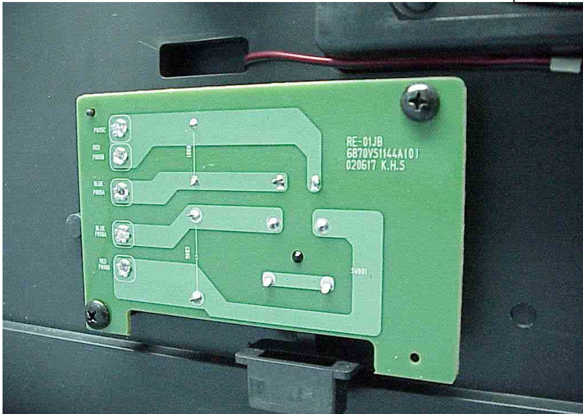
Figure 57 SW Board (Solder Side)
