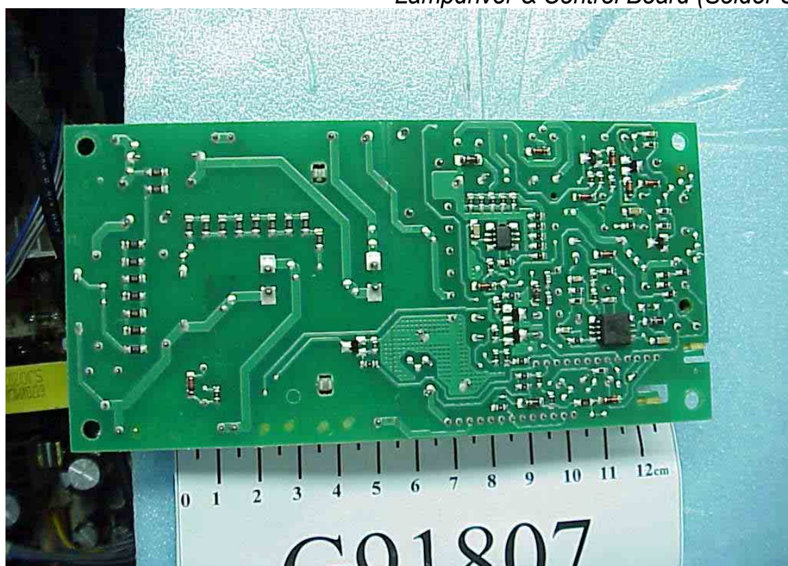
Figure 48 Lampdriver & Control Board (Solder Side)
