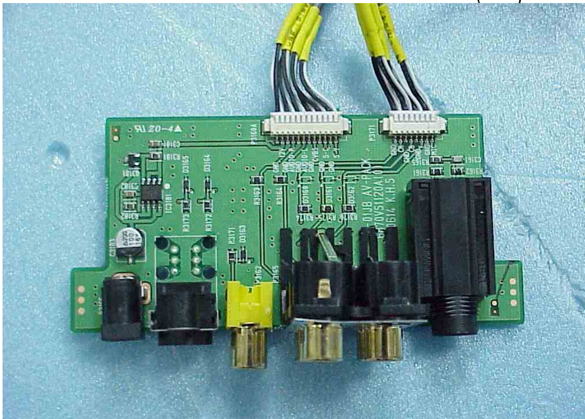
A/V Control Board (Component Side)
