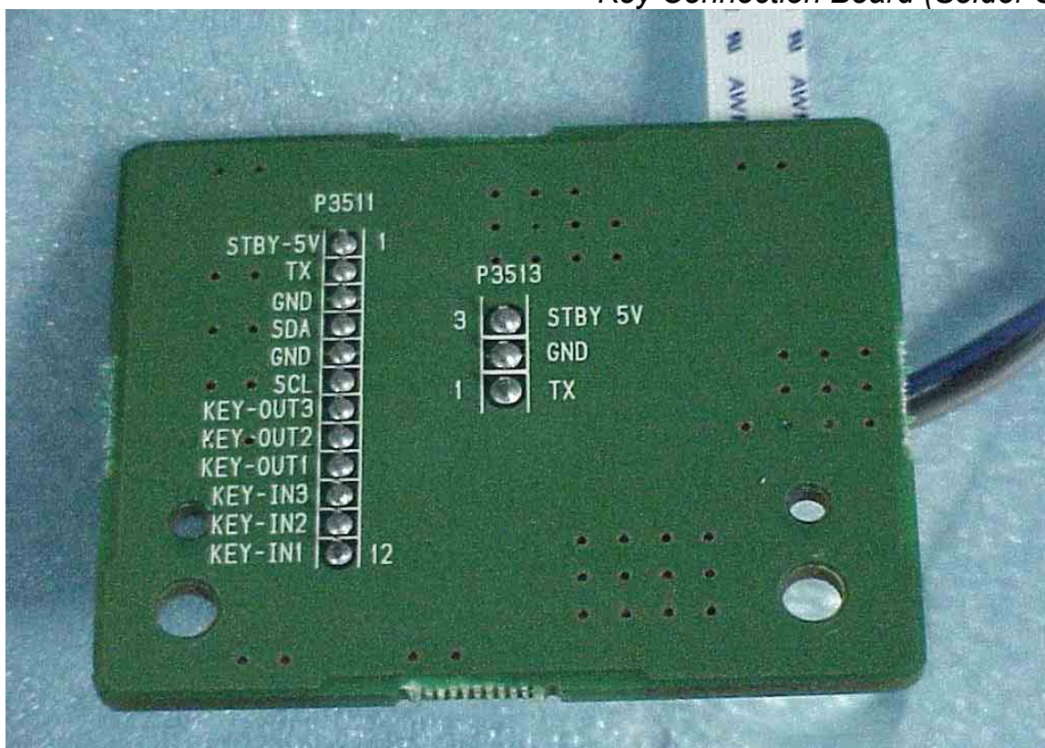
Figure 22 Key Connection Board (Solder Side)
