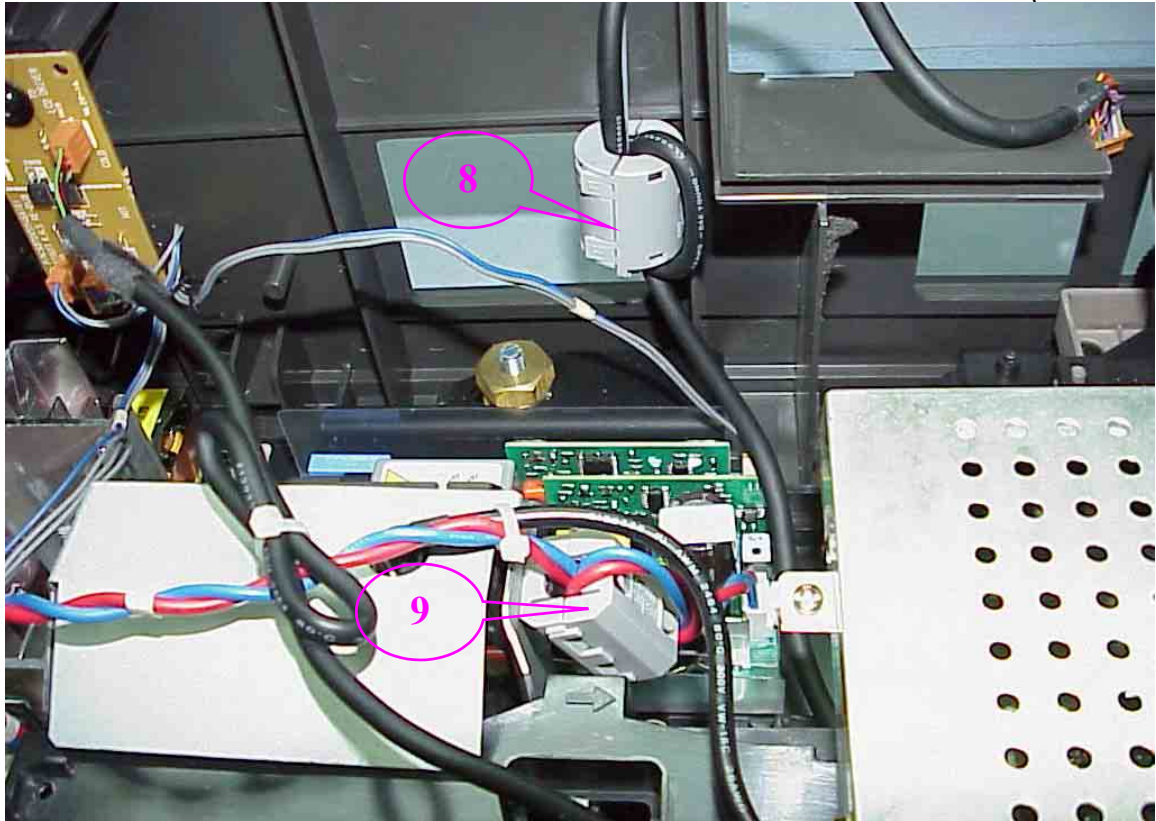
Figure 27 Internal View (EMI Cores)
