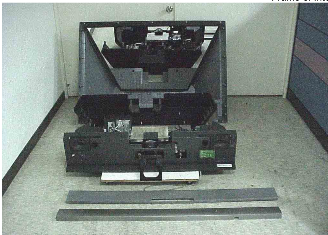
Figure 13 Frame of Internal
