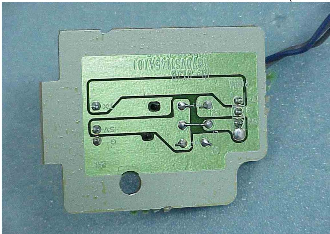
Figure 20 Remote Control Receiver Board (Solder Side)
