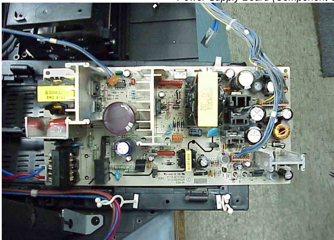
Figure 53 Power Supply Board (Component Side)
