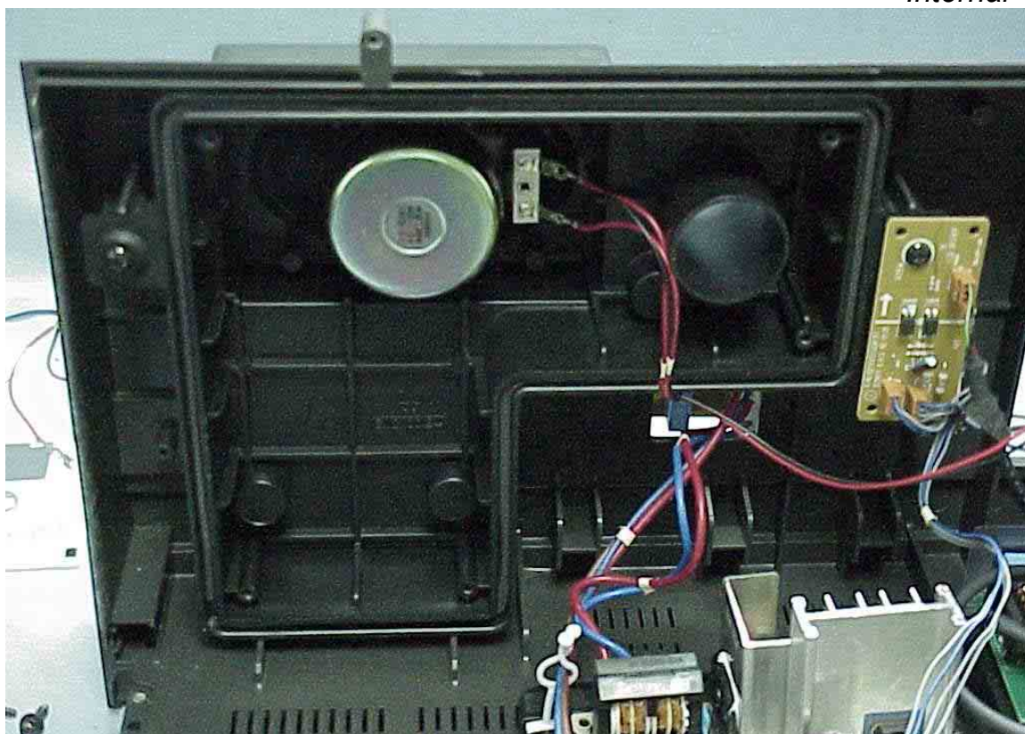
Figure 55 Internal View
