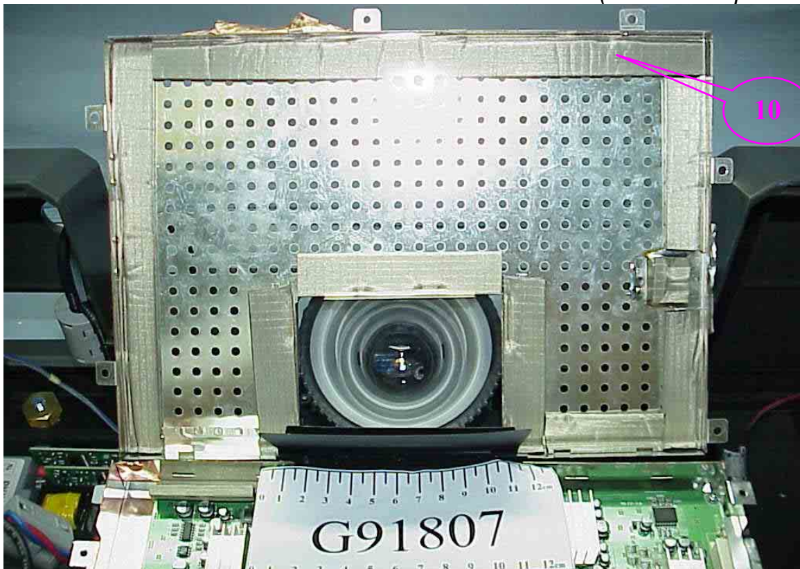
Figure 29 Frame of Internal (Lens & Lamp Module)
