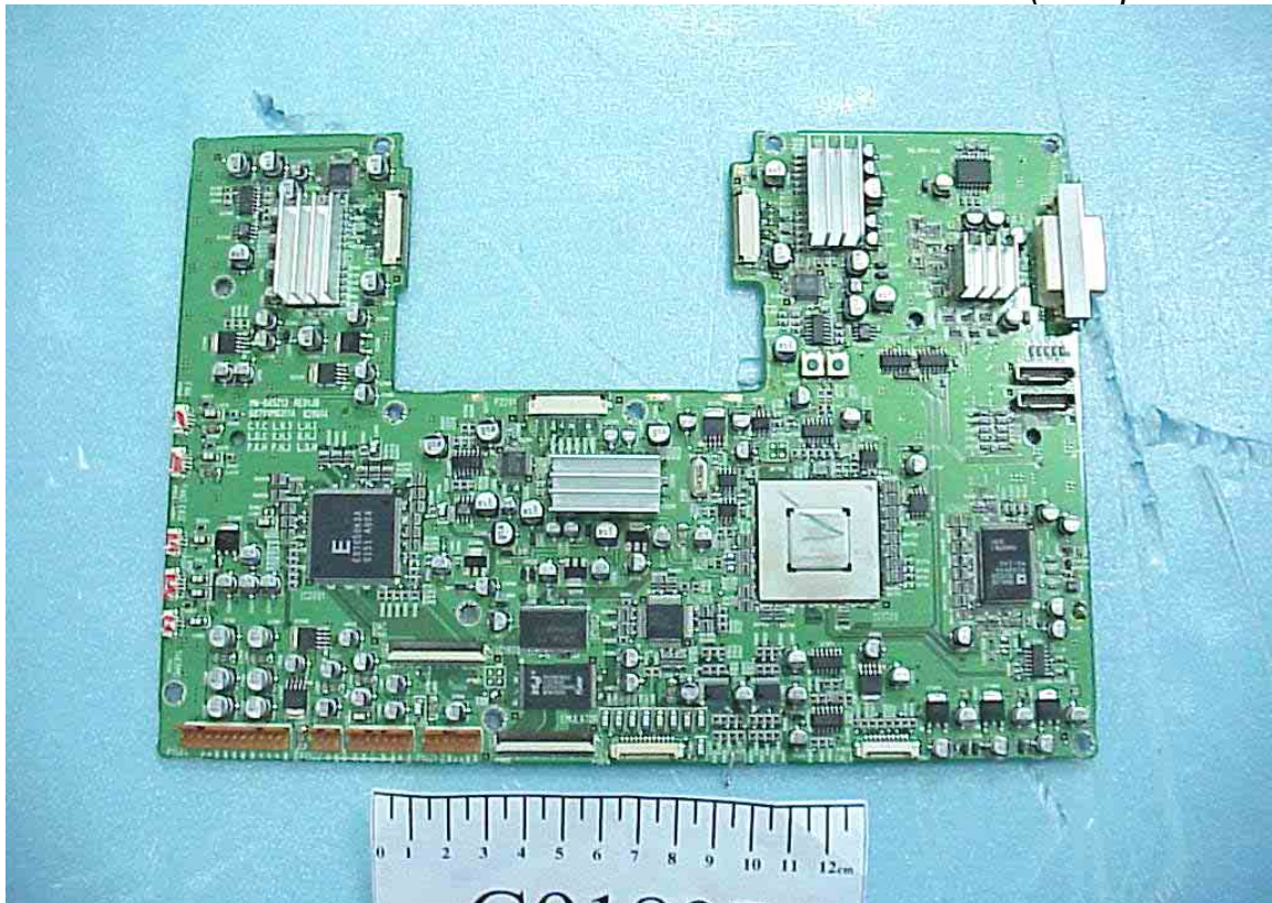
Figure 41 Main Board (Component Side)
