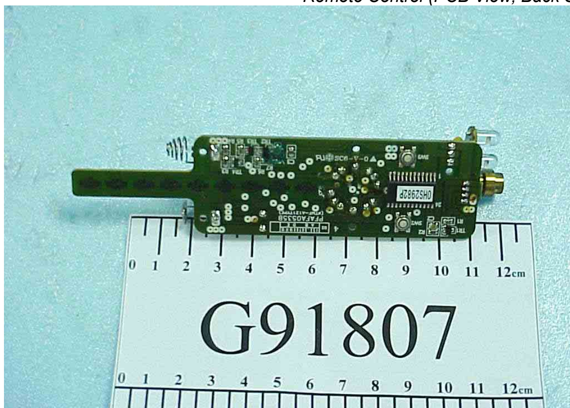
Figure 63 Remote Control (PCB View, Back Side)
