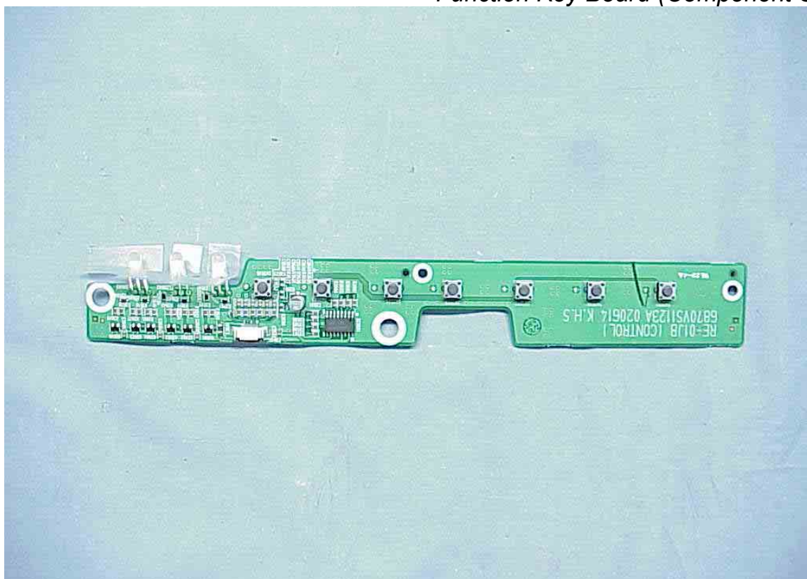
Figure 25 Function Key Board (Component Side)
