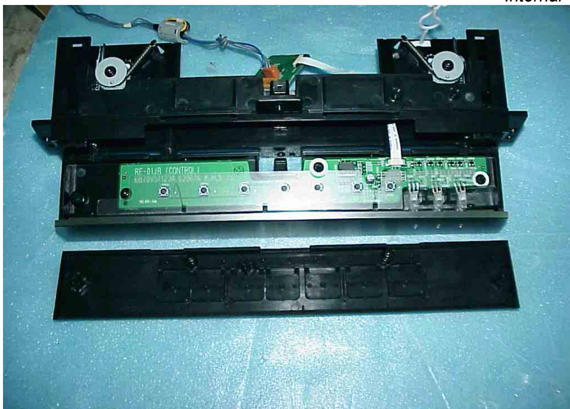
Figure 24 Internal View
