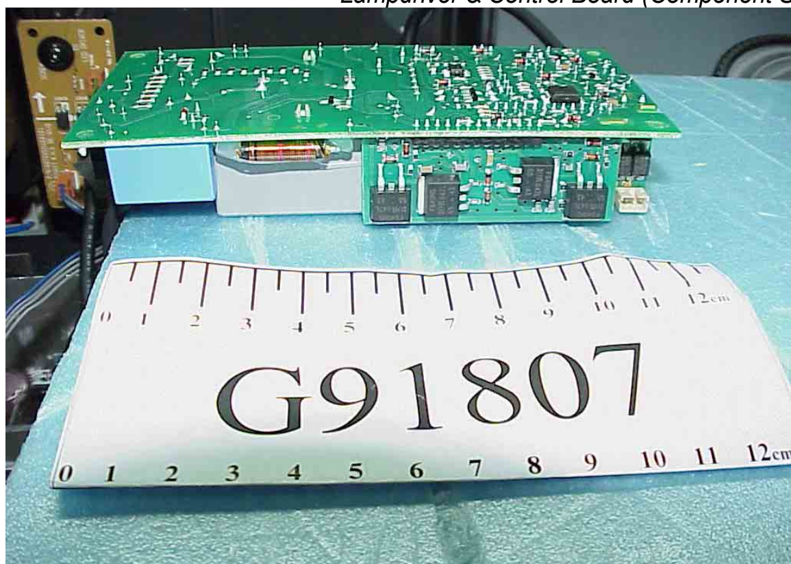
Figure 47 Lampdriver & Control Board (Component Side)
