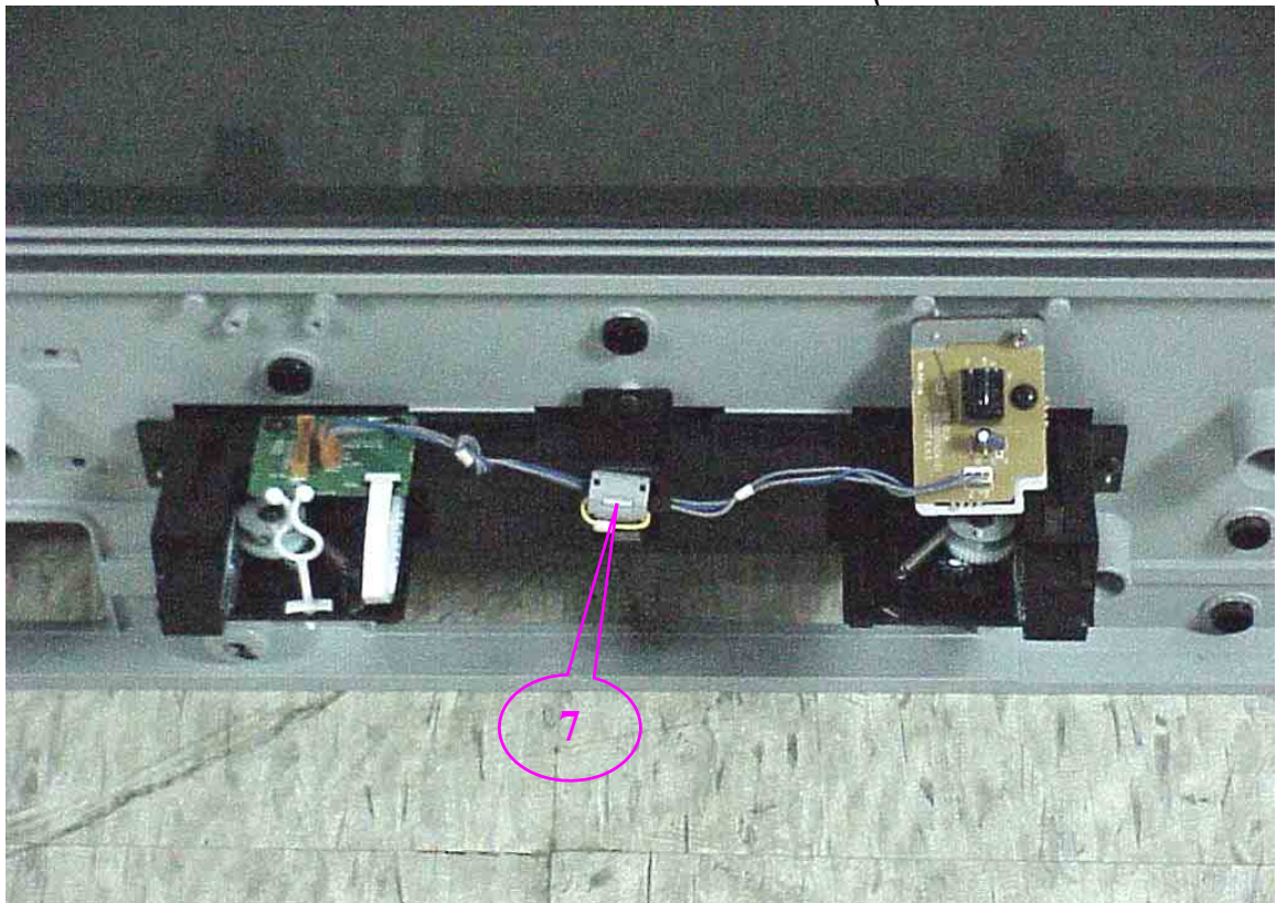
Figure 16 Internal View (Control Board & EMI Core)
