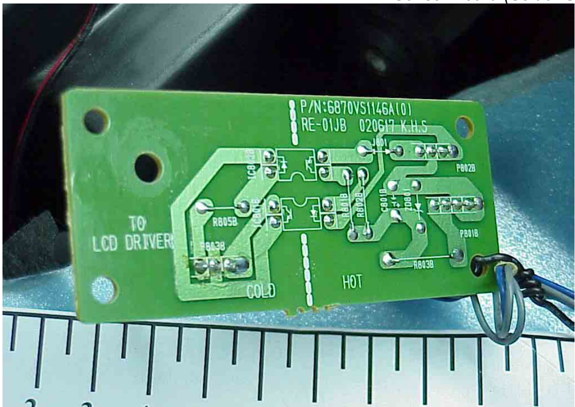
Figure 50 Sensor Board (Solder Side)
