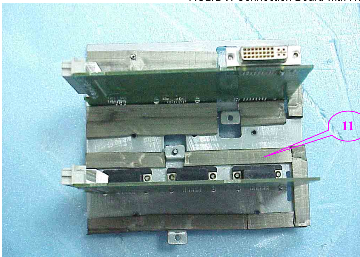
Figure 37 RGB/DVI Connection Board with Holder
