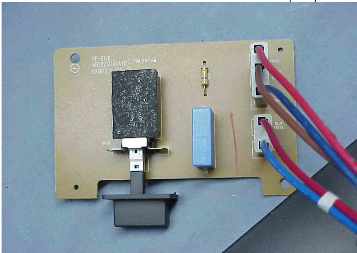
Figure 58 SW Board (Component Side)
