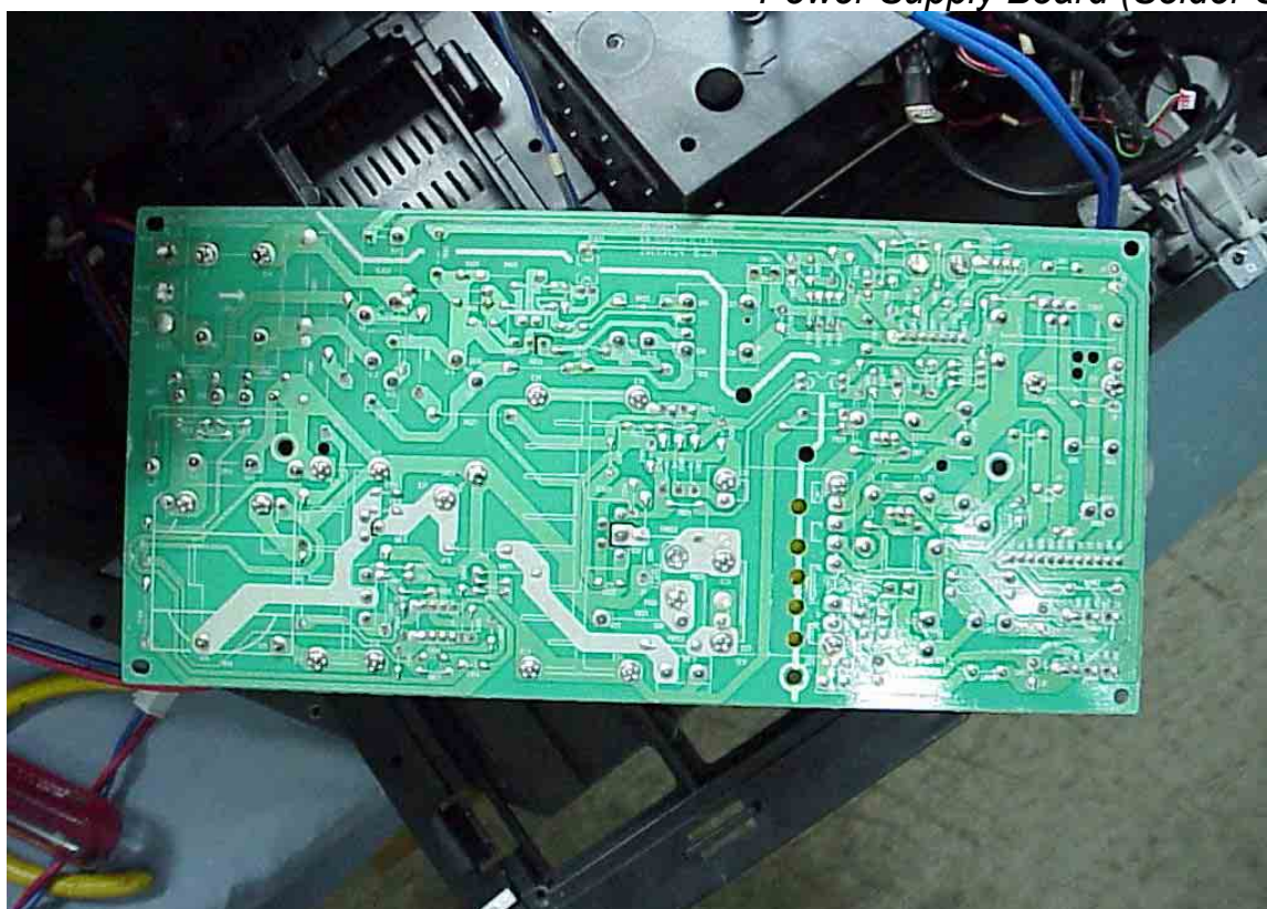
Figure 54 Power Supply Board (Solder Side)
