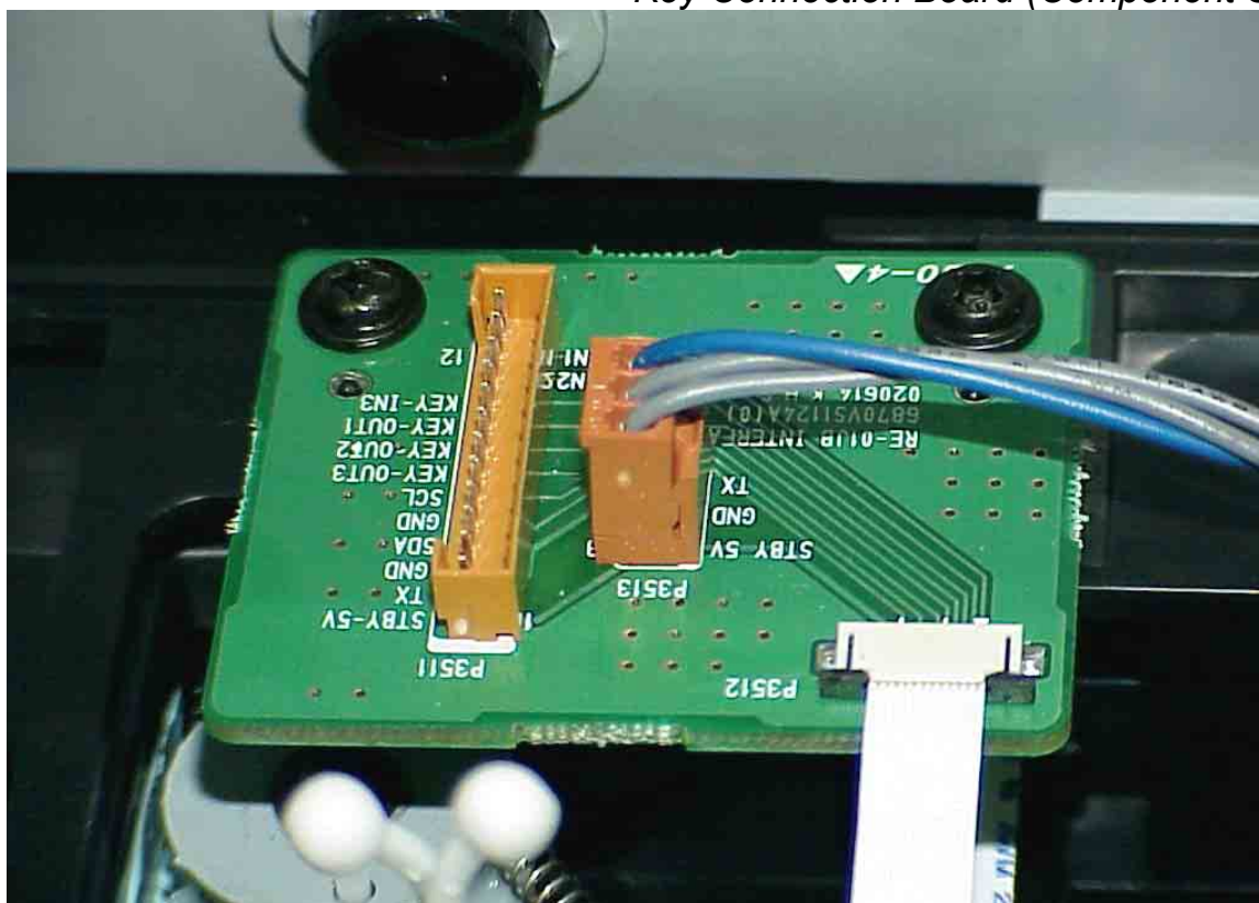
Figure 21 Key Connection Board (Component Side)
