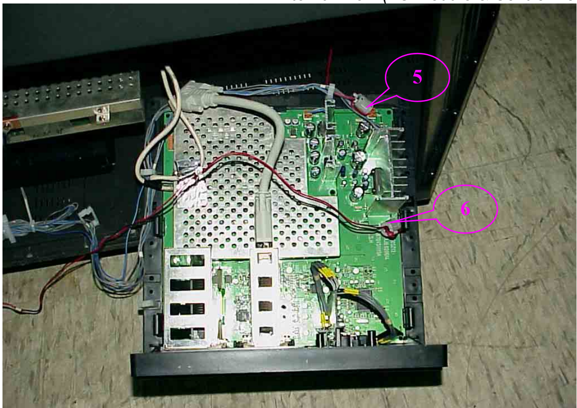
Figure 12 Internal View (I/O Module & Control Board)
