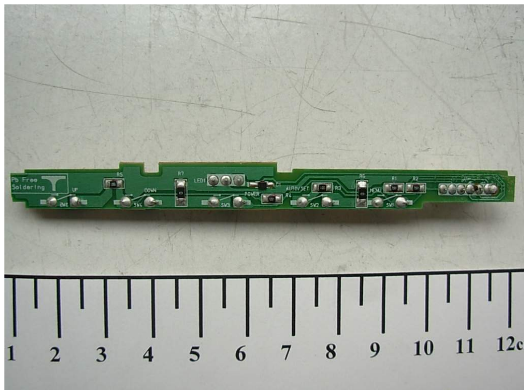
FIGURE 4 LCD MONITOR (M/N: N1742LT) KEY BOARD (SOLDERED SIDE)
