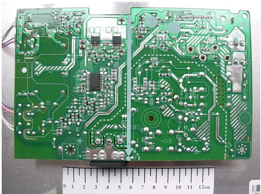
FIGURE 6 LCD MONITOR (M/N: N1742LT) POWER BOARD (SOLDERED SIDE)
