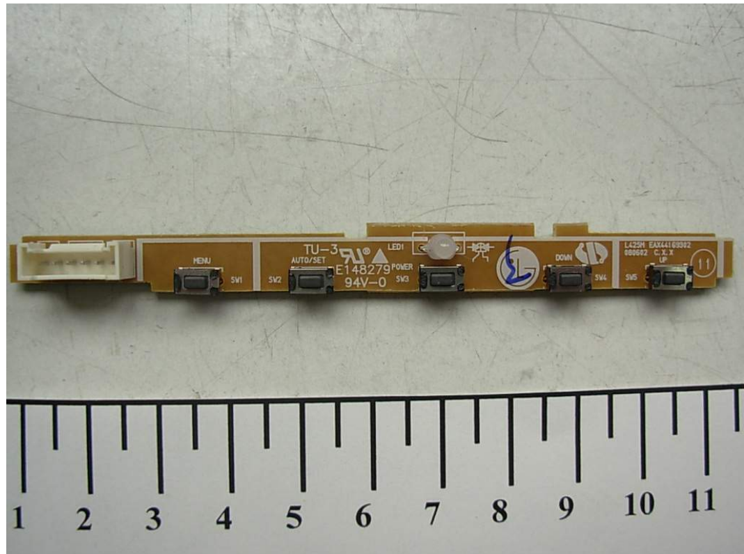
FIGURE 3 LCD MONITOR (M/N: N1742LT) KEY BOARD (COMPONENT SIDE)
