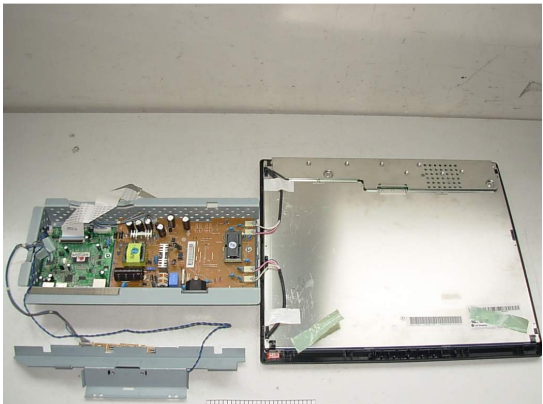
FIGURE 2 LCD MONITOR (M/N: N1742LT) BOARDS REMOVED
