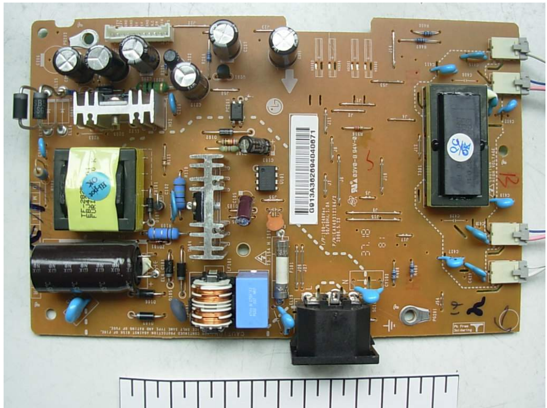
FIGURE 5 LCD MONITOR (M/N: N1742LT) POWER BOARD (COMPONENT SIDE)
