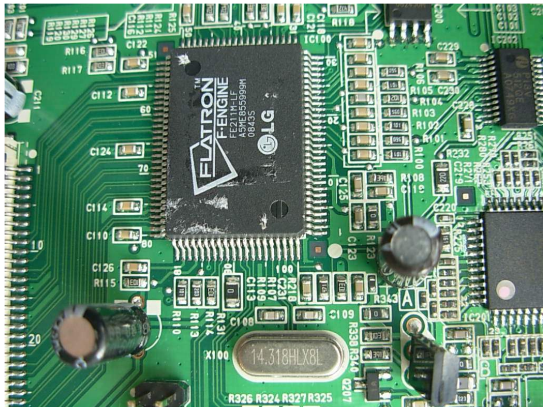
FIGURE 9 LCD MONITOR (M/N: N1742LT) CHIP 1 & CRYSTAL ON MAIN BOARD
