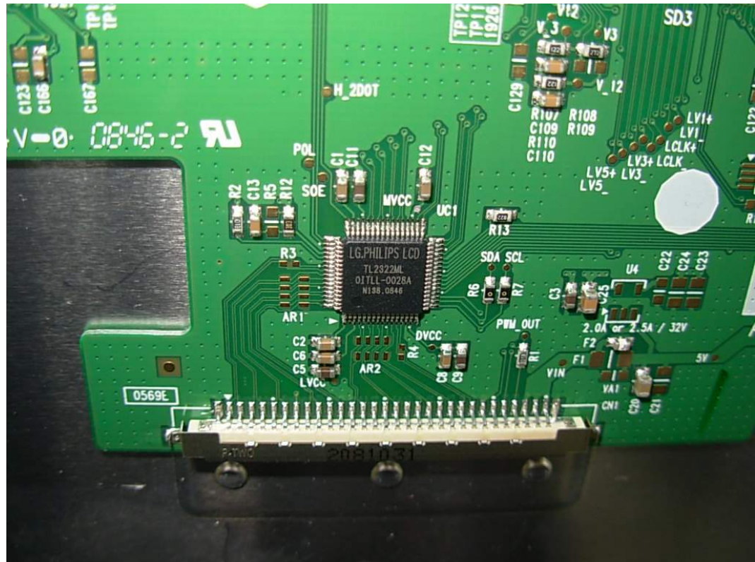
FIGURE 15 LCD MONITOR (M/N: N1742LT) CHIP ON LCD PANEL MAIN BOARD
