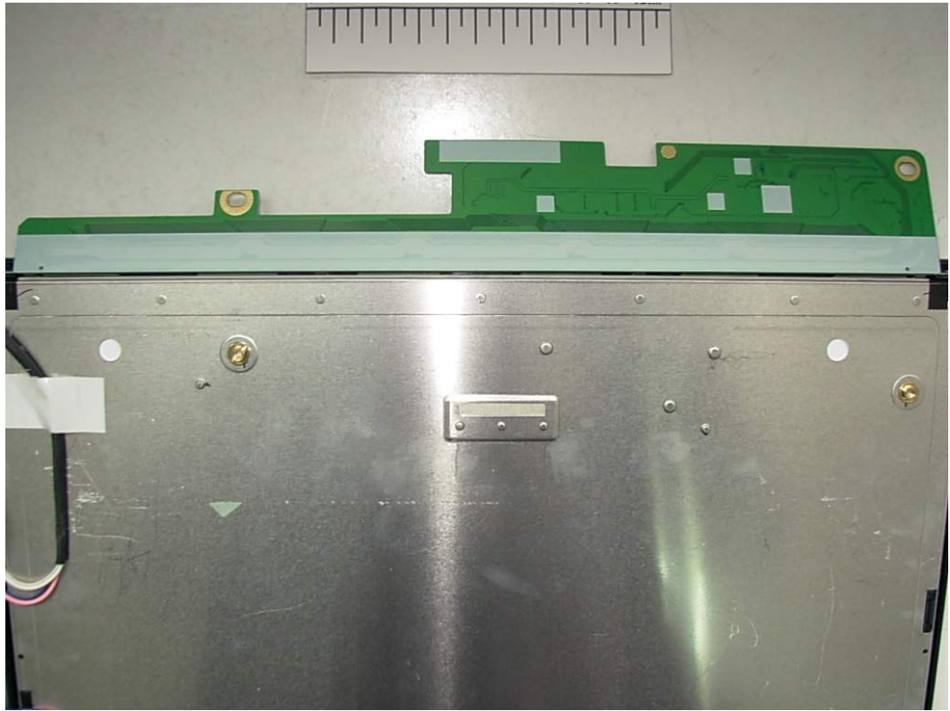
FIGURE 13 LCD MONITOR (M/N: N1742LT) LCD PANEL MAIN BOARD (SOLDERED SIDE)
