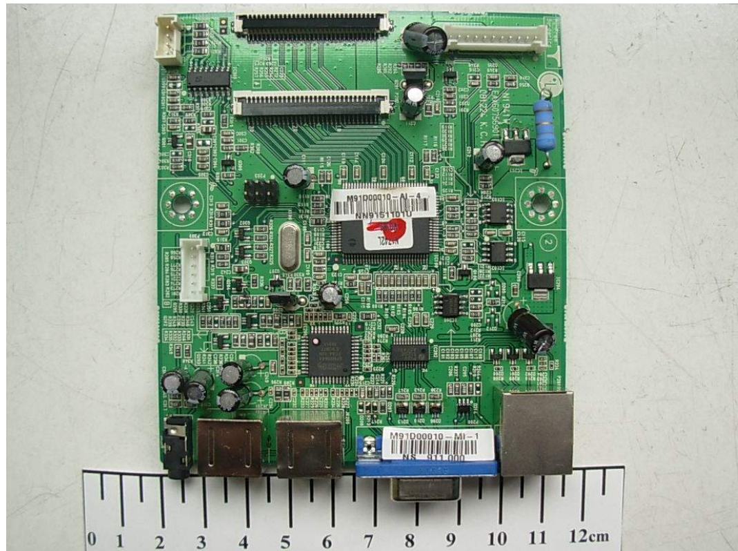
FIGURE 7 LCD MONITOR (M/N: N1742LT) MAIN BOARD (COMPONENT SIDE)
