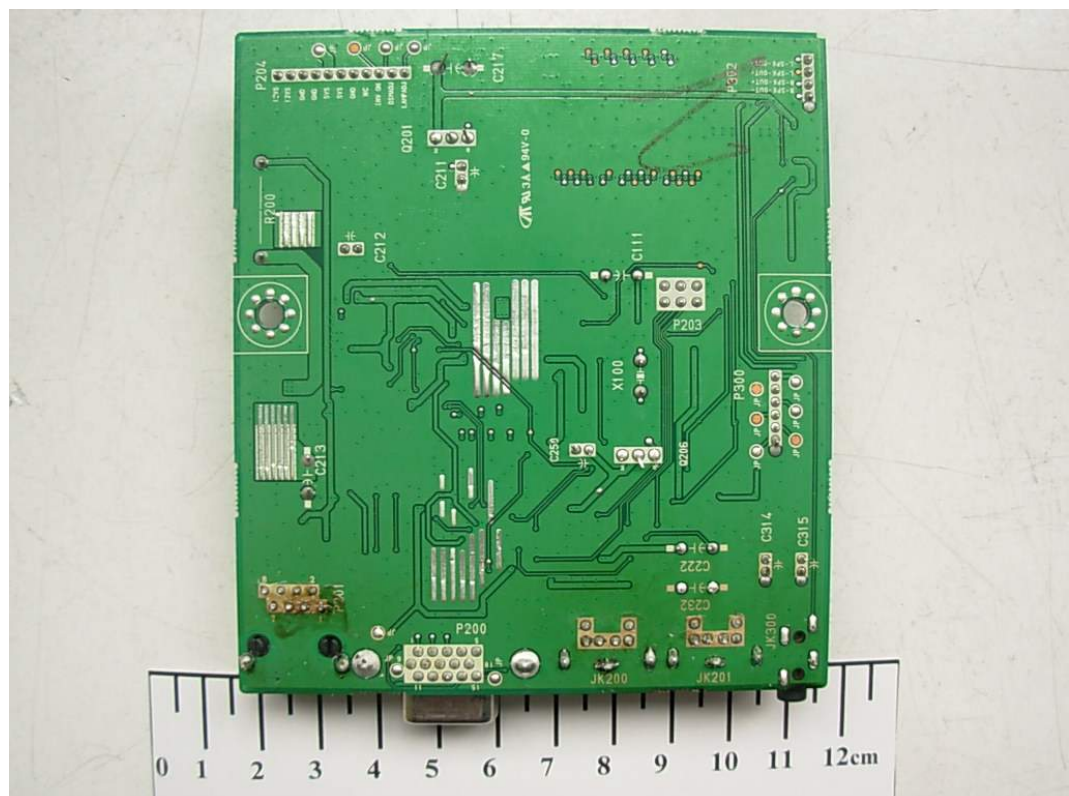
FIGURE 8 LCD MONITOR (M/N: N1742LT) MAIN BOARD (SOLDERED SIDE)
