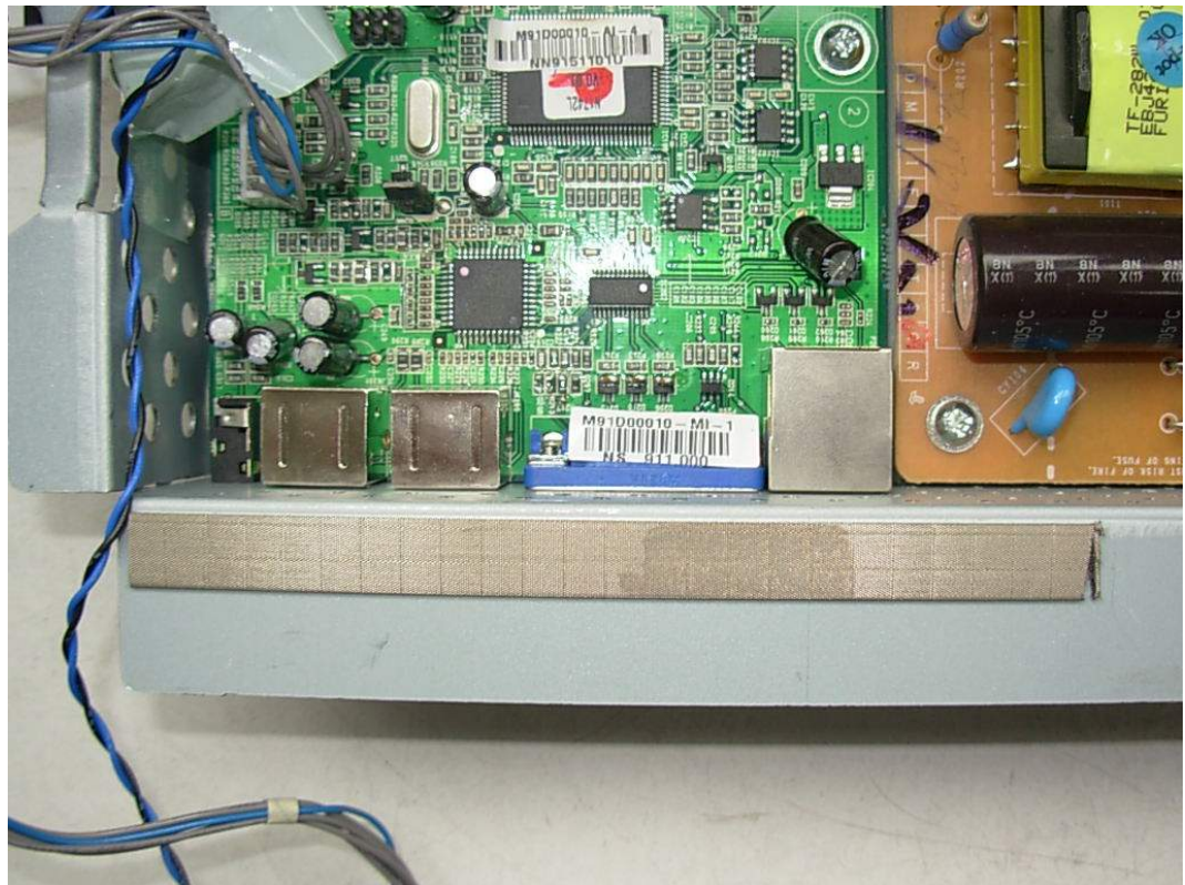
FIGURE 17 LCD MONITOR (M/N: N1742LT) DEBUG #2
