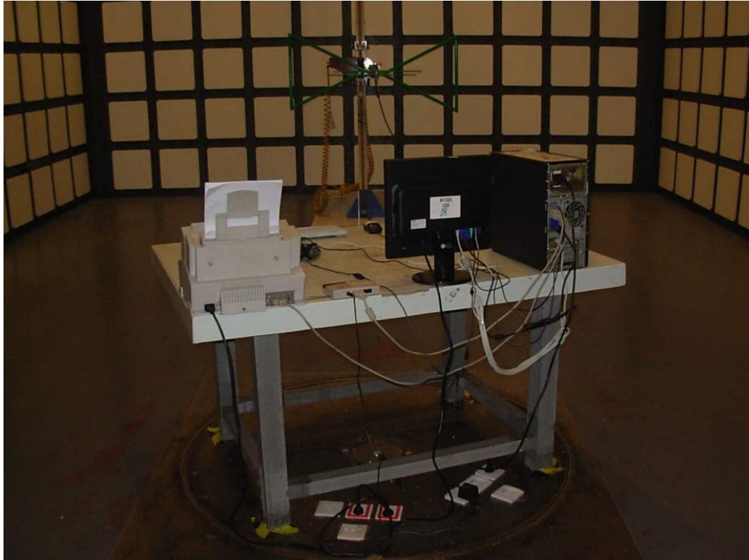
SETUP WITH MAXIMUM DETECTED EMISSION AT HORIZONTAL POLARIZATION (X-PORT 1280*1024@60Hz)
