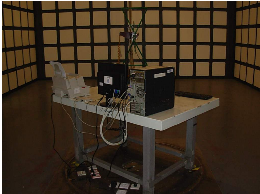
SETUP WITH MAXIMUM DETECTED EMISSION AT VERTICAL POLARIZATION (X-PORT 1280*1024@60Hz)
