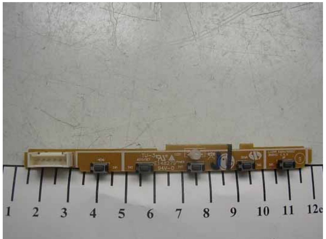
FIGURE 3 NETWORK MONITOR (M/N: N1942LT) KEY BOARD (COMPONENT SIDE)
