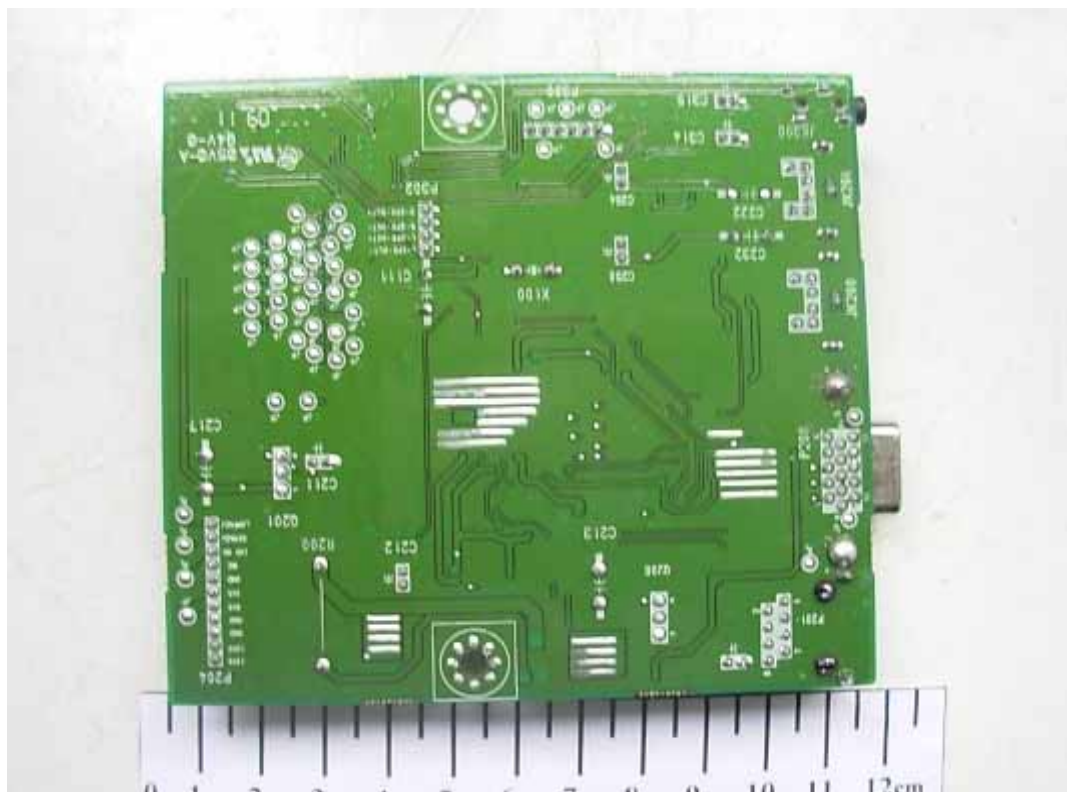
FIGURE 8 NETWORK MONITOR (M/N: N1942LT) MAIN BOARD (SOLDERED SIDE)
