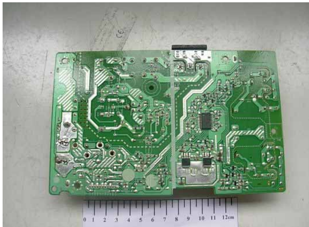
FIGURE 6 NETWORK MONITOR (M/N: N1942LT) POWER BOARD (SOLDERED SIDE)
