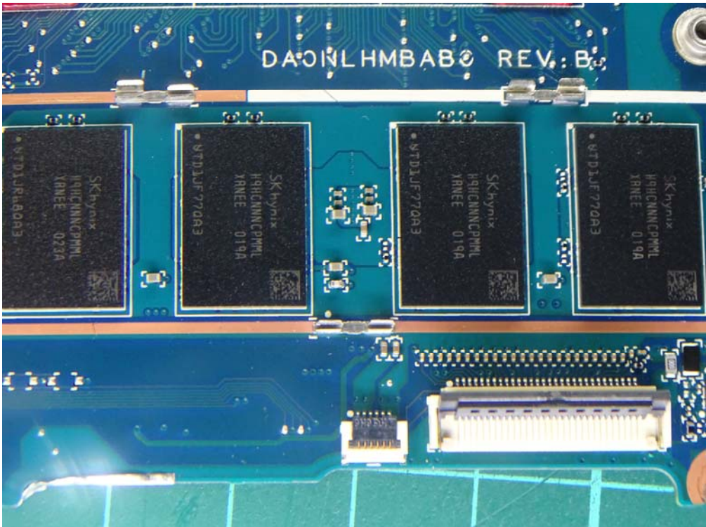
(45) EUT Photo
