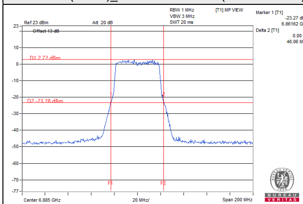
802.11ax (HE40)_Chain 1 / CH 187 (U-NII-7 Band)
