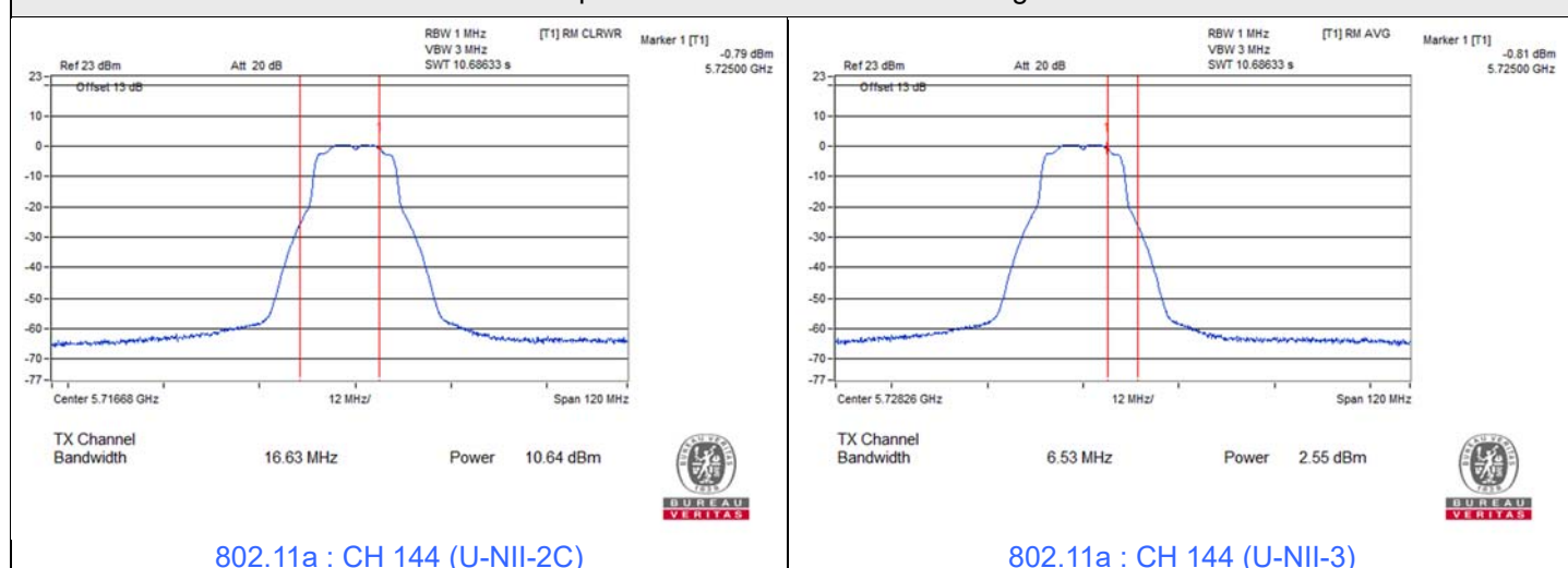
Spectrum Plot for channel straddling
