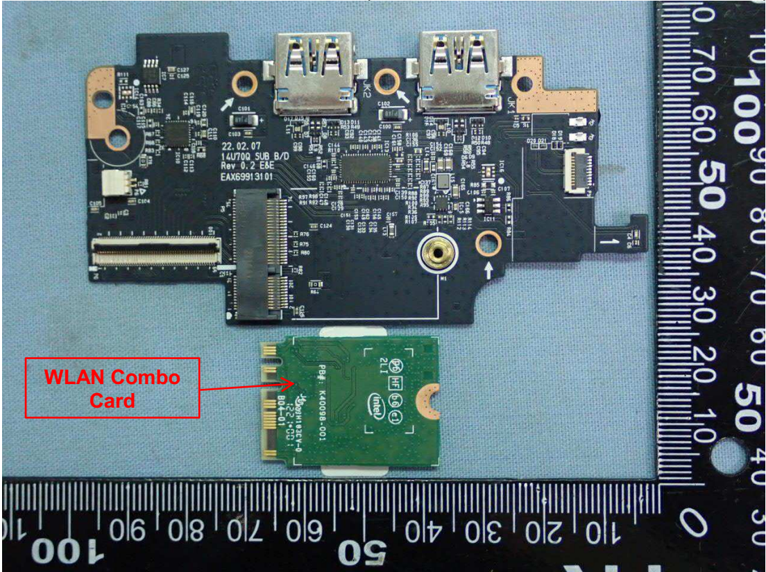
Figure 19 Internal View (WLAN SUB Bard, WLAN Combo CARD)
