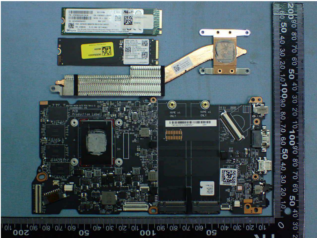
Figure 16 Internal View
