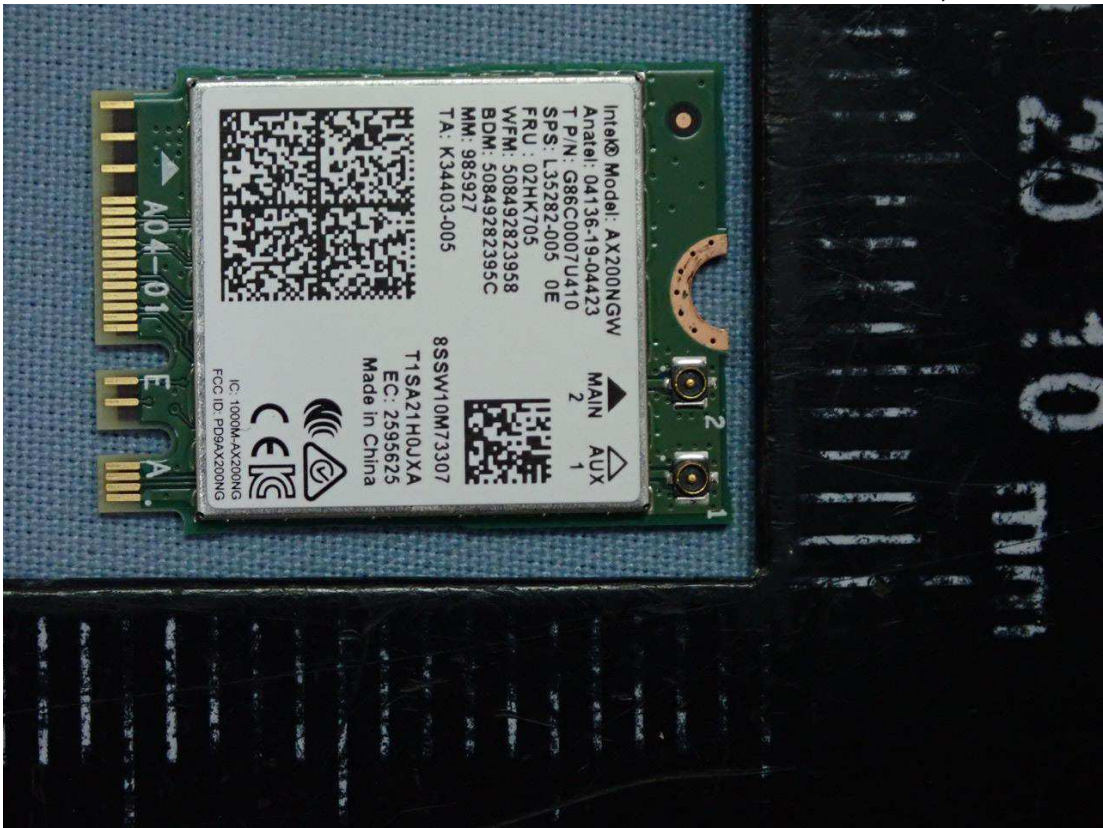
Figure 23 WLAN Combo Card, Front View
