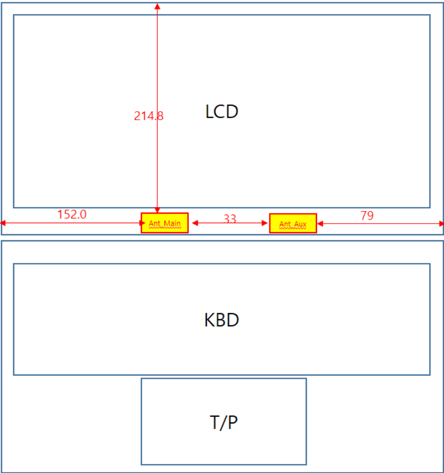
Figure 28 Internal View (Antenna Location)
