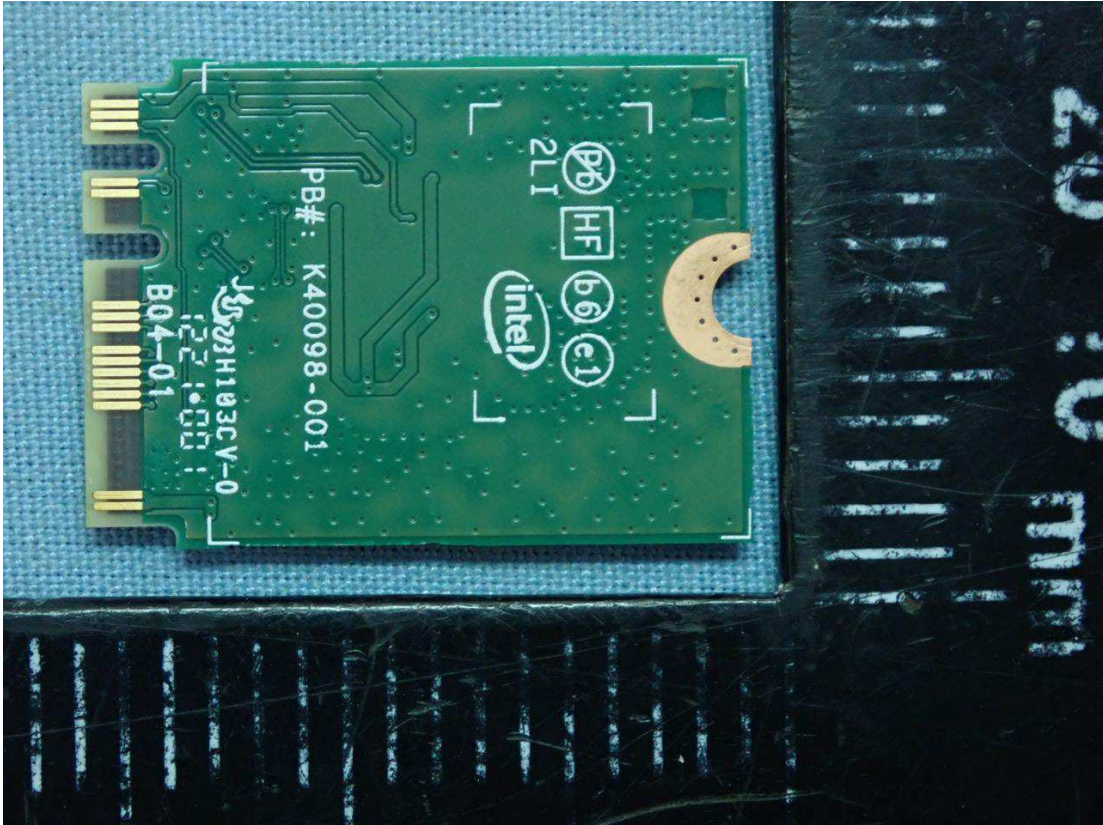
Figure 25 WLAN Combo Card, Back View
