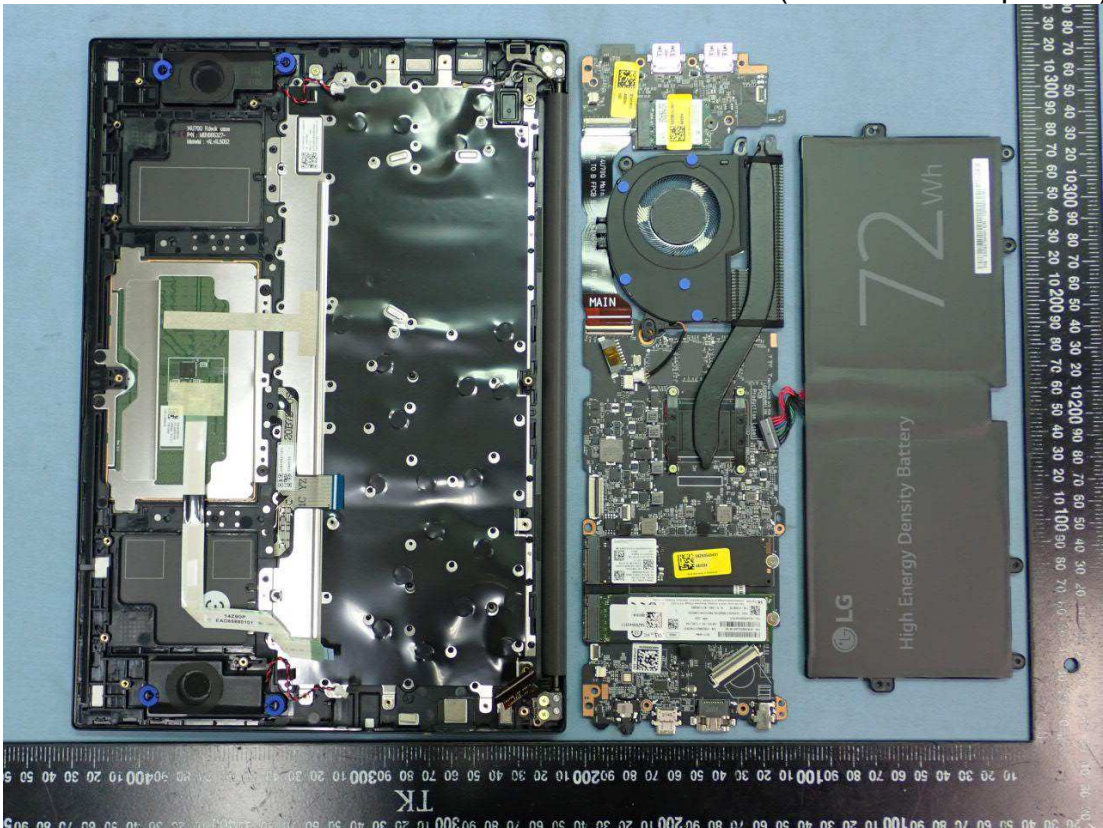
Figure 9 Internal View (Removed Component)
