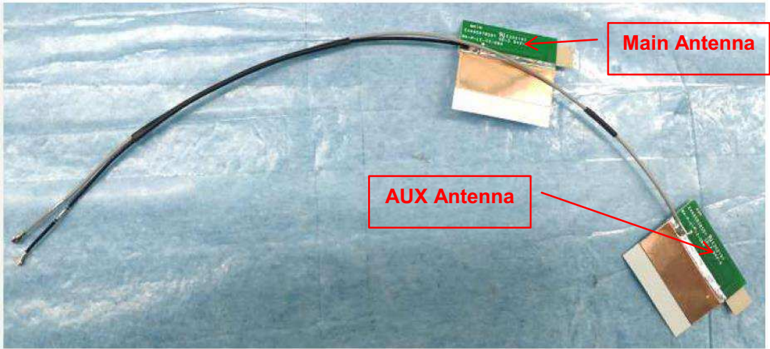
Figure 29 Antenna View, Front View
