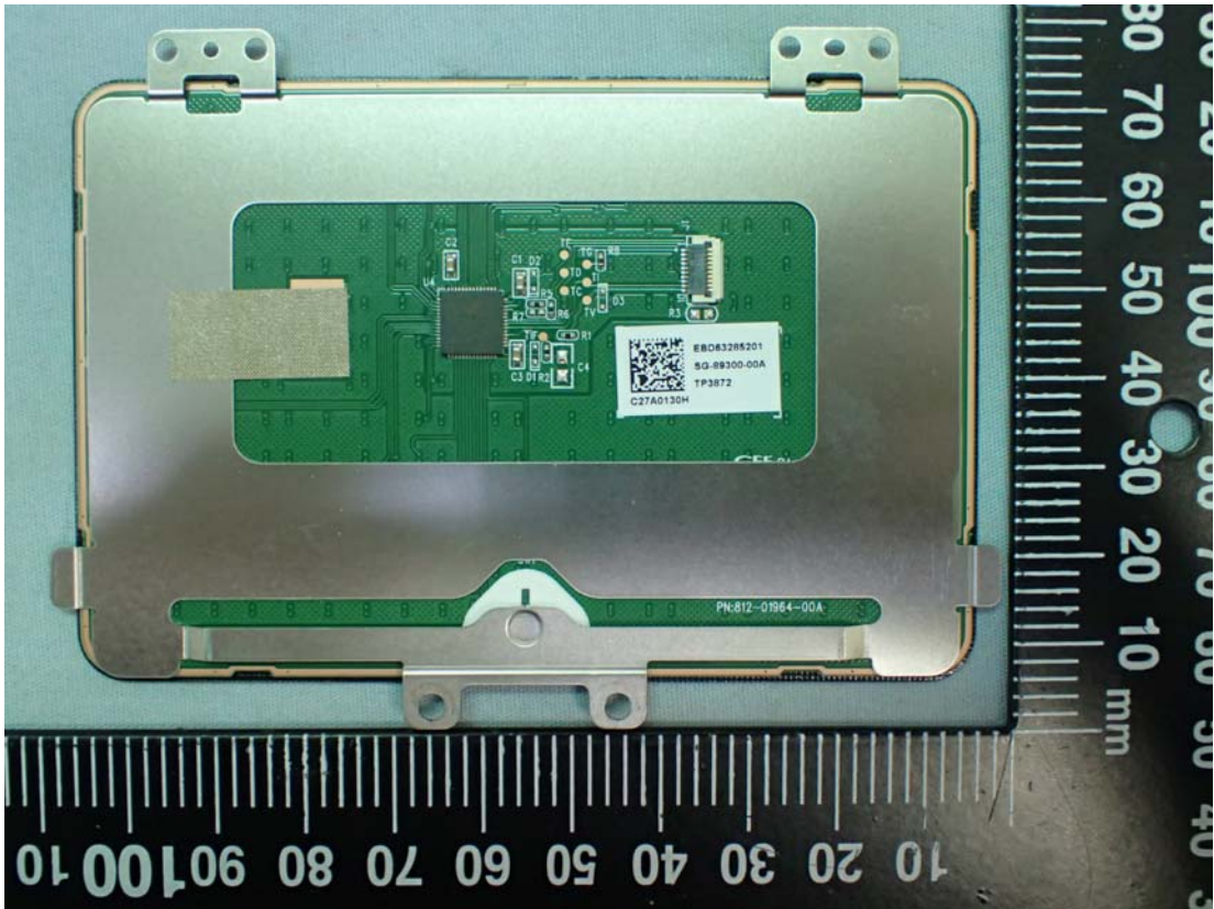
Figure 18 Touch Pad, Back View
