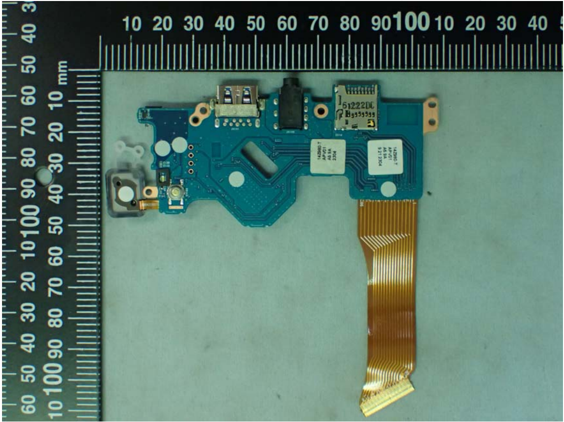
Figure 22 SUB Board (With Finger Printer), Back View
