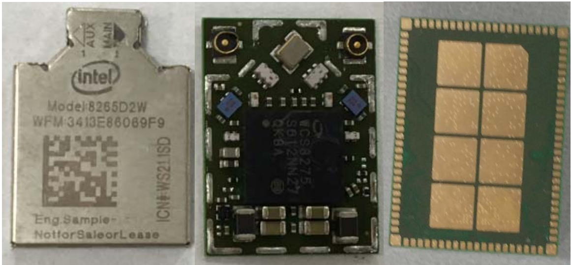
Figure 24 WLAN Combo Card, Remove Cover
