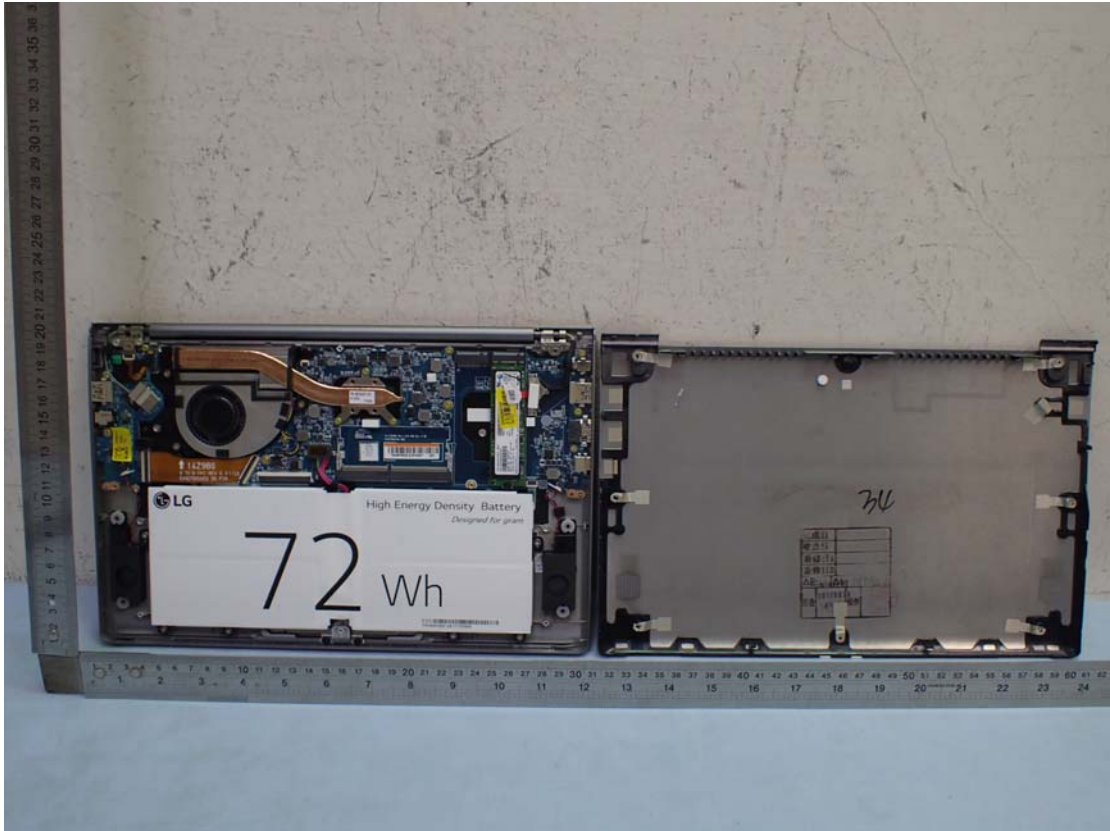
Figure 9 Internal View (Remove Cover View)
