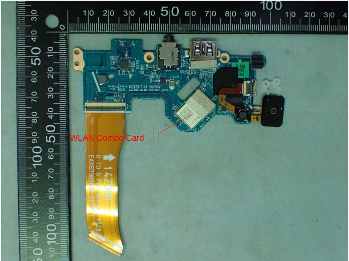
Figure 21 SUB Board (With Finger Printer), Front View
