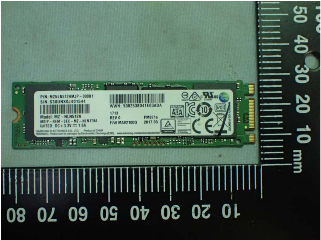
Figure 27 SSD, Front View
