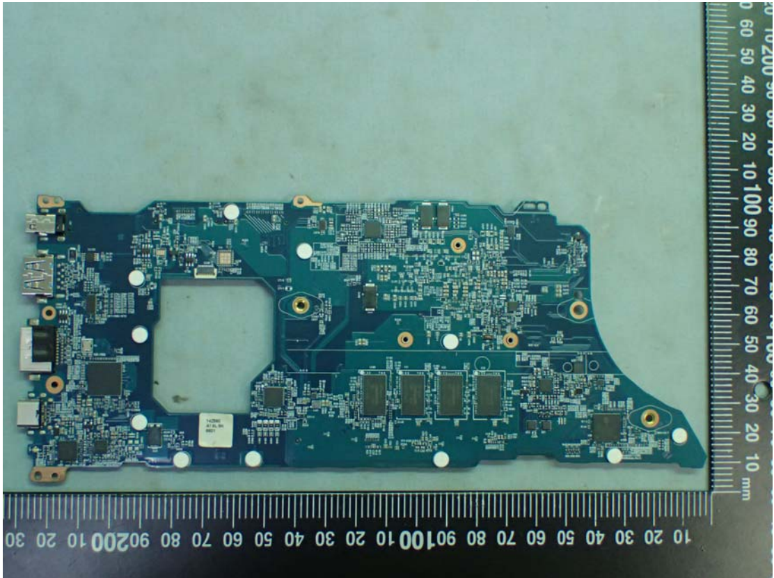
Figure 20 Main Board (with Thunderbolt), Back View
