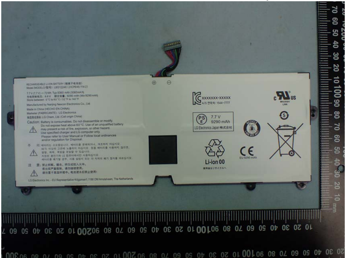
Figure 34 Battery Pack, Back View
