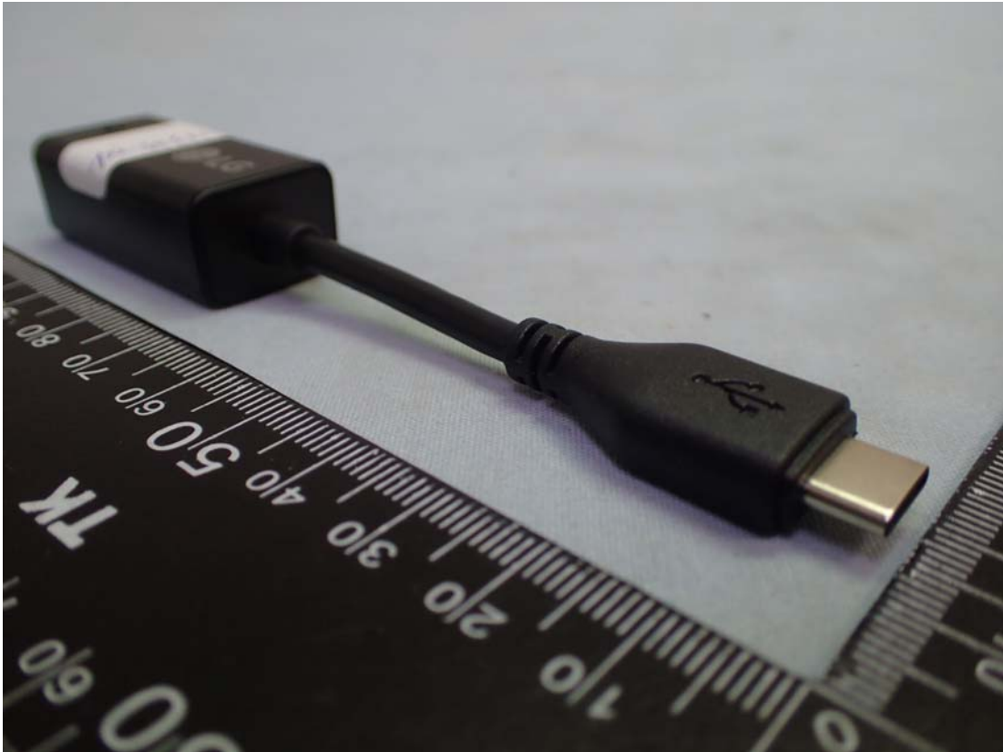
Figure 36 LAN Gender (Black), Back View
