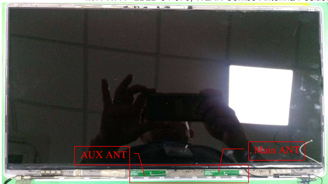
Figure 34 M/N WA-P-LBLB-04-070, WLAN Combo Antenna Position
