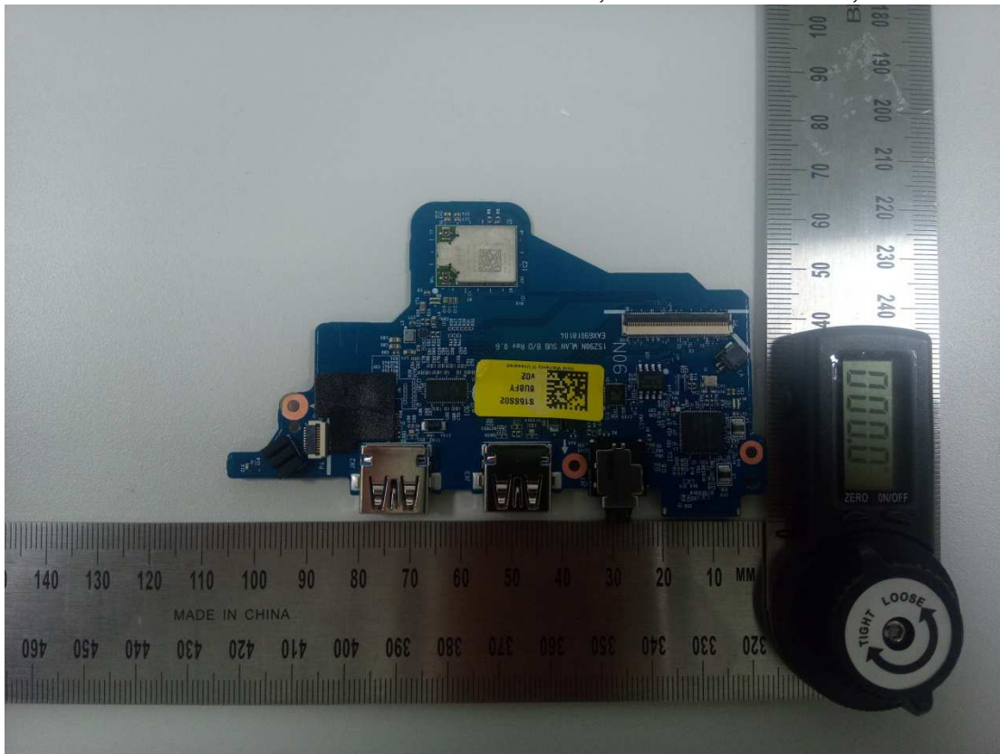
Figure 27 Hannstar, WLAN SUB Board, Front View
