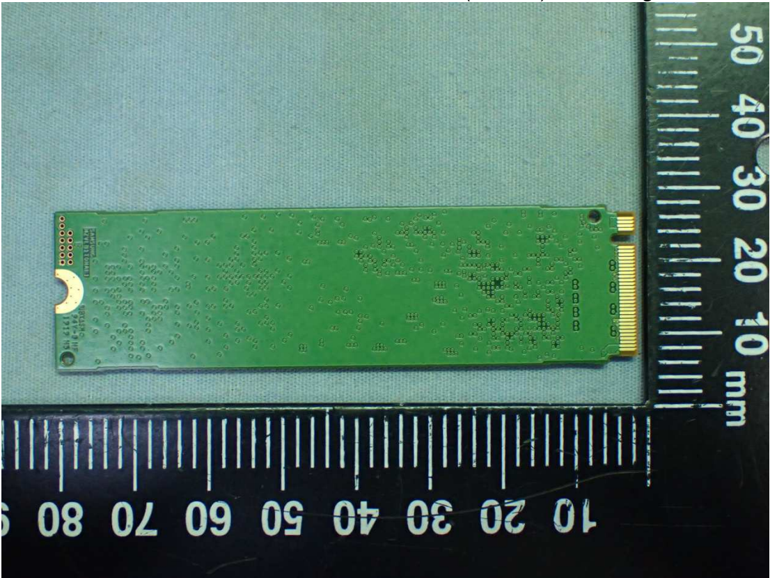
Figure 44 SSD (256GB), Samsung, Back View
