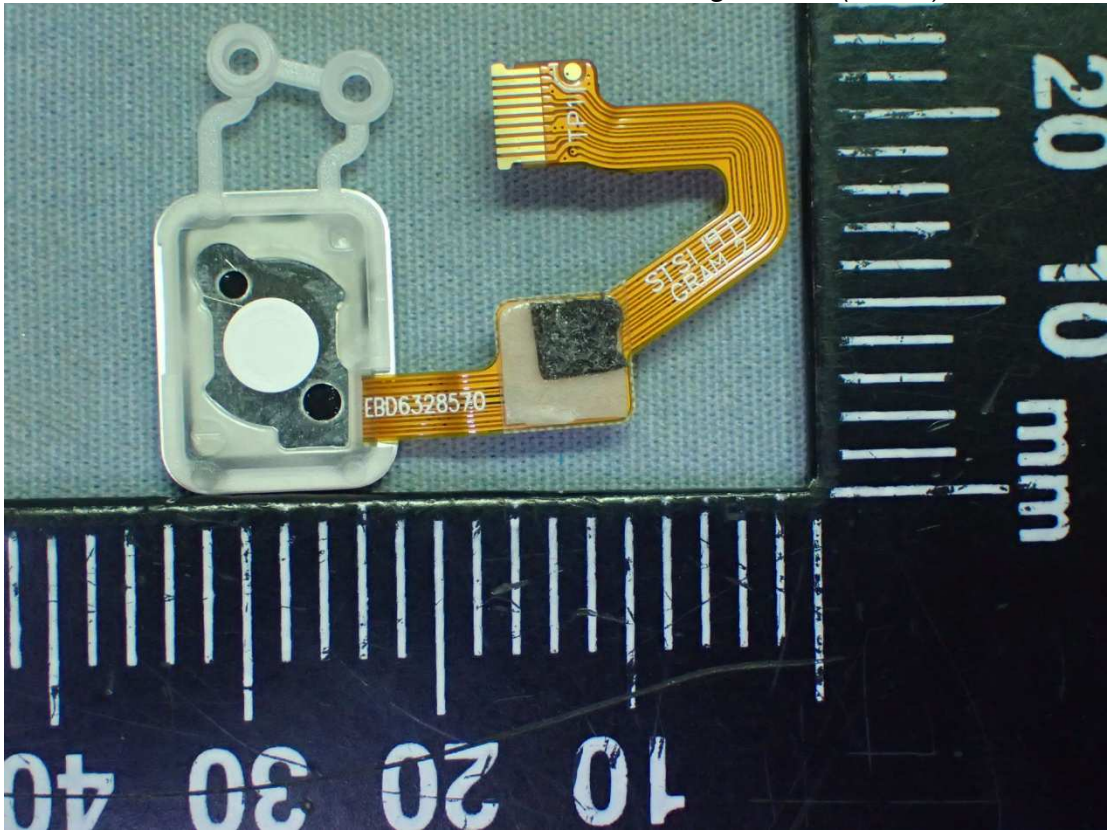
Figure 52 Finger Print (White), Back View
