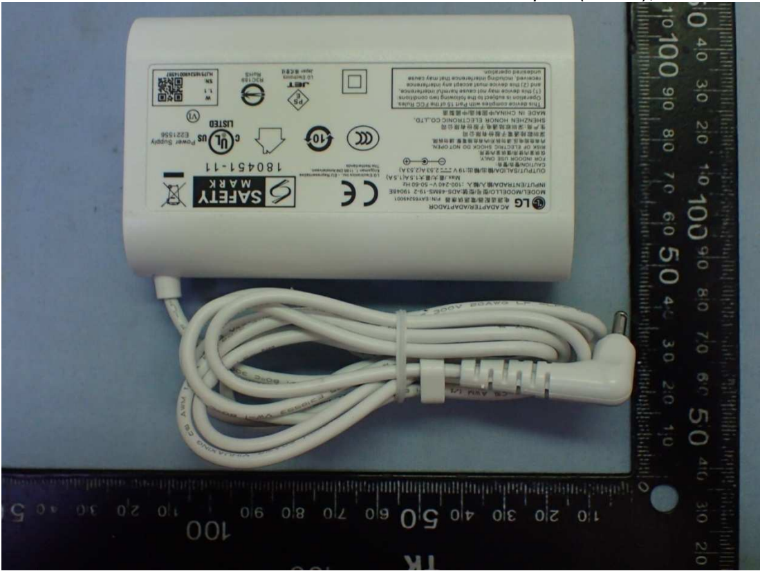
Figure 63 AC Adapter (White), Back View
