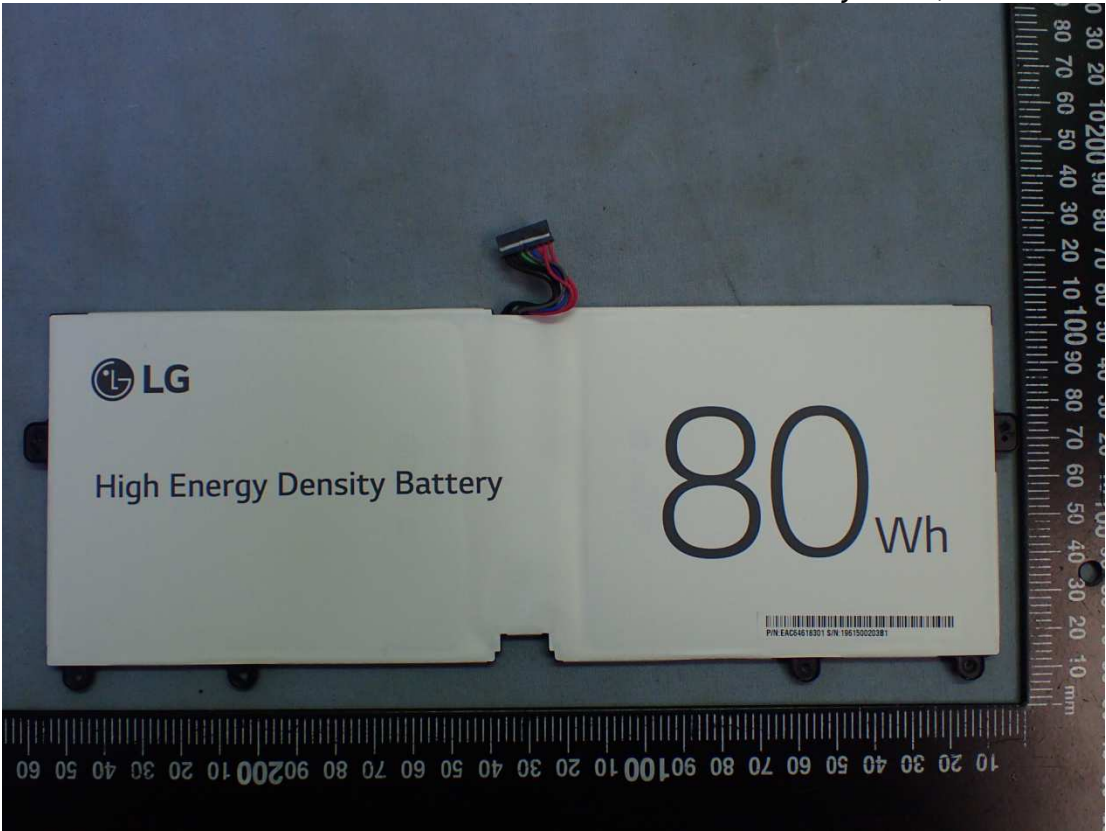
Figure 39 Battery Pack, Front View
