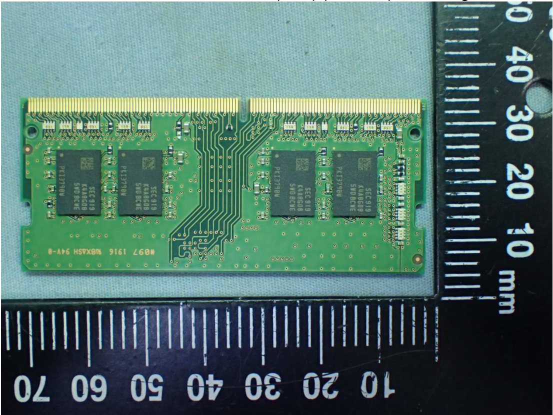
Figure 46 RAM (8GB) (On Card), Samsung, Back View
