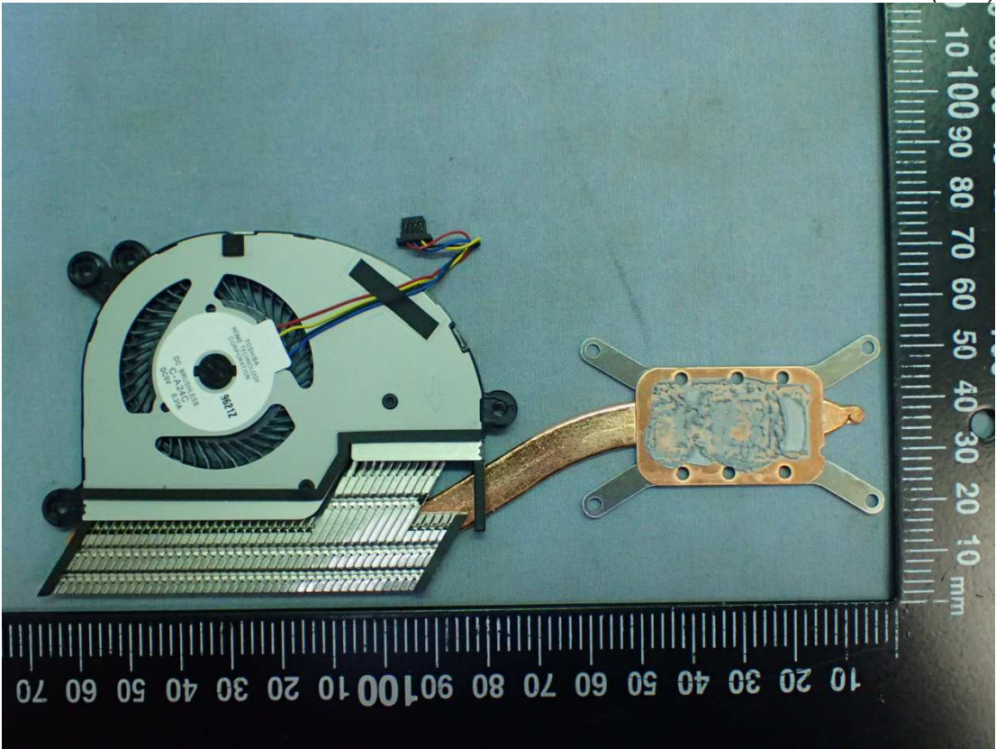
Figure 17 Internal View (Fan)
