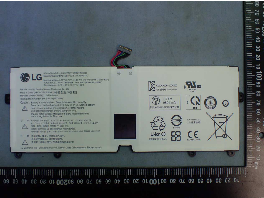
Figure 40 Battery Pack, Back View
