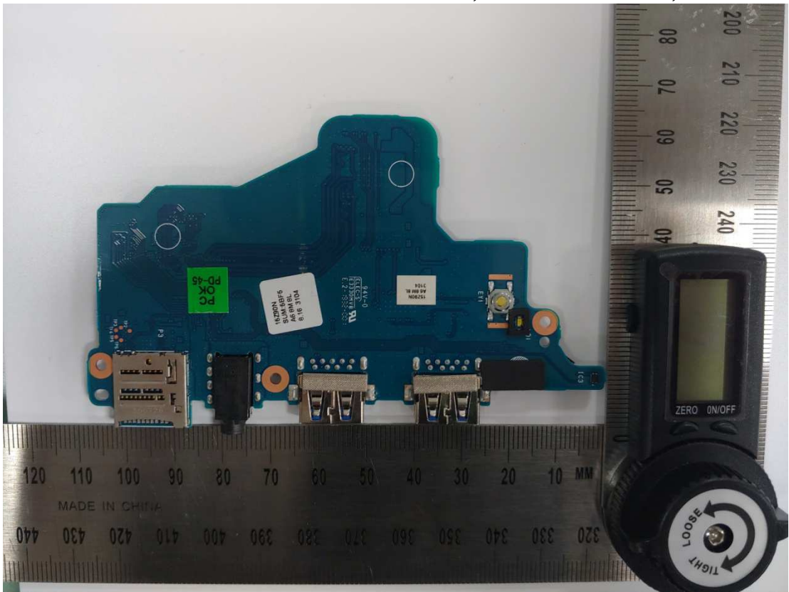
Figure 30 Elec & Eltek, WLAN SUB Board, Back View
