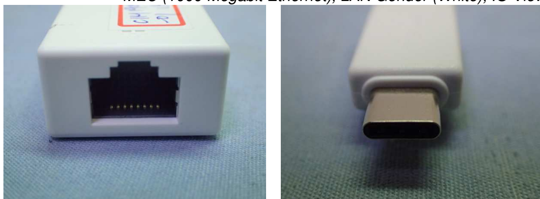
Figure 54 MEC (1000 Megabit Ethernet), LAN Gender (White), IO View
