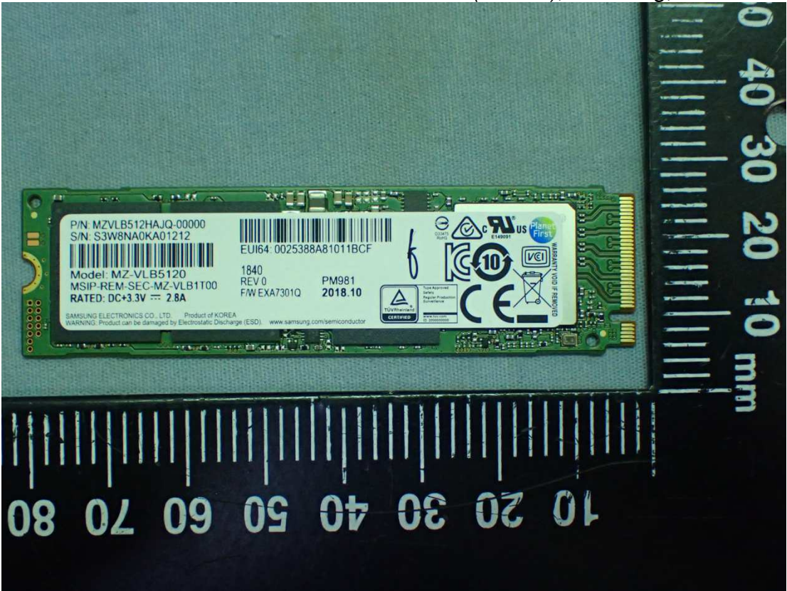
Figure 41 SSD (512GB), Samsung, Front View
