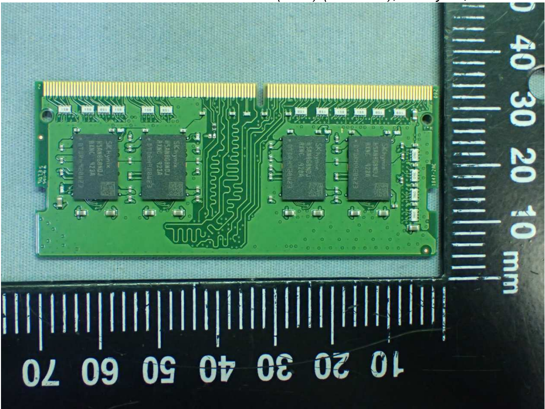
Figure 48 RAM (8GB) (On Card), SK hynix, Back View
