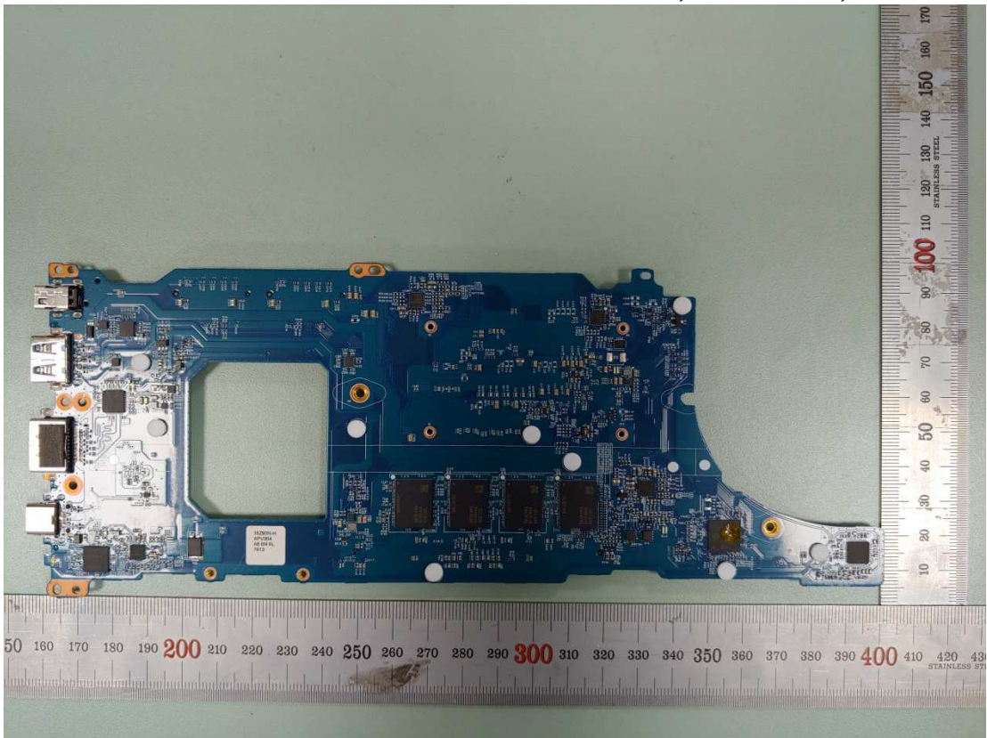
Figure 26 Elec & Eltek, Main Board, Back View
