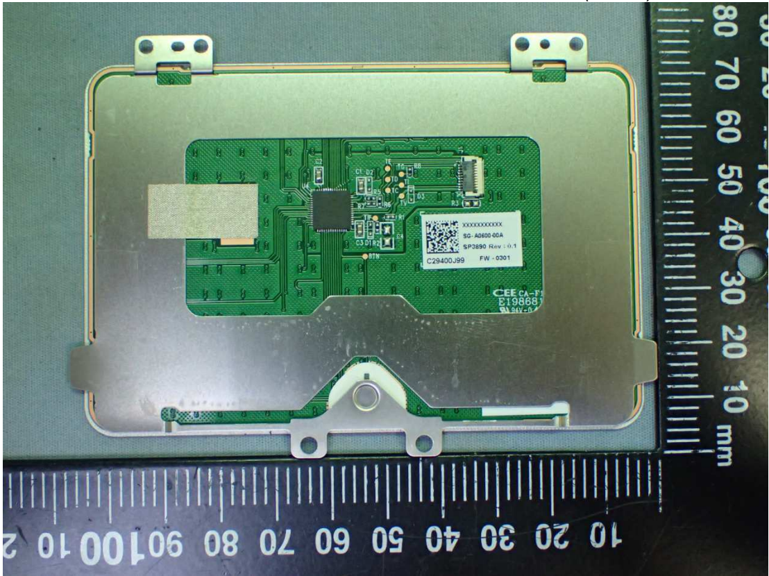
Figure 50 Touch Pad (White), Back View
