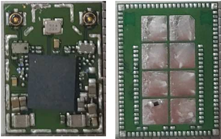
Figure 32 WLAN Combo Card, Remove Cover
