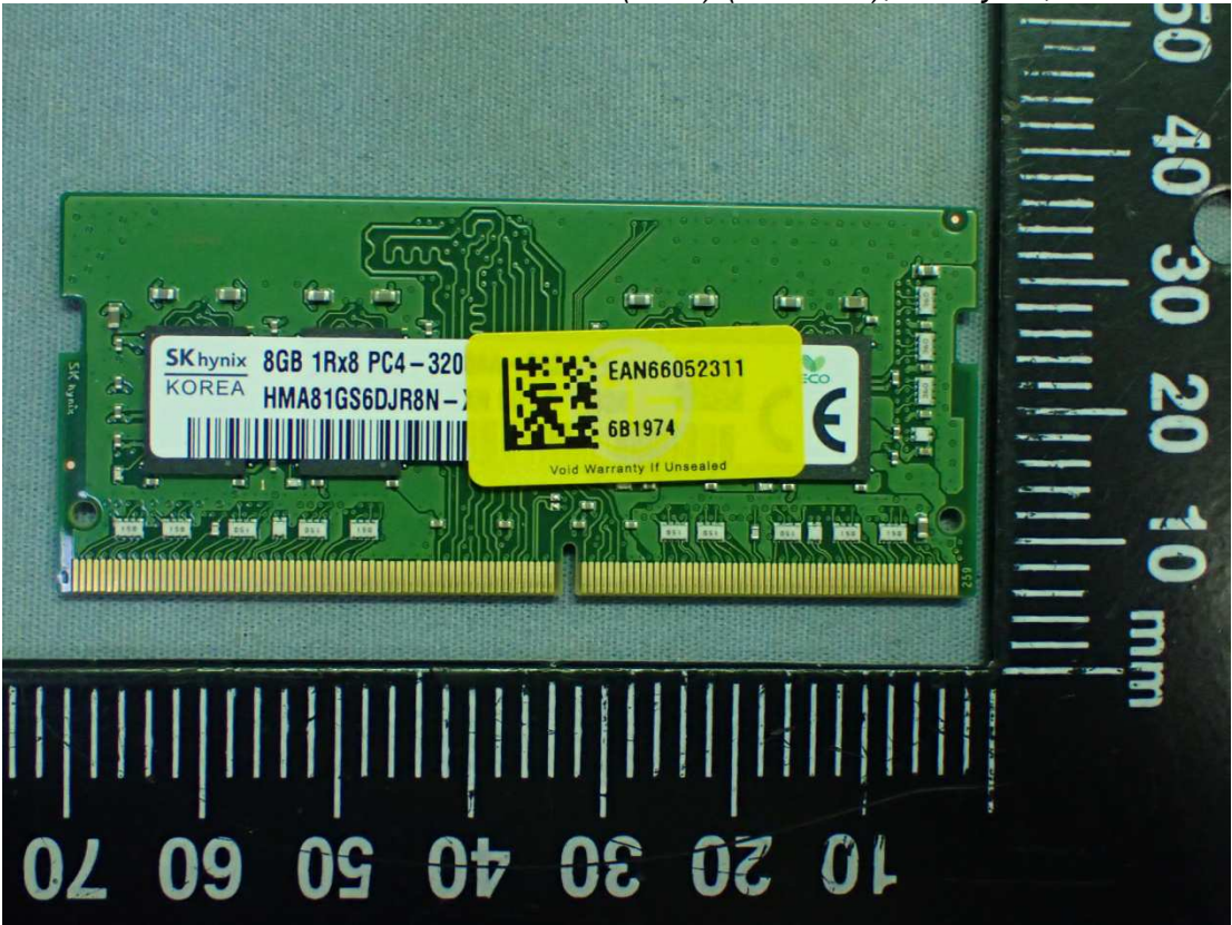
Figure 47 RAM (8GB) (On Card), SK hynix, Front View
