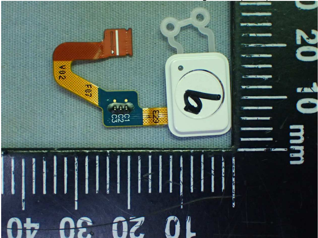
Figure 51 Finger Print (White), Front View
