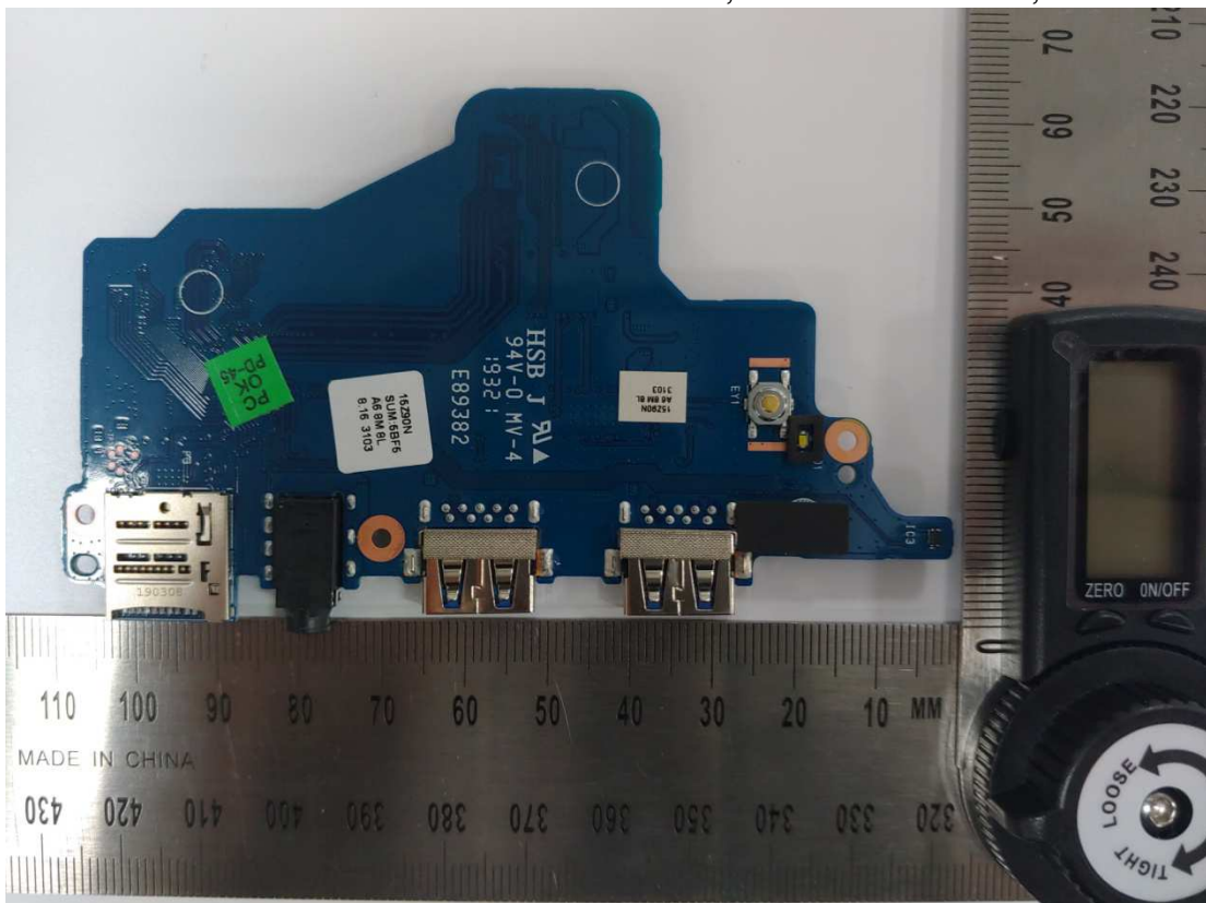
Figure 28 Hannstar, WLAN SUB Board, Back View
