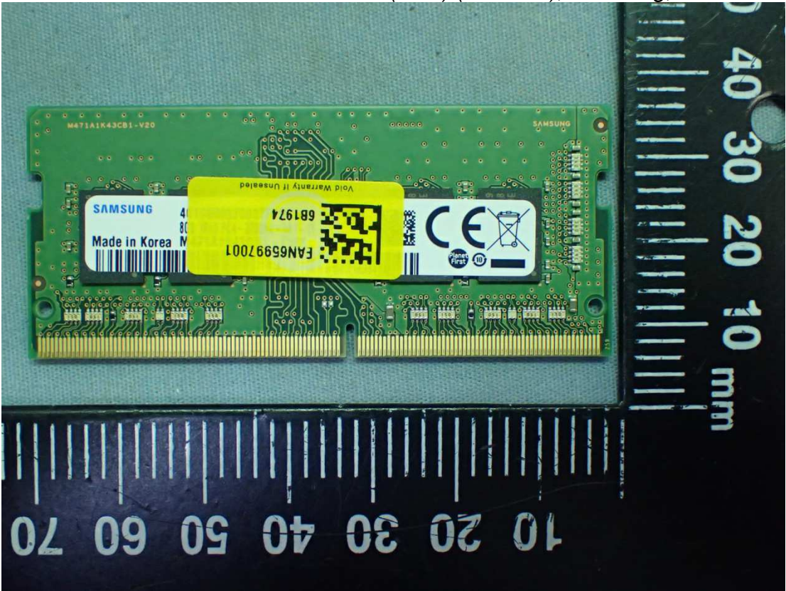
Figure 45 RAM (8GB) (On Card), Samsung, Front View
