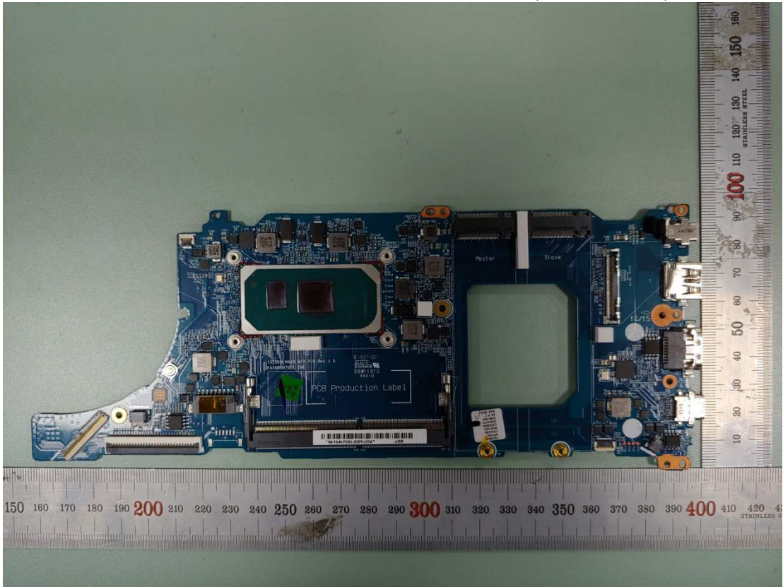
Figure 25 Elec & Eltek, Main Board, Front View
