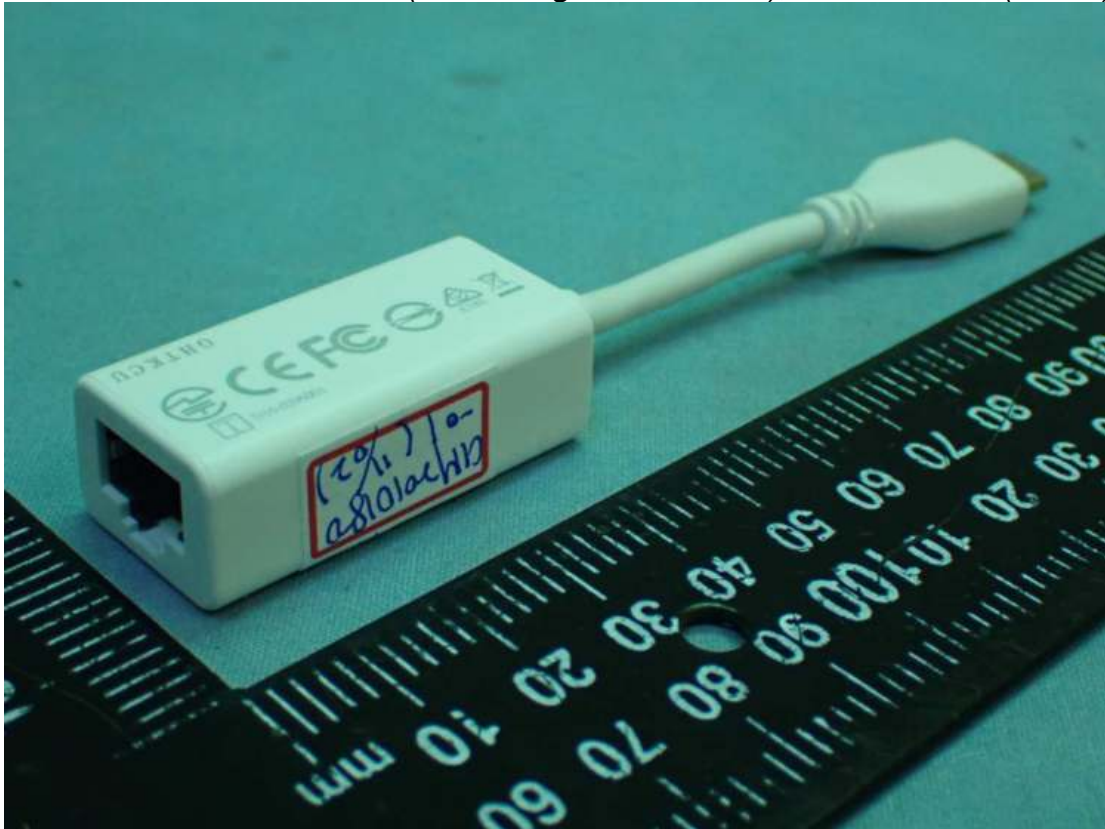
Figure 59 MEC (1000 Megabit Ethernet), LAN Gender (White)
