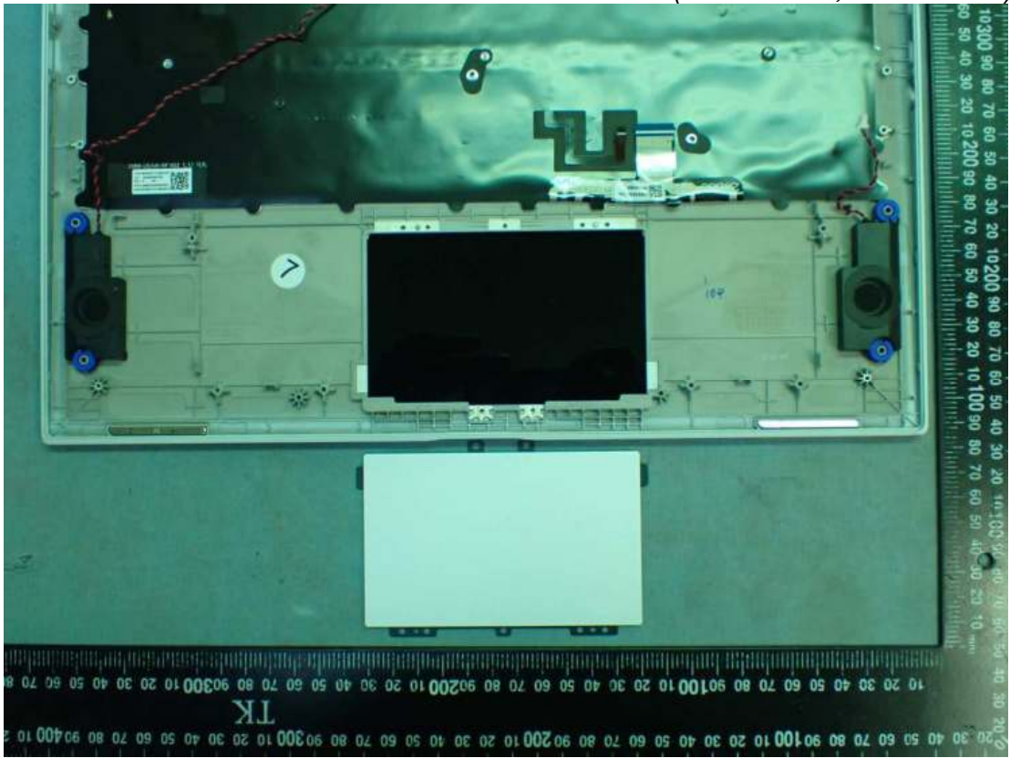
Figure 20 Internal View (Touch Pad, Front View)
