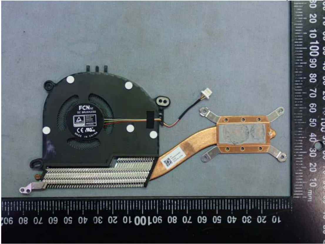
Figure 18 Internal View (DC Fan)
