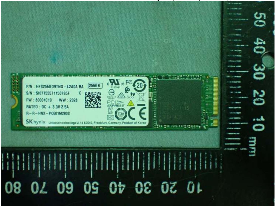
Figure 49 SK hynix, SSD (256GB), Front View
