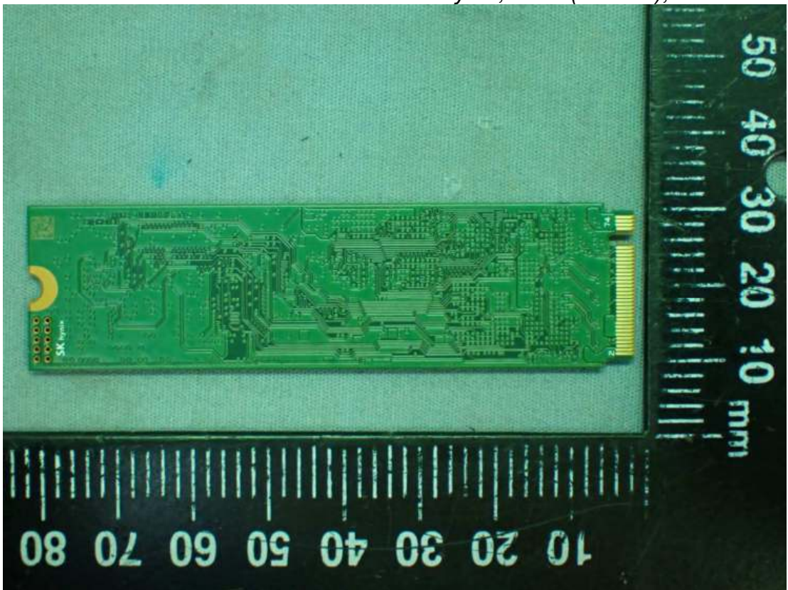
Figure 50 SK hynix, SSD (256GB), Back View
