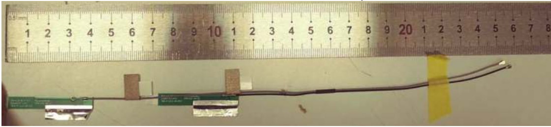
Figure 35 M/N WA-P-LELE-04-002, WLAN Combo Antenna
