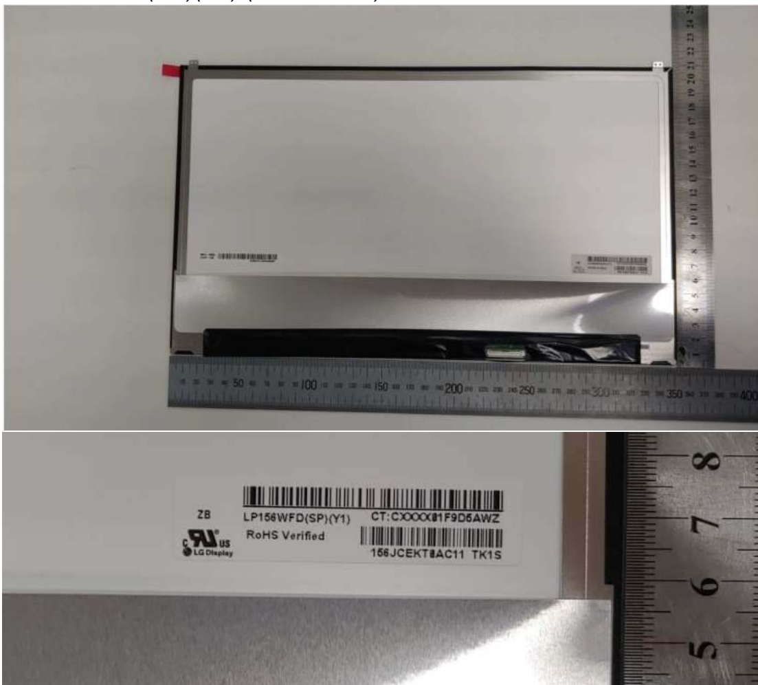
Figure 32 M/N: LP156WFD(SP)(Y1) (With Touch), LCD Panel, Back View/ Label View
