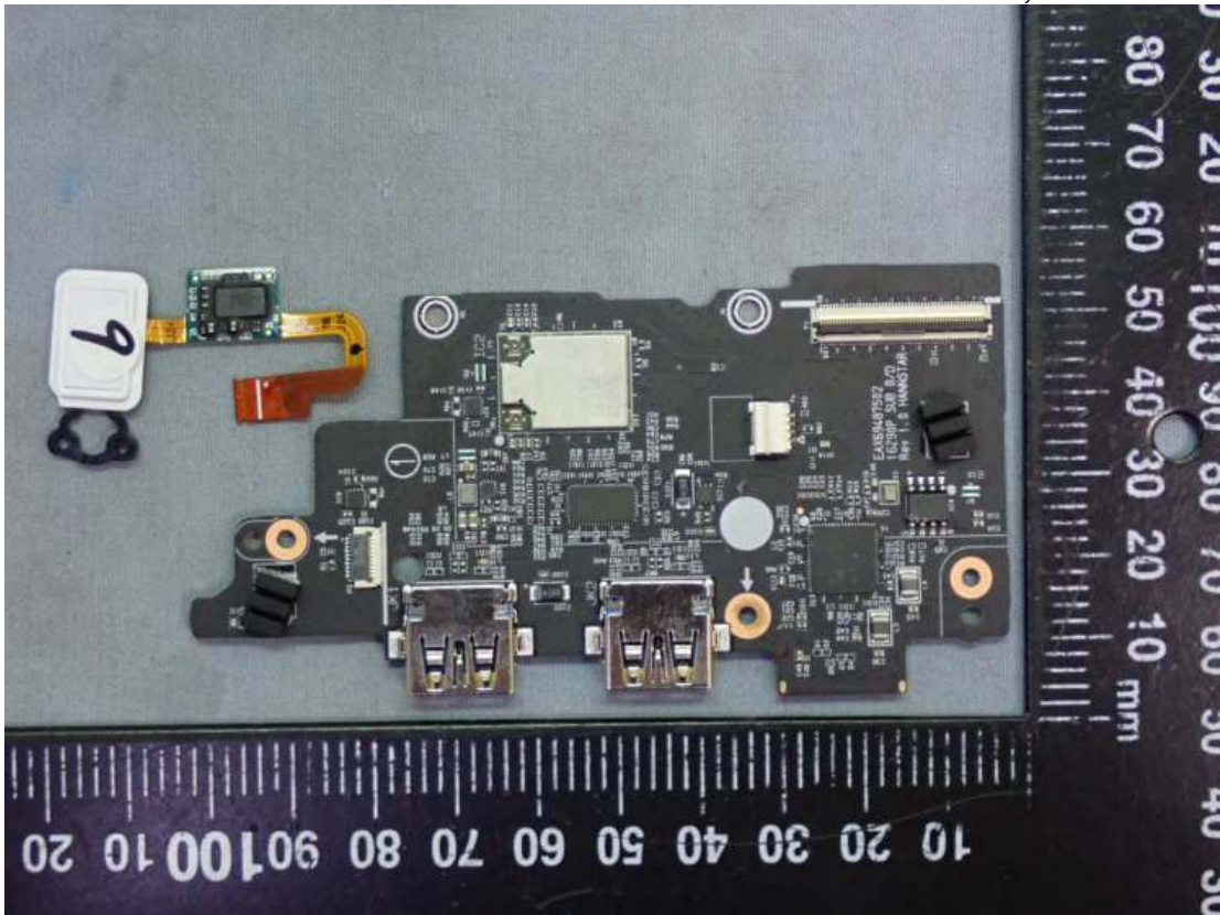
Figure 27 WLAN SUB Board, Front View
