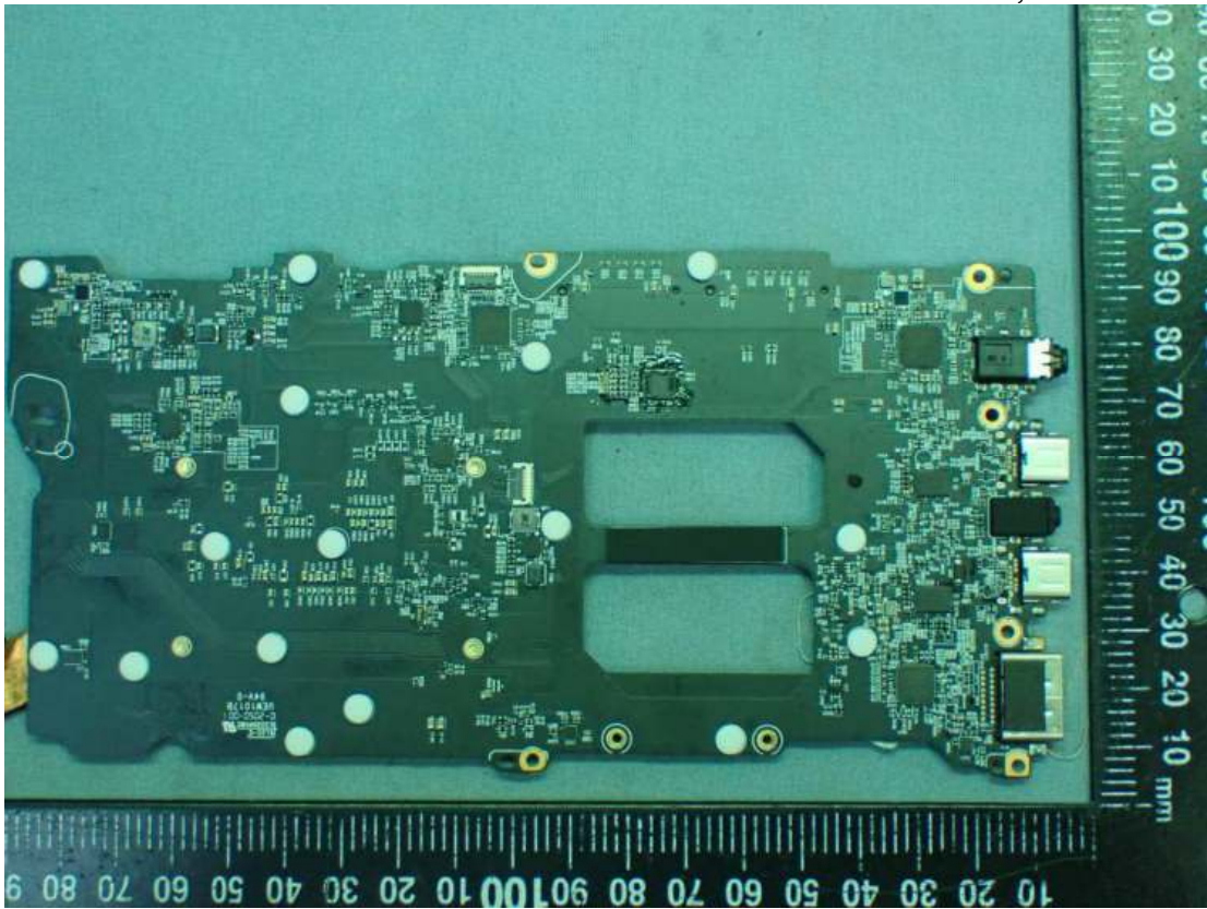
Figure 25 Main Board with TPM IC, Back View
