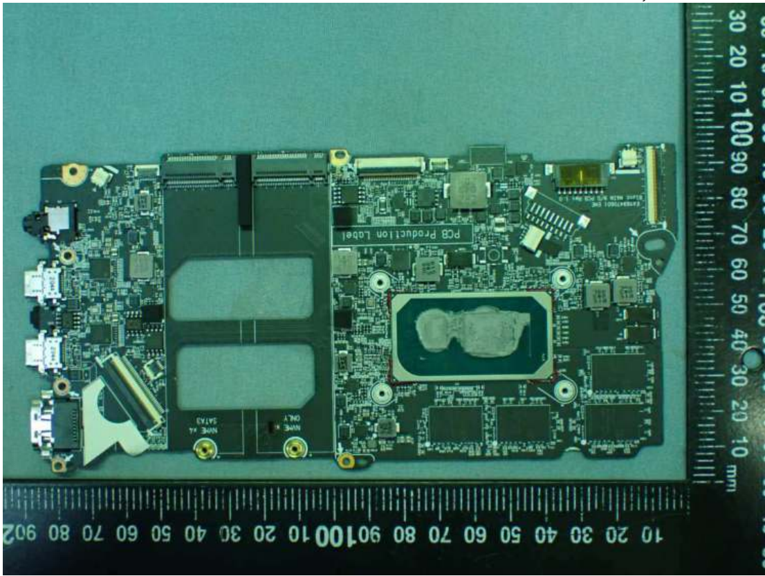
Figure 24 Main Board with TPM IC, Front View
