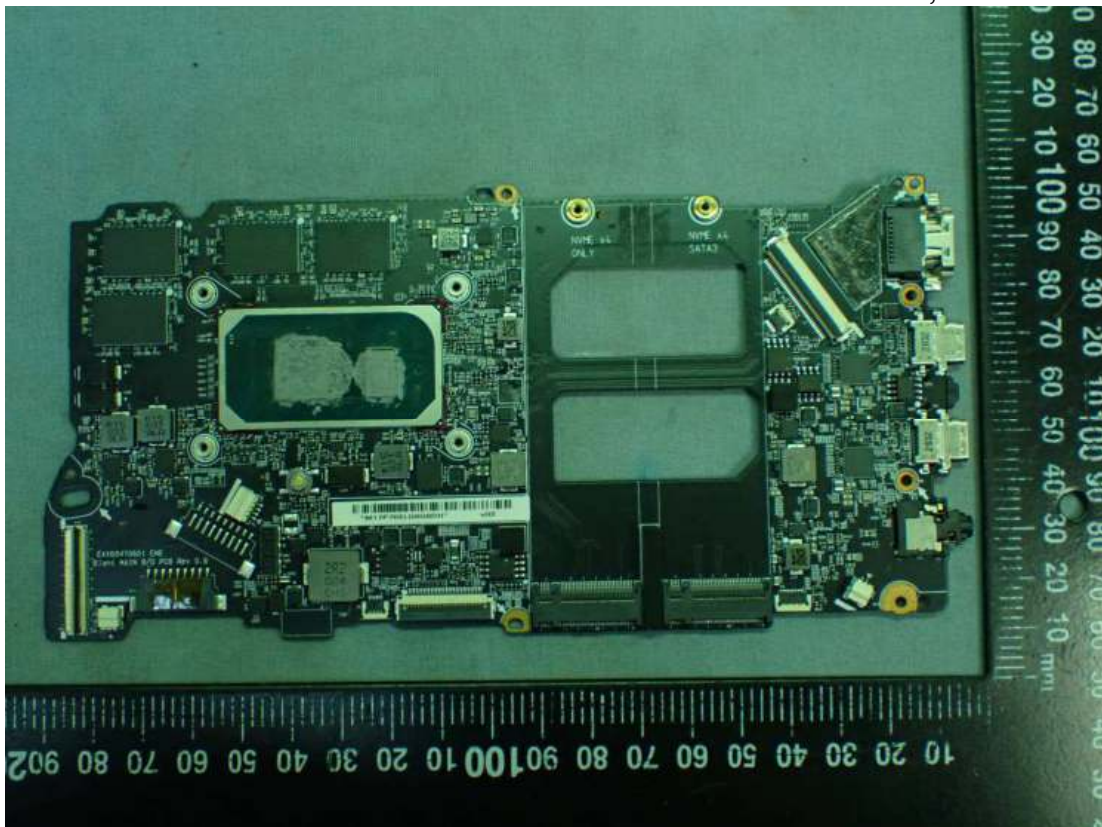
Figure 22 Main Board without TPM IC, Front View
