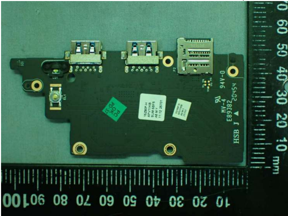
Figure 28 WLAN SUB Board, Back View
