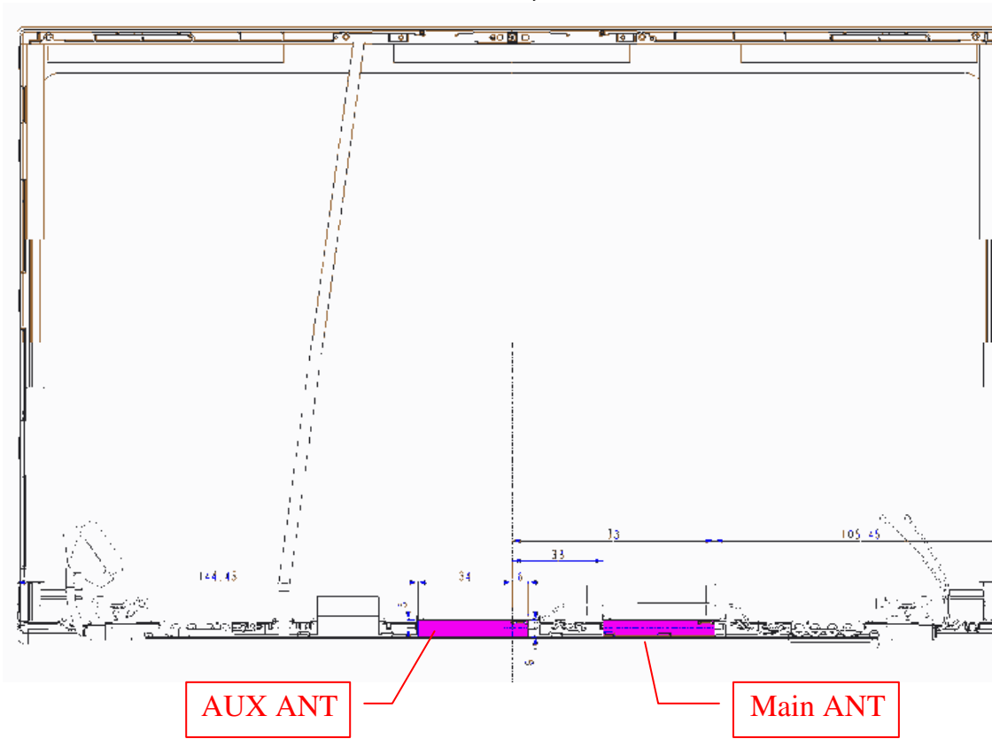
Figure 36 M/N WA-P-LELE-04-002, WLAN Combo Antenna Position
