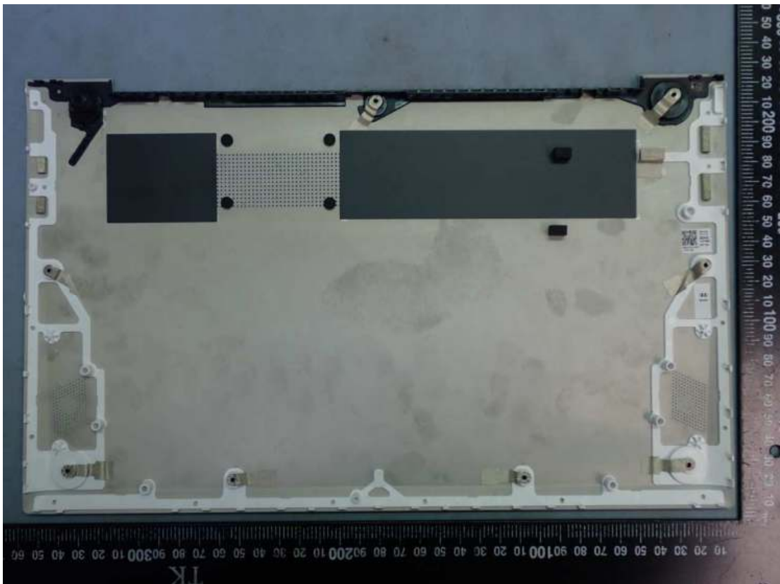
Figure 16 Internal View
