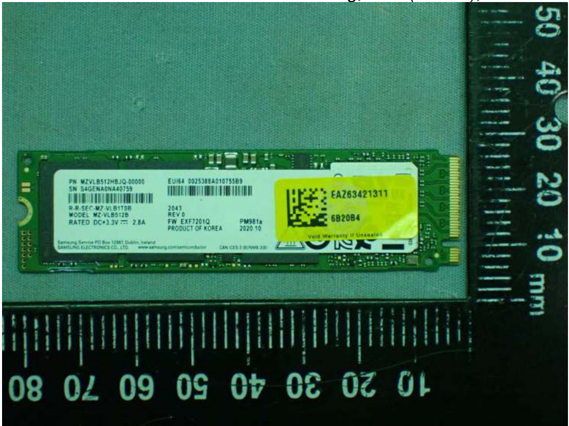
Figure 41 Samsung, SSD (512GB), Front View
