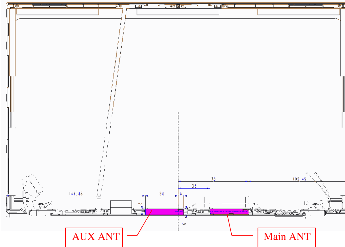
Figure 38 M/N L1LRF004-CS-H, WLAN Combo Antenna Position
