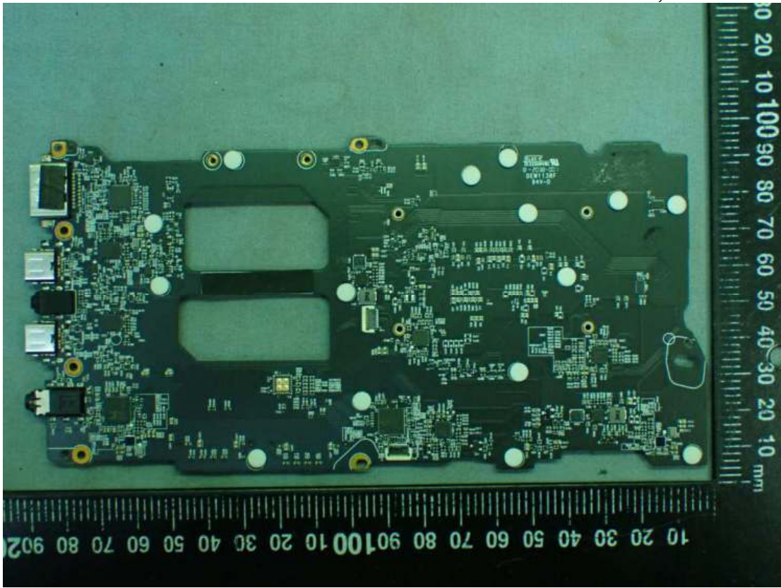
Figure 23 Main Board without TPM IC, Back View
