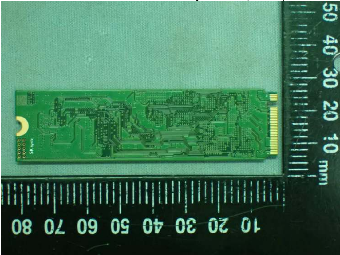
Figure 44 SK hynix, SSD (512GB), Back View
