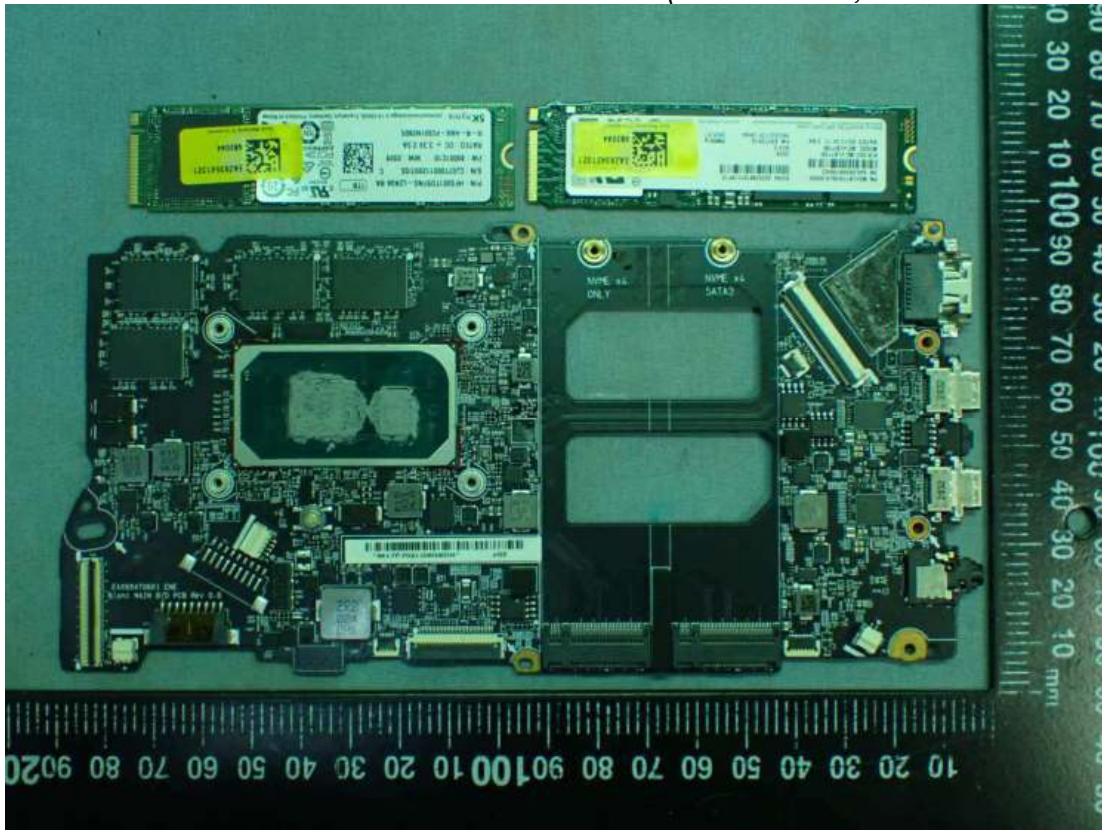
Figure 21 Internal View (Main Board, Removed SSD)
