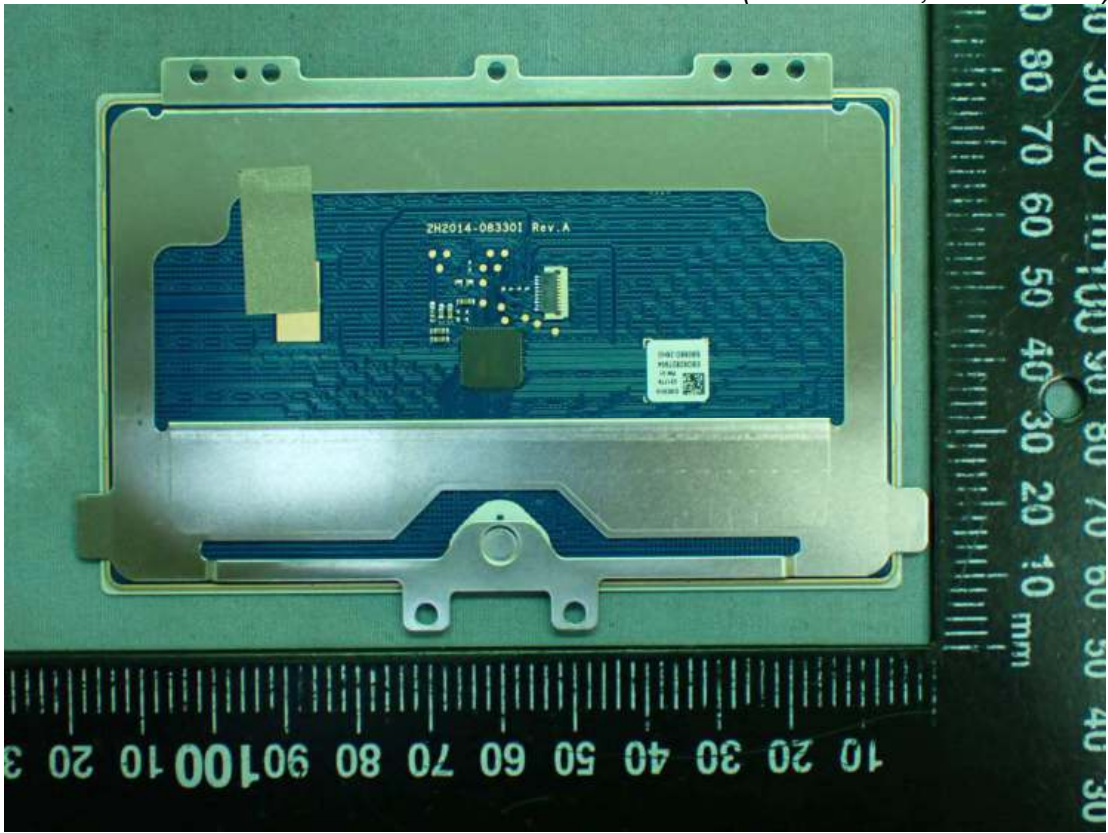
Figure 19 Internal View (Touch Pad, Back View)
