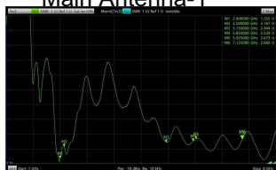
Main Antenna-1
