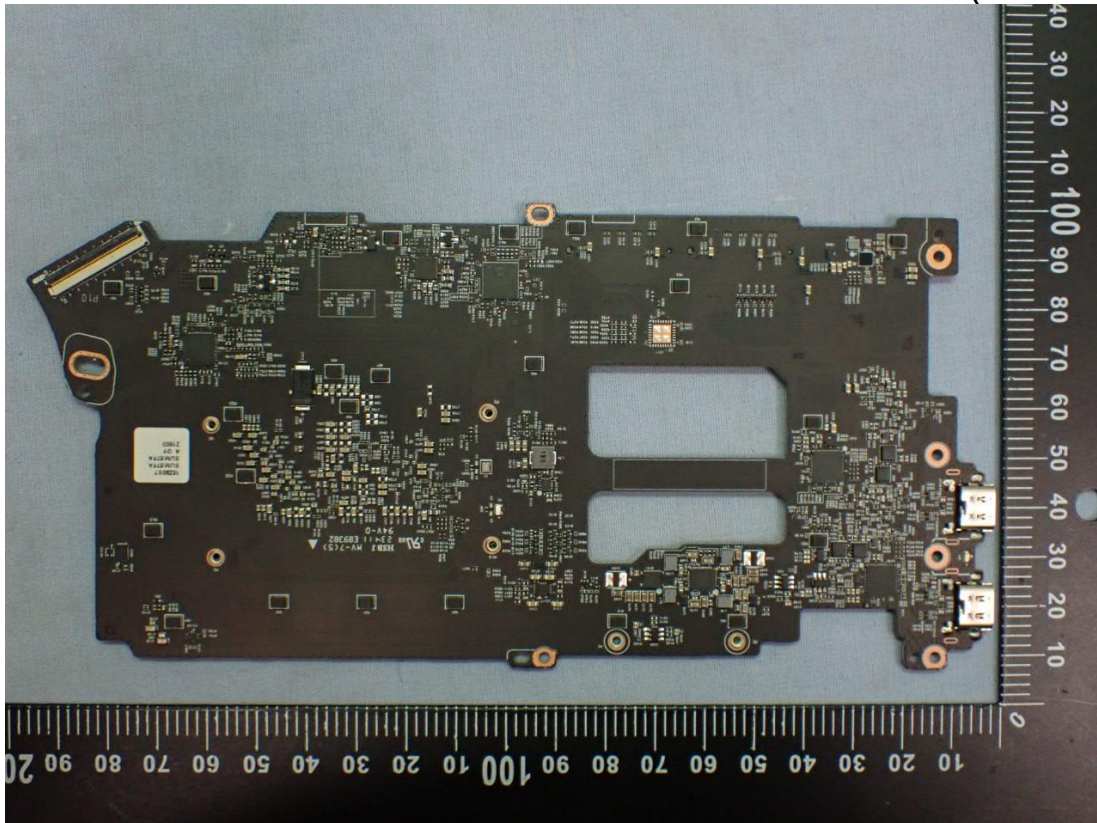
Figure 18 15Z90ST MAIN B/D PCB Main Board (Back View)
