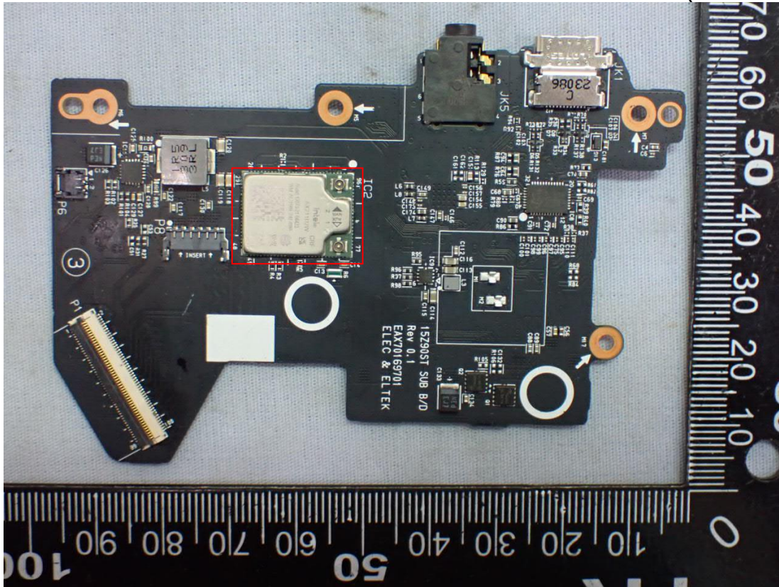
Figure 13 15Z90ST SUB B/D WLAN SUB Board (Front View)
