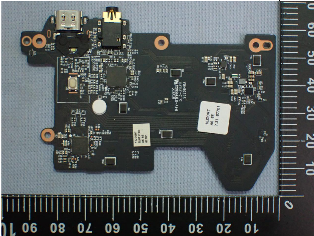
Figure 14 15Z90ST SUB B/D WLAN SUB Board (Back View)
