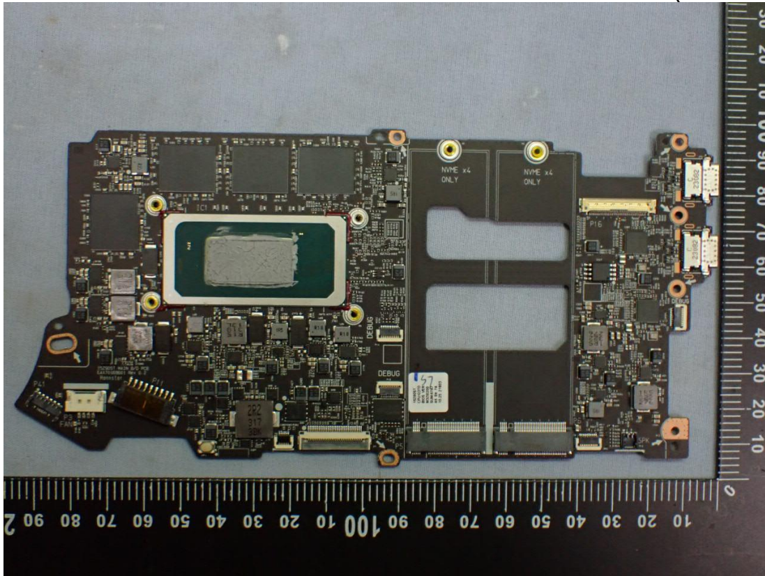
Figure 17 15Z90ST MAIN B/D PCB Main Board (Front View)
