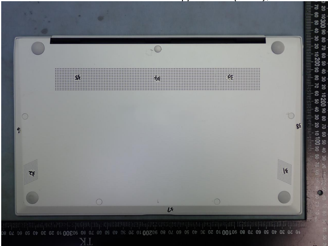
Figure 10 General Appearance (White), Bottom View
