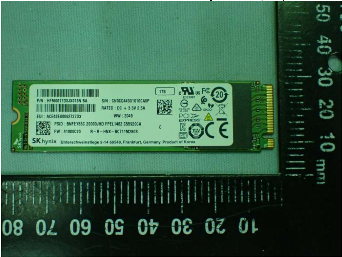
Figure 41 SK hynix, SSD (1TB), Front View
