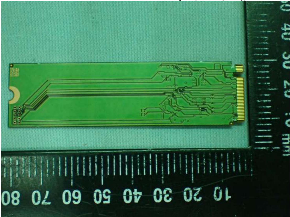
Figure 42 SK hynix, SSD (1TB), Back View
