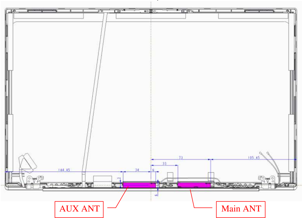
Figure 32 M/N WA-P-LELE-04-002, WLAN Combo Antenna Position
