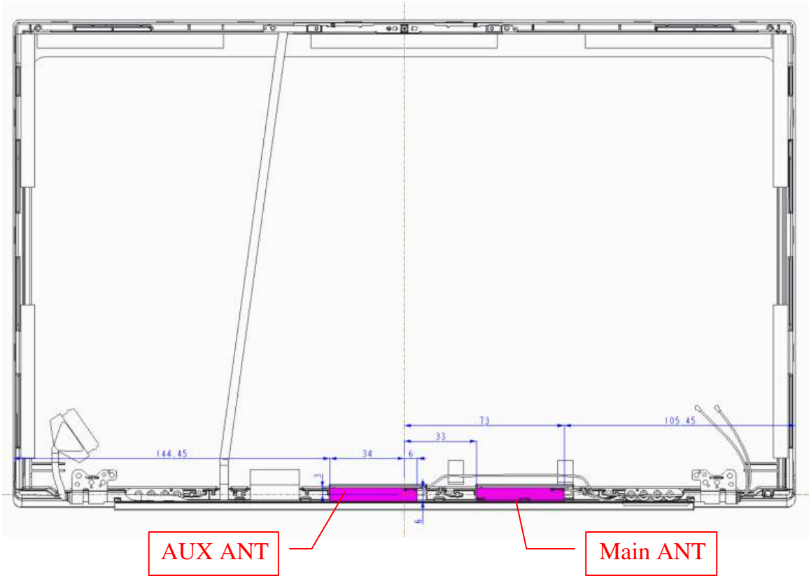
Figure 34 M/N L1LRF004-CS-H, WLAN Combo Antenna Position
