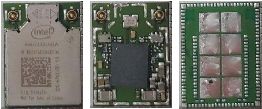
Figure 26 WLAN Combo Card, Remove Cover
