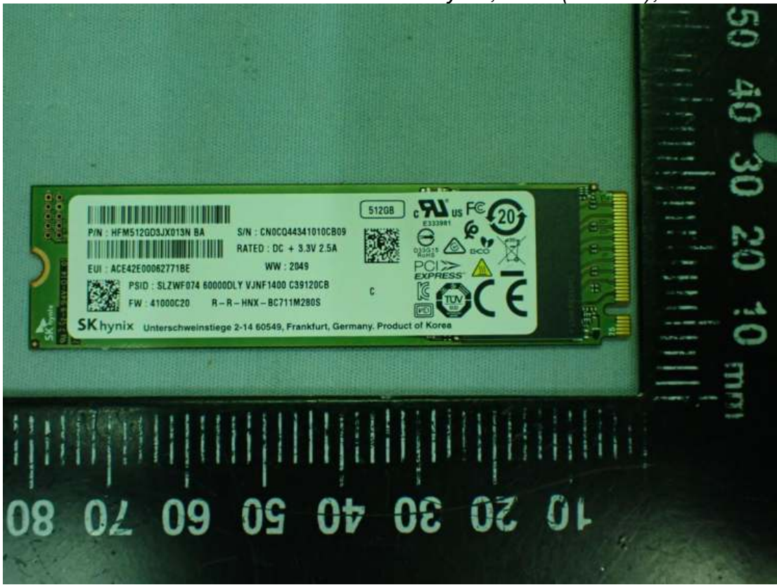
Figure 39 SK hynix, SSD (512GB), Front View
