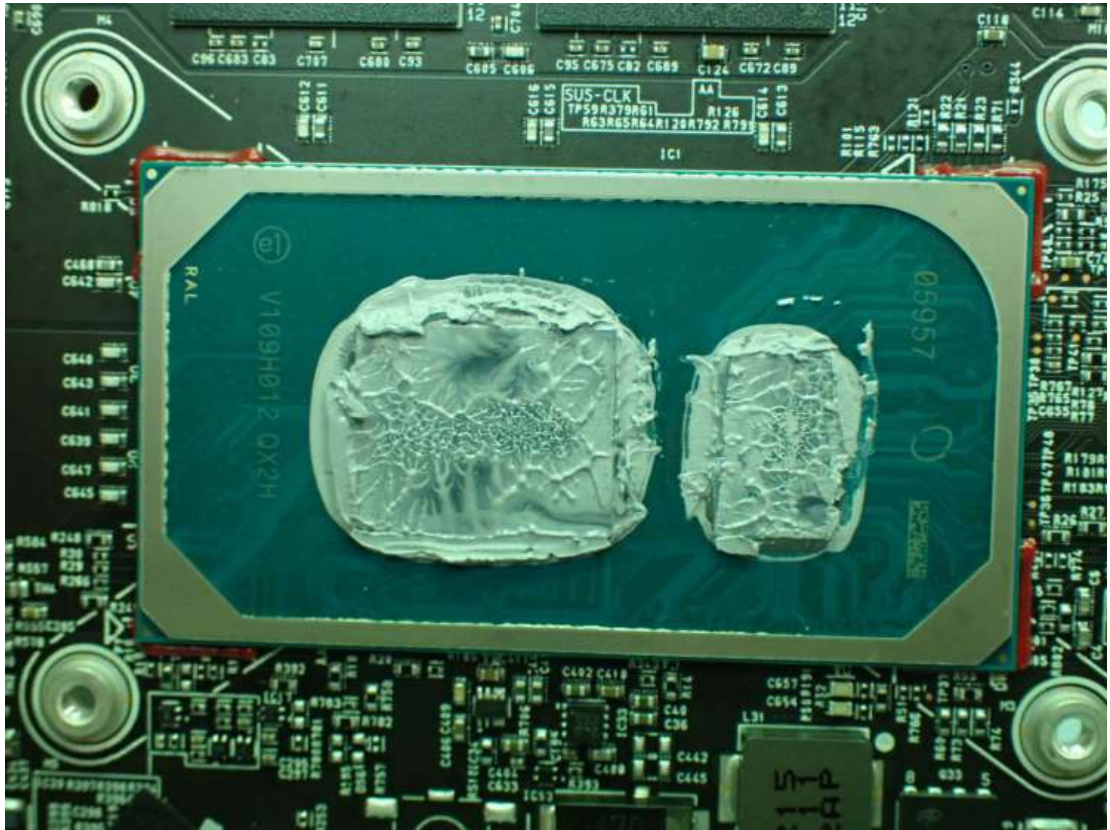
Figure 22 CPU View
