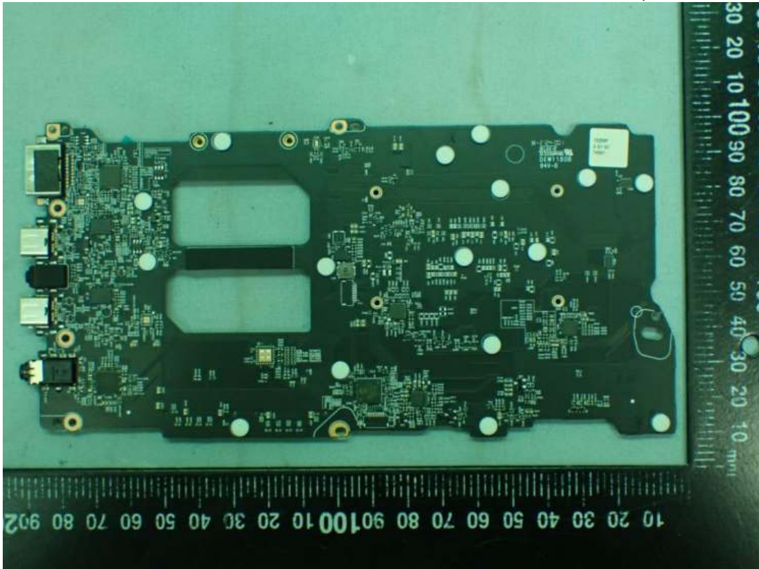
Figure 19 1xZ90P MAIN B/D PCB Main Board, Back View
