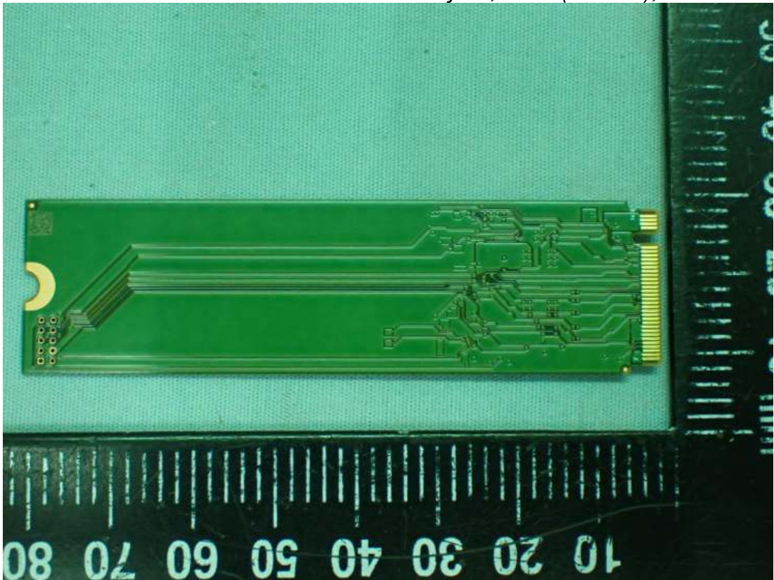
Figure 38 SK hynix, SSD (256GB), Back View
