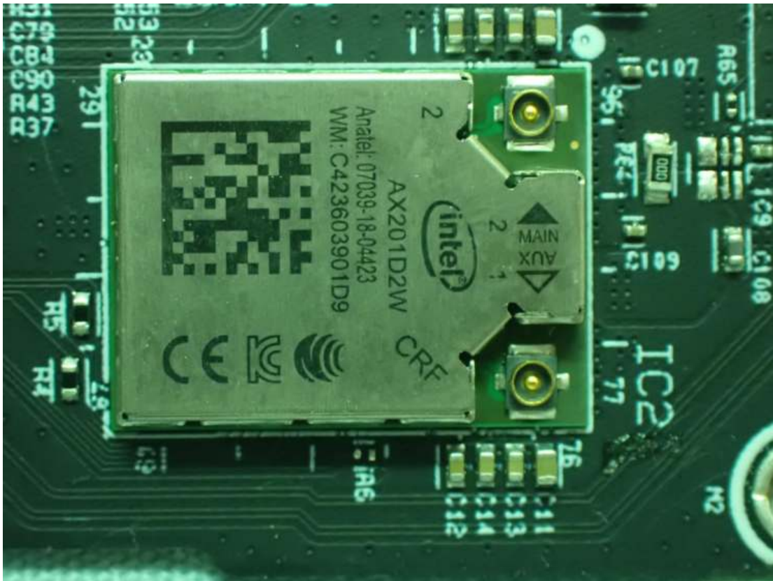
Figure 25 WLAN Combo Card View
