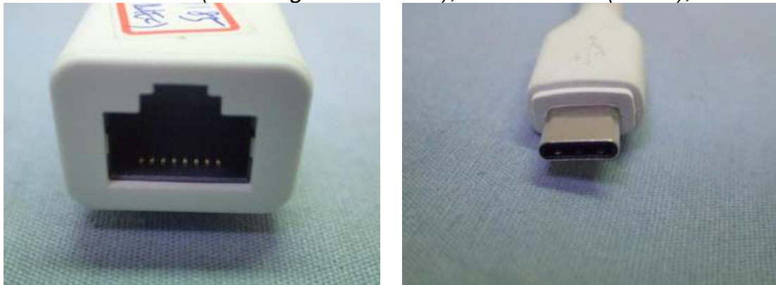
Figure 44 SUZHOU MEC (100 Megabit Ethernet), LAN Gender (White), IO View
