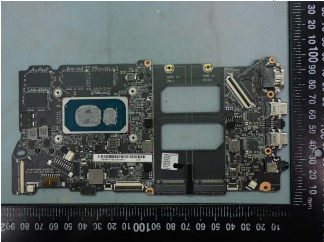
Figure 20 Blanc MAIN B/D PCB Main Board, Front View
