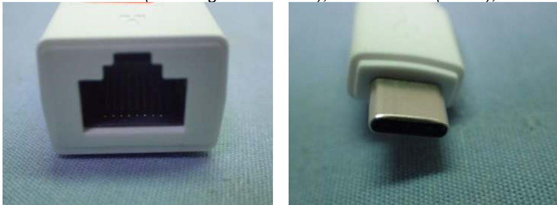
Figure 46 ARIN (100 Megabit Ethernet), LAN Gender (White), IO View
