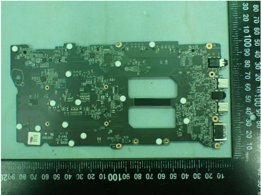
Figure 21 Blanc MAIN B/D PCB Main Board, Back View
