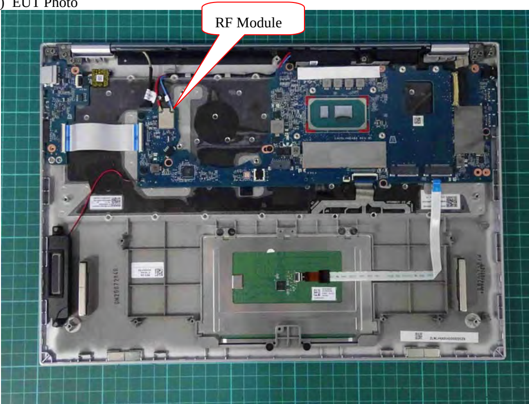
(38) EUT Photo
