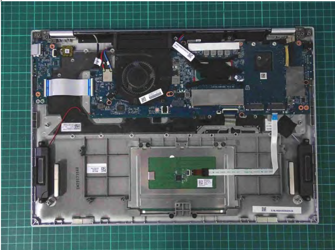
(26) EUT Photo
