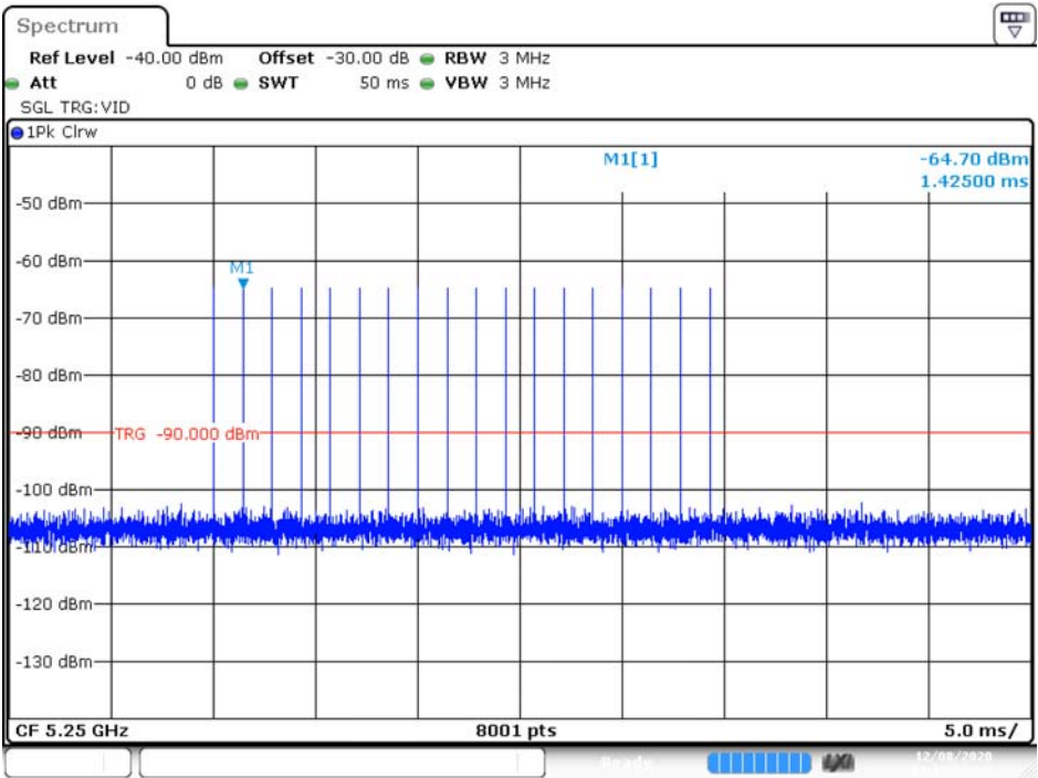
Mode 1: Transmit - 802.11ax-160MHz Radar Type 0 Calibration Plot (5250MHz)
