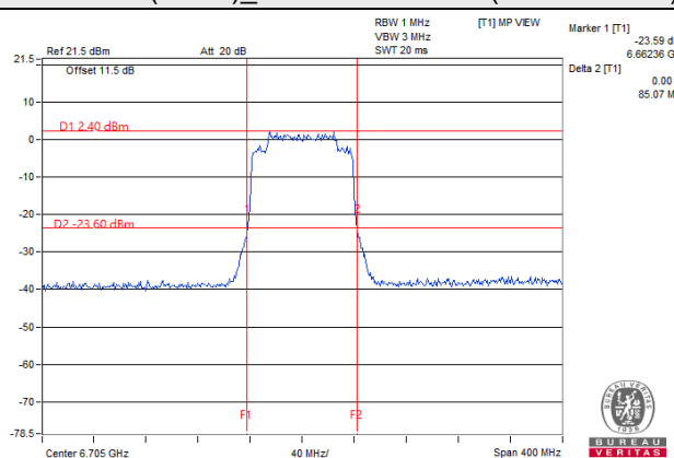
802.11ax (HE80)_Chain 0 / CH 151 (U-NII-7 Band)
