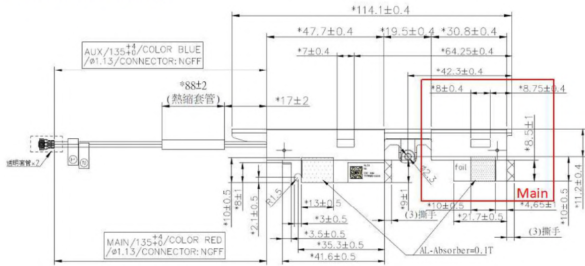
Main Antenna Drawing:
