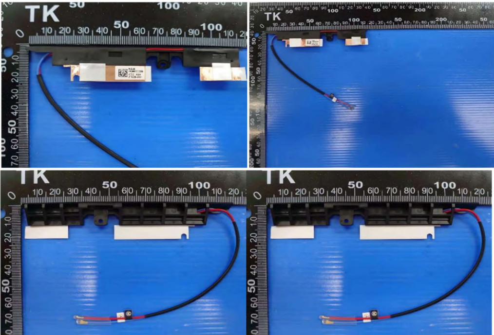
Main Antenna Photo (Front/Back):
