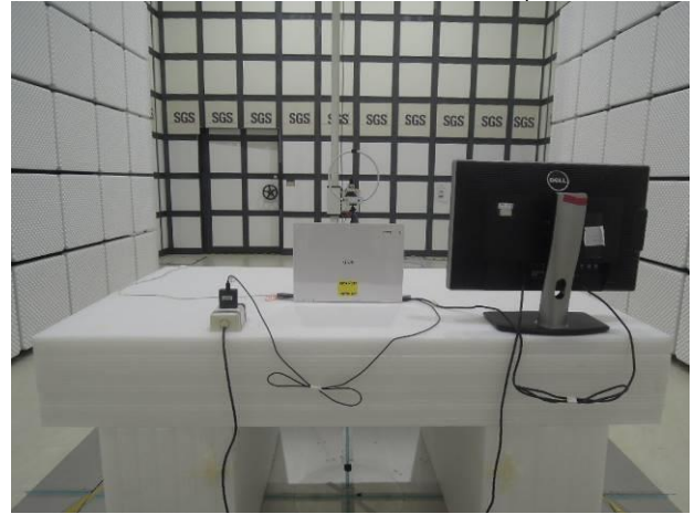
FCC 15_407 WLAN Radiated Setup
