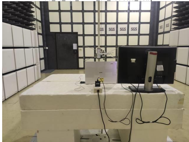
FCC 15_407 WLAN 6E Radiated Setup
