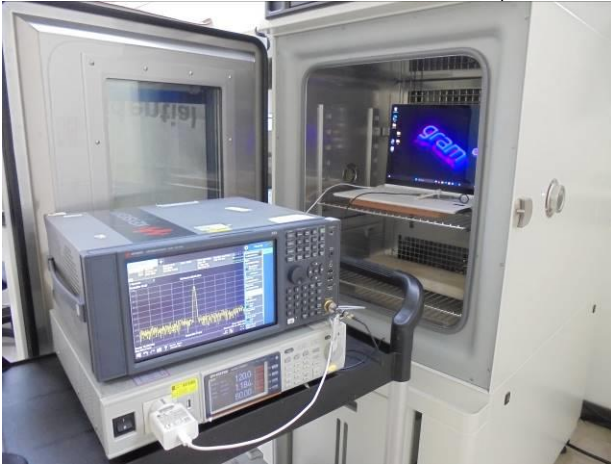
FCC_15_225_NFC_Conducted_INPAQ_Setup
