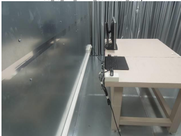
FCC_15_407_WLAN_Conduction_Setup
