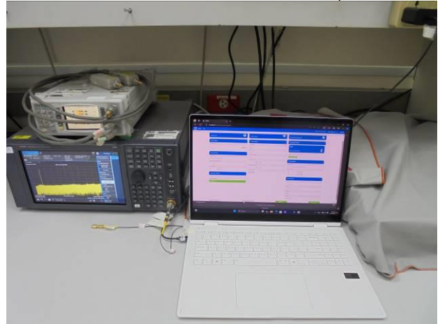
FCC_15_407_WLAN_6E_Conducted_Setup
