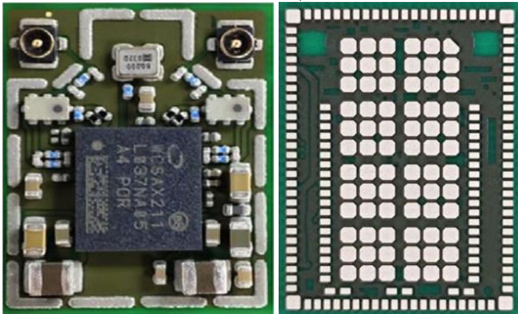
Figure 8 WLAN Combo Card, Without Shield and Back View
