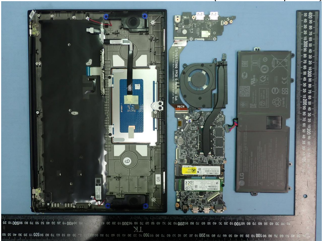
Figure 2 Internal View (Removed Components)
