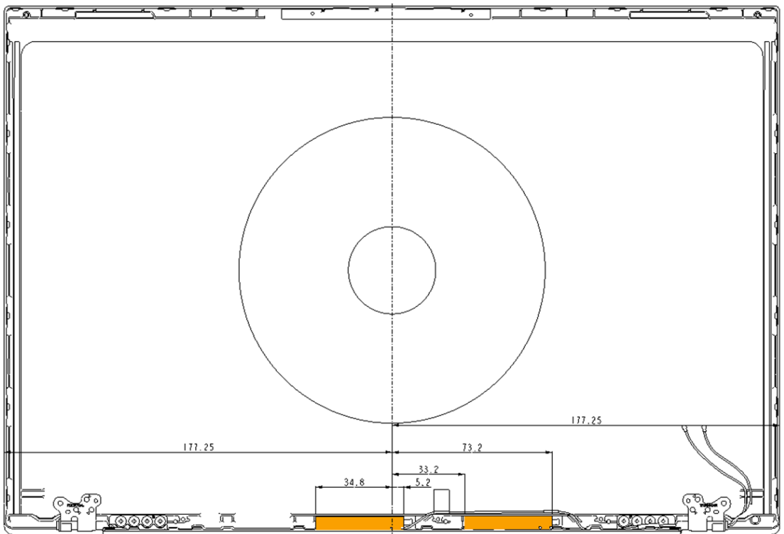
Figure 12 L1LRF008-CS-H, WLAN Combo Antenna Position
