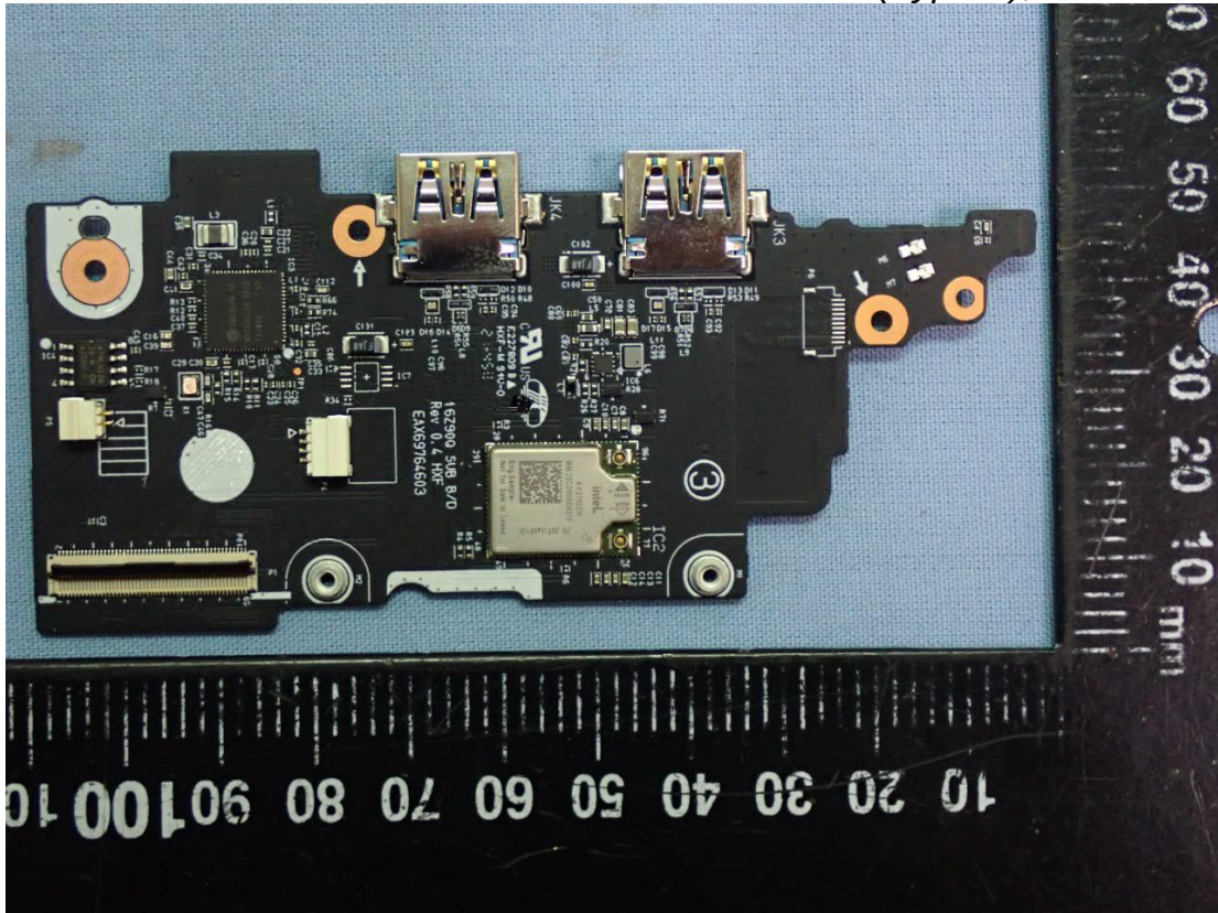
Figure 3 WLAN SUB Board (Type A), Front View
