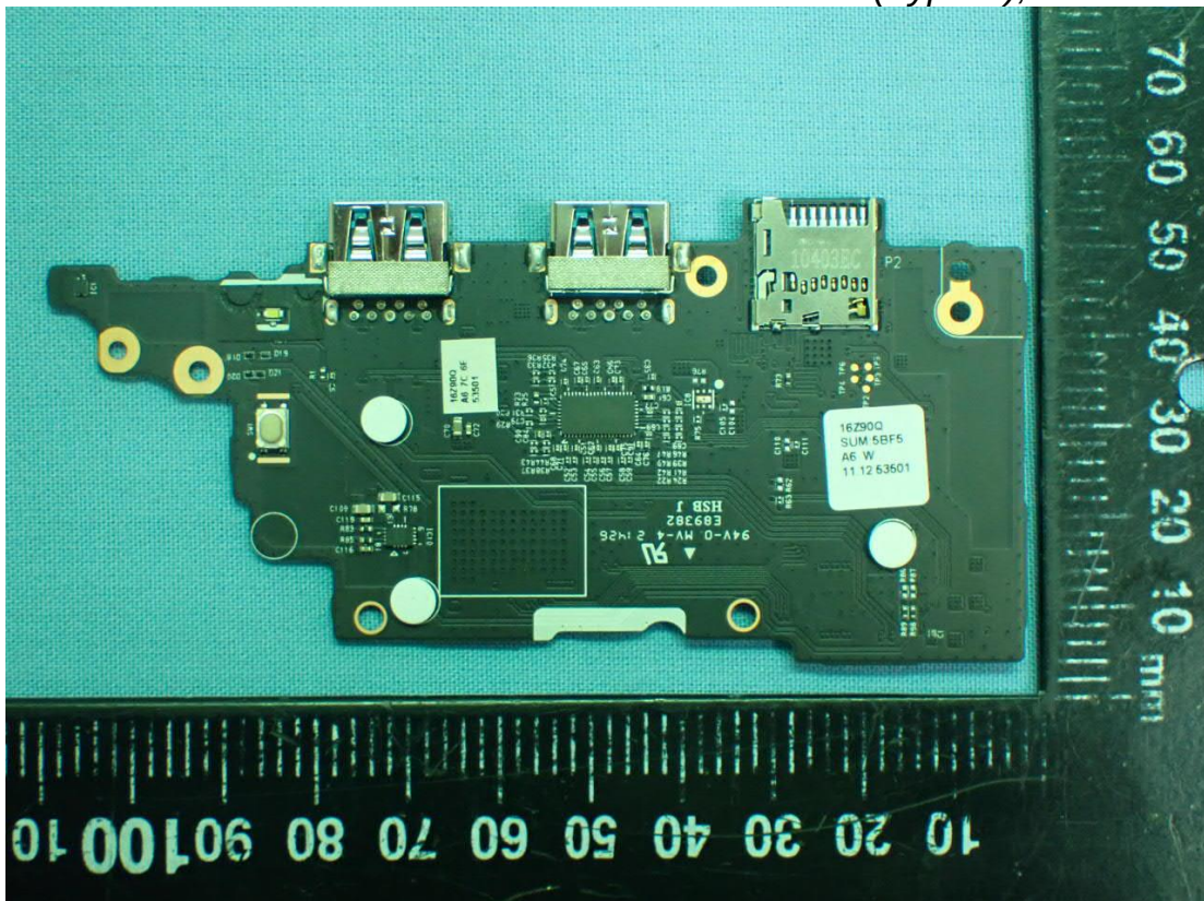
Figure 6 WLAN SUB Board (Type B), Back View
