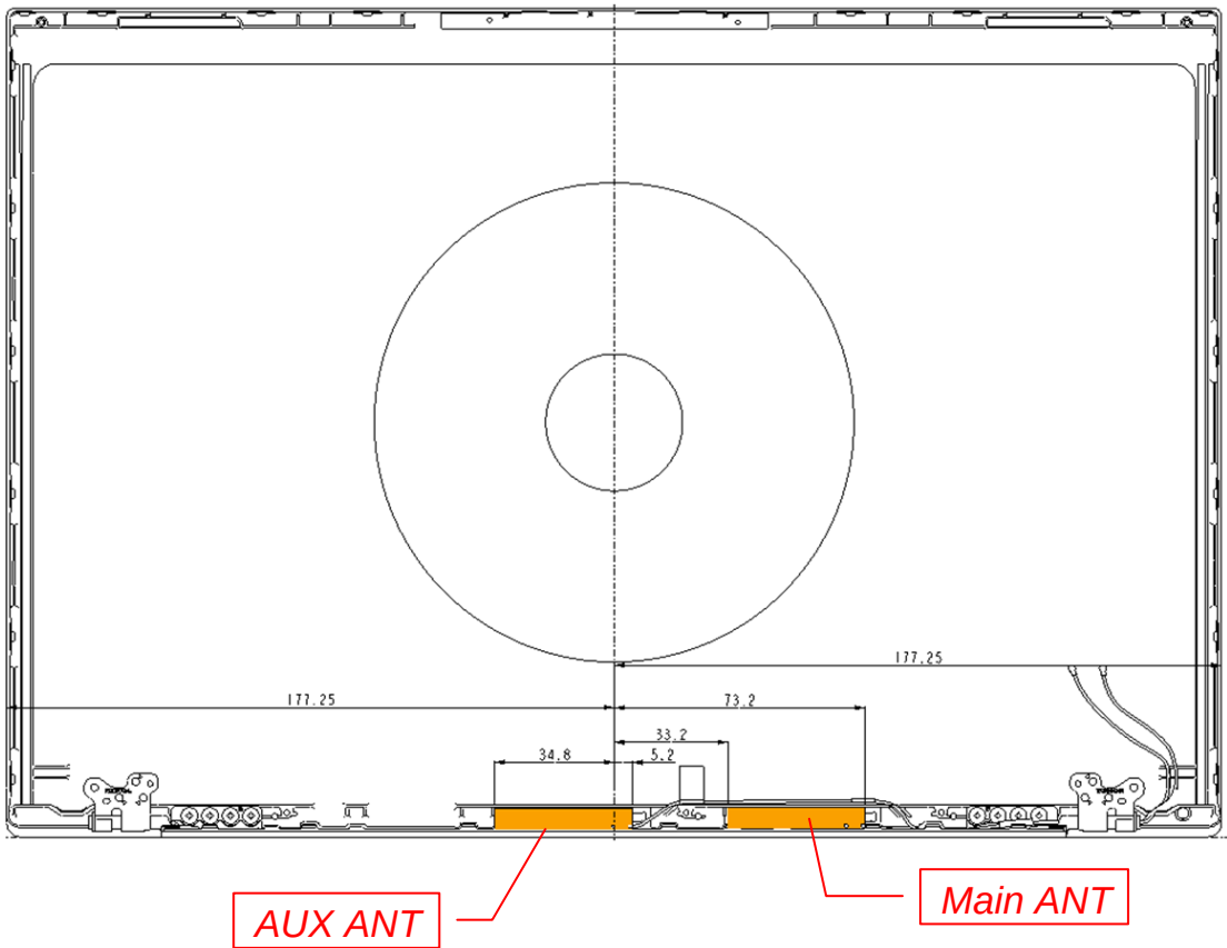
Figure 10 WA-P-LELE-04-009, WLAN Combo Antenna Position
