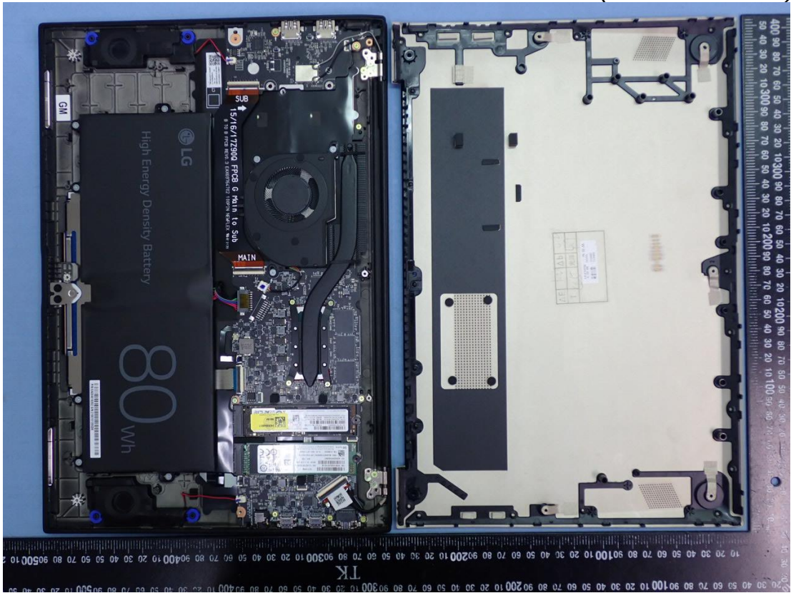
Figure 1 Internal View (Removed Cover)
