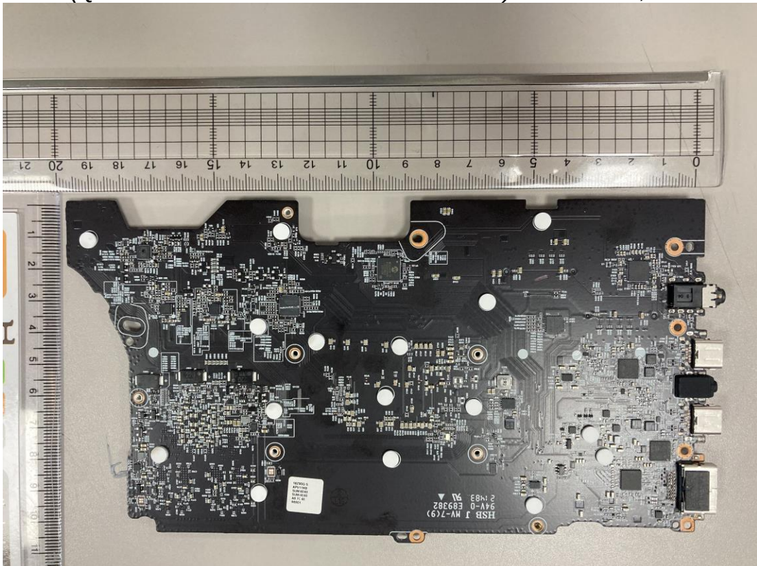
Figure 16 (QUEEN NVIDIA MAIN B/D PCB w/ TPM) Main Board, Back View
