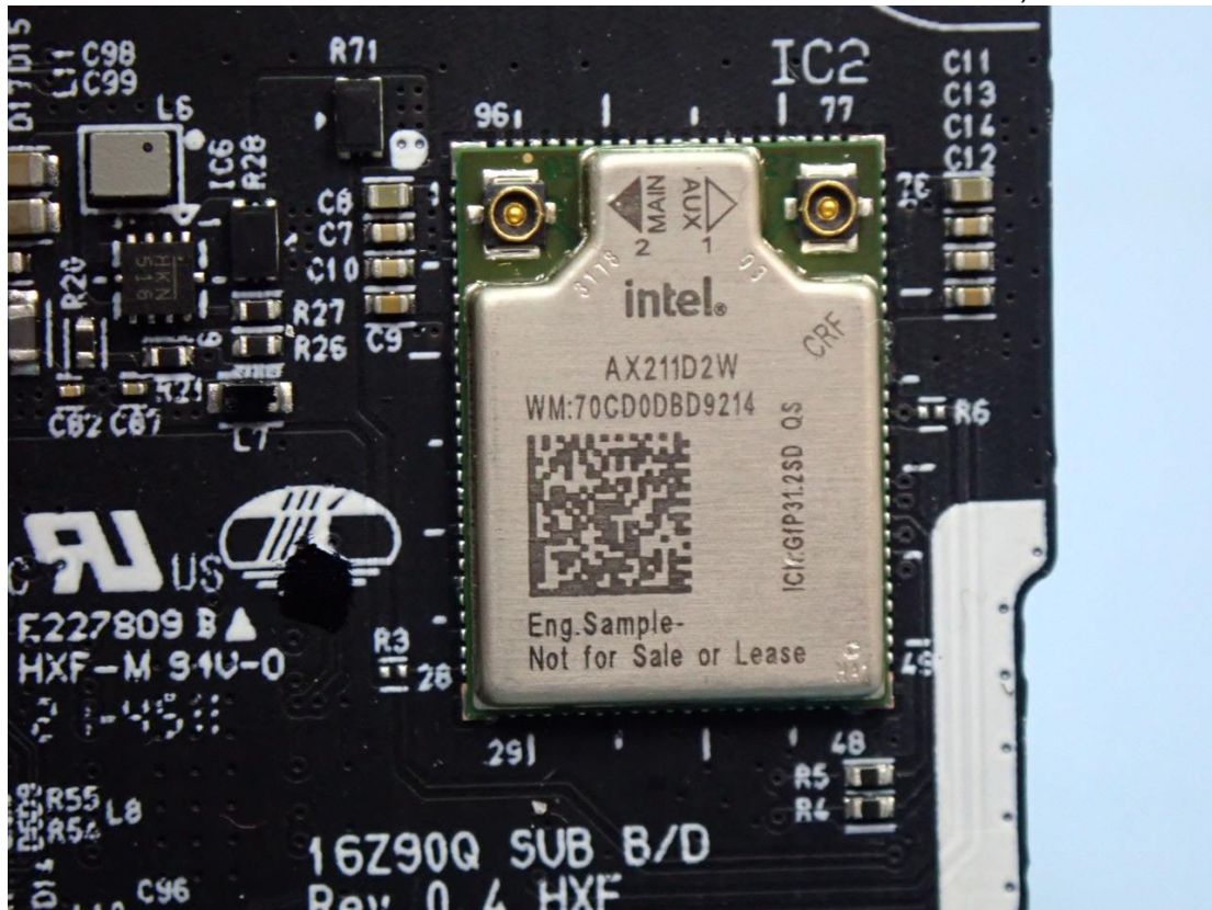
Figure 7 WLAN Combo Card, Front View
