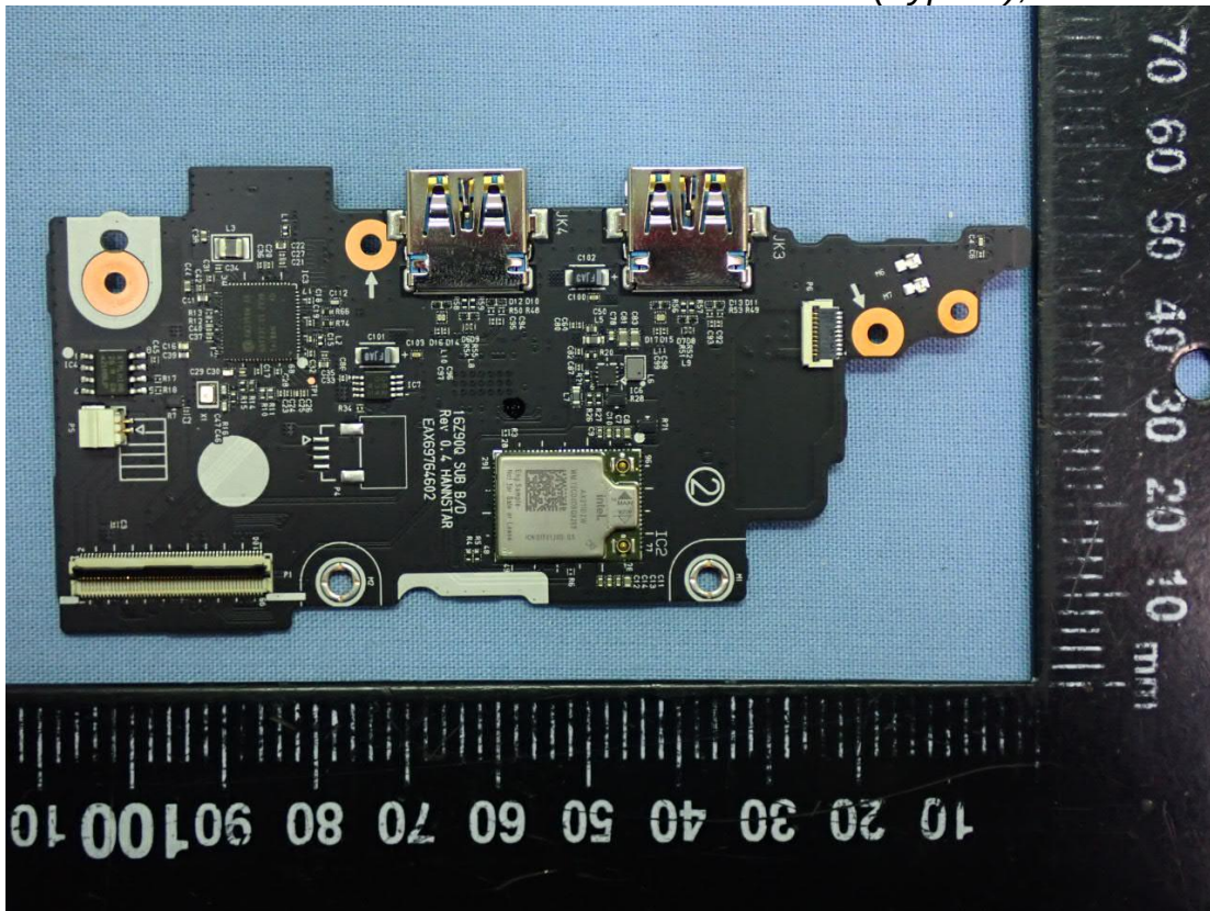
Figure 5 WLAN SUB Board (Type B), Front View
