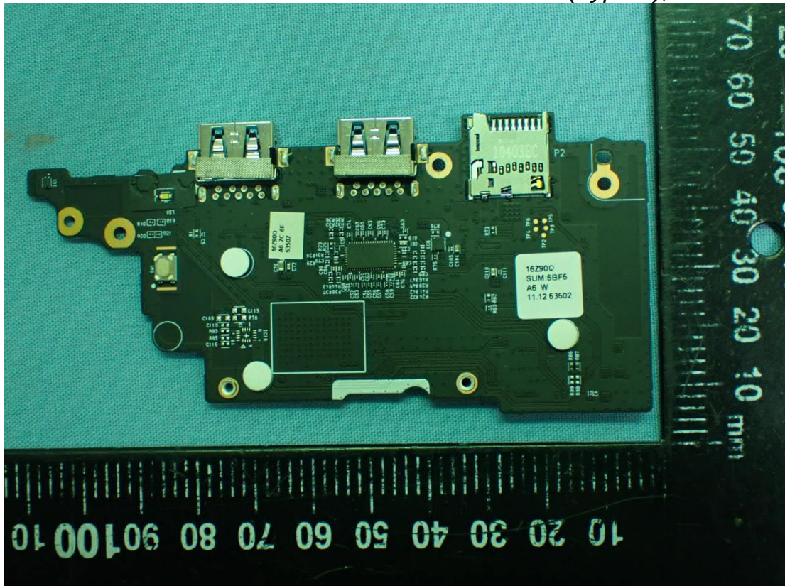
Figure 4 WLAN SUB Board (Type A), Back View
