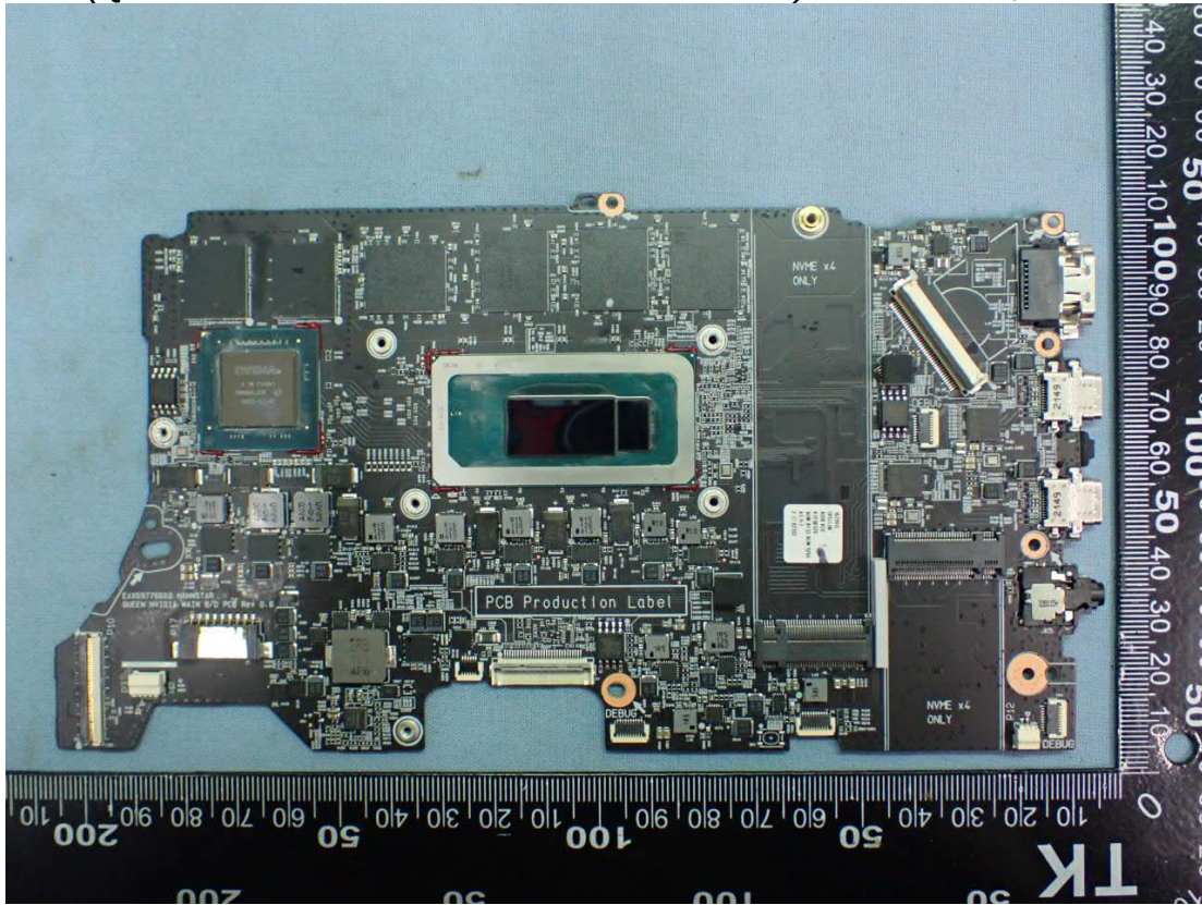
Figure 13 (QUEEN NVIDIA MAIN B/D PCB w/o TPM) Main Board, Front View
