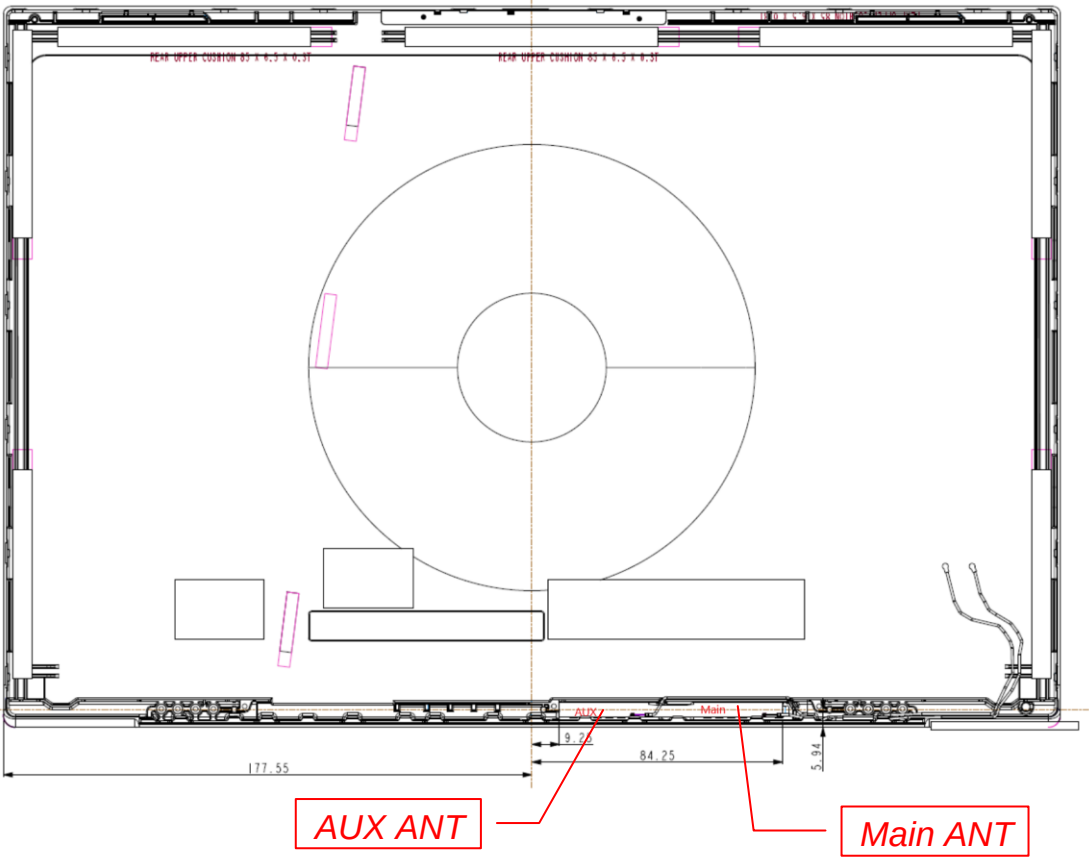
Figure 3 This Time Add WA-P-LBLB-04-110, WLAN Combo Antenna Position
