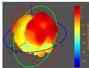
AUX Antenna
