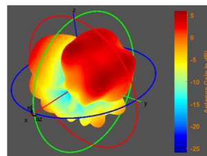
Main Antenna
