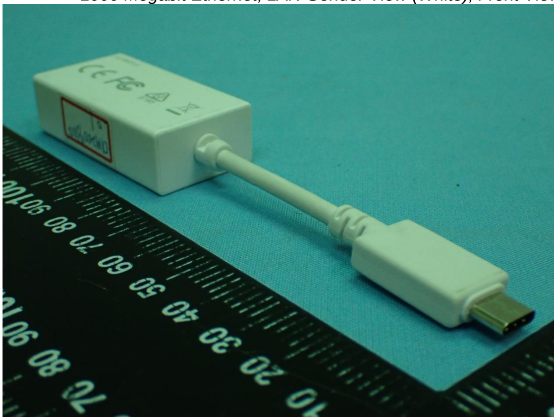
Figure 10 1000 Megabit Ethernet, LAN Gender View (White), Front View
