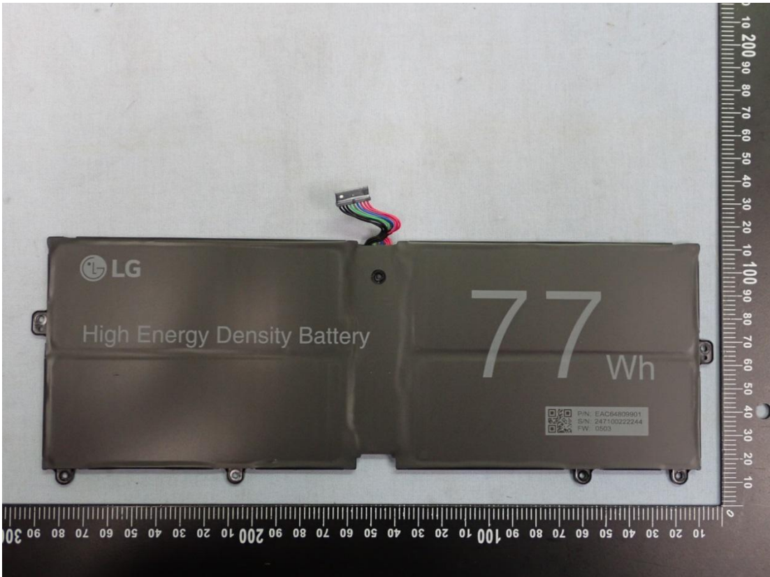
Figure 50 Battery, Front View
