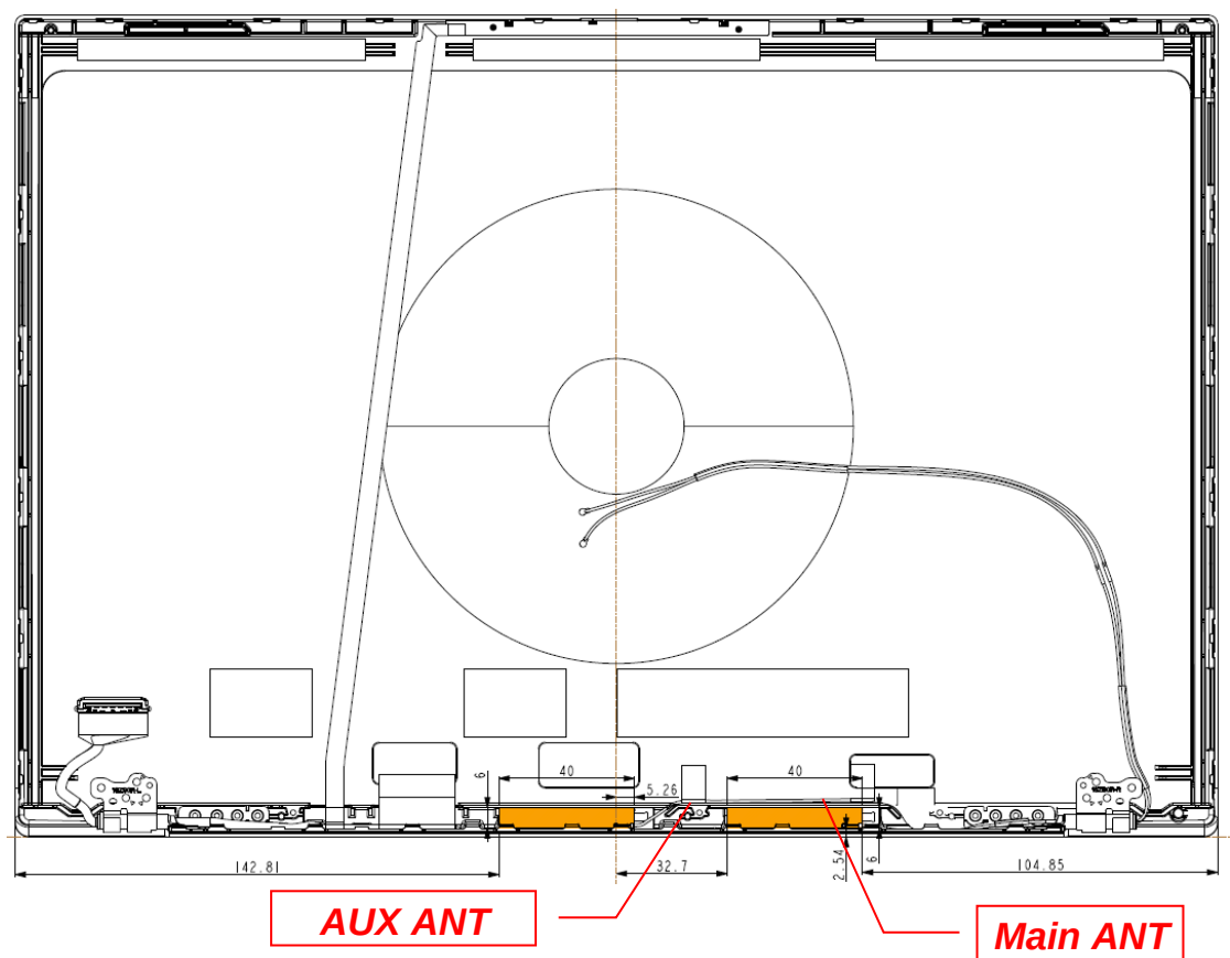
Figure 41 WLAN Combo Antenna Position with LUXSHARE L1LRF017-CS-H
