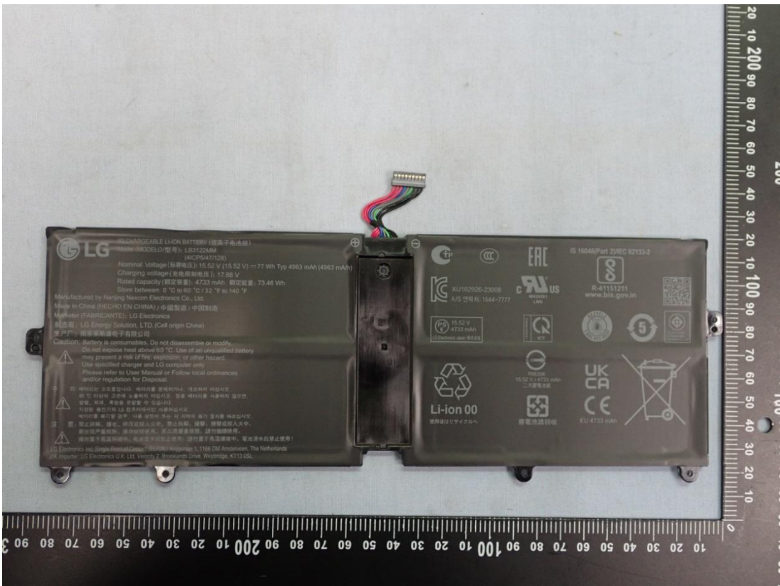
Figure 51 Battery, Back View
