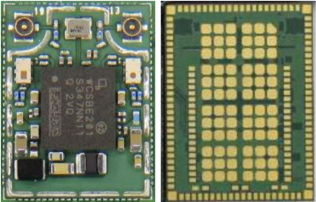
Figure 39 WLAN Combo Card, Without Shield and Back View
