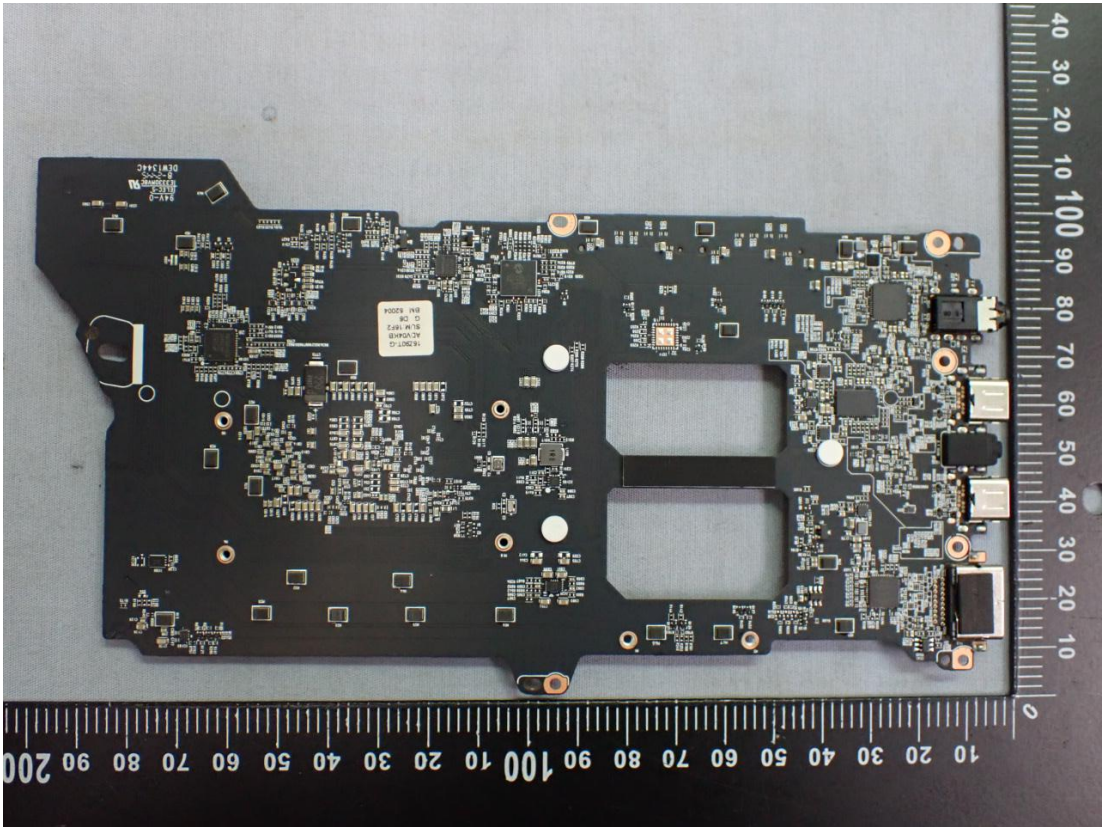
Figure 37 Main Board, Back View
