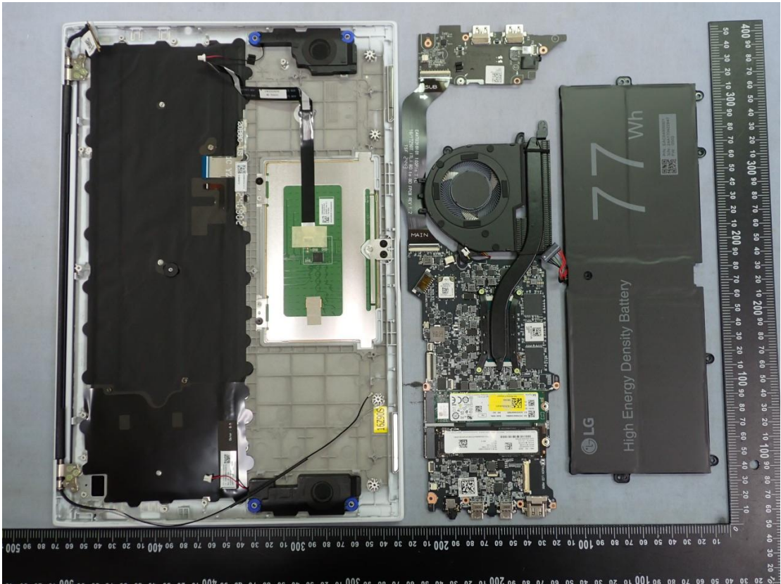
Figure 33 Internal View
