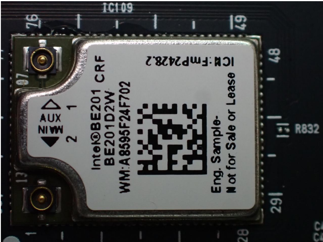
Figure 38 WLAN Combo Card View
