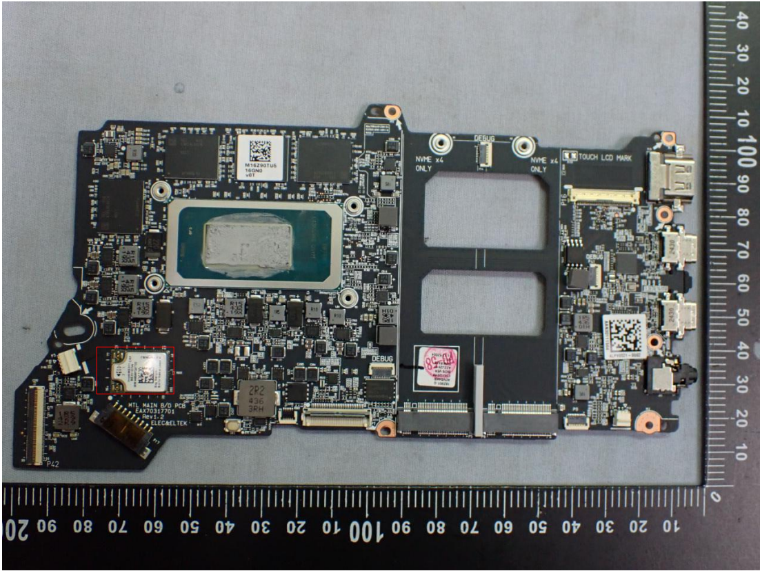
Figure 36 Main Board, Front View
