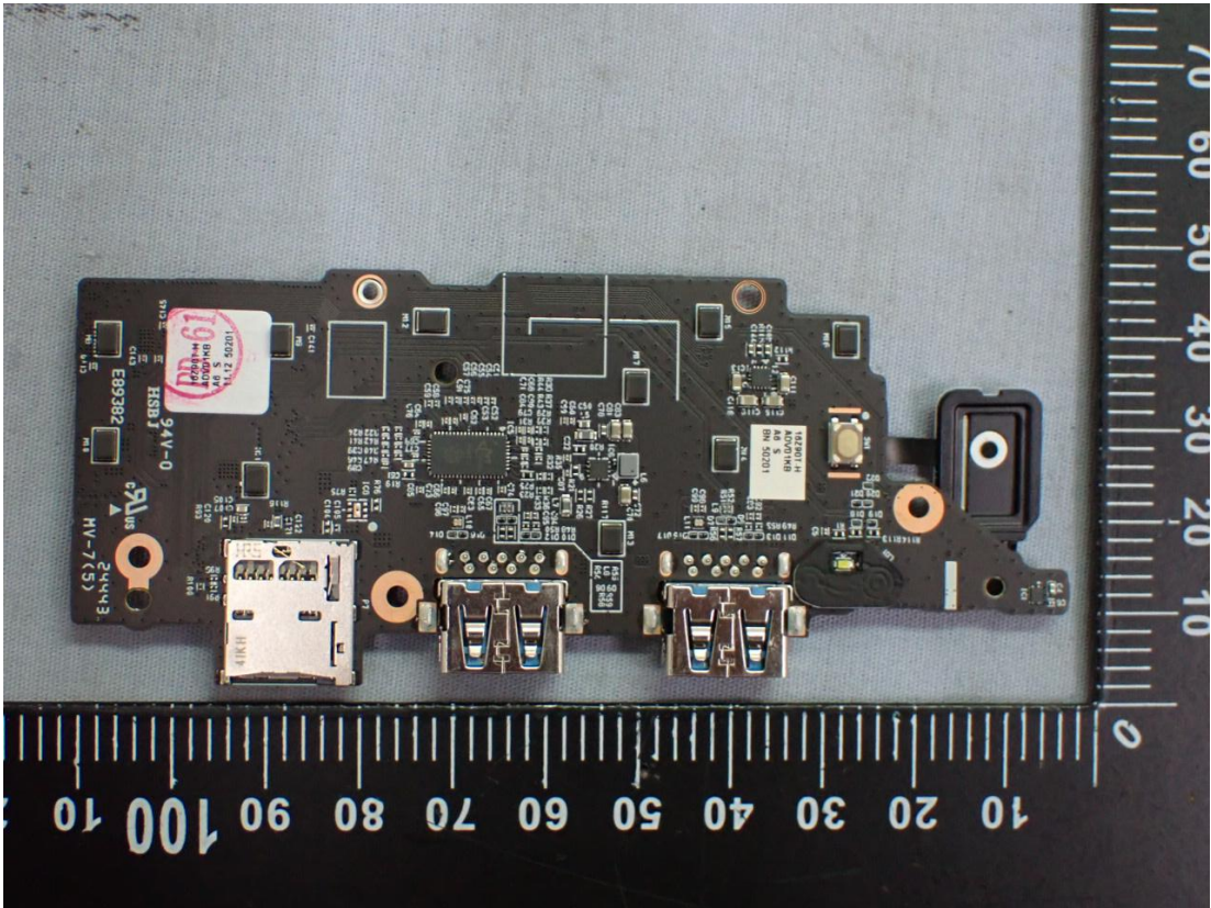
Figure 35 SUB Board, Back View
