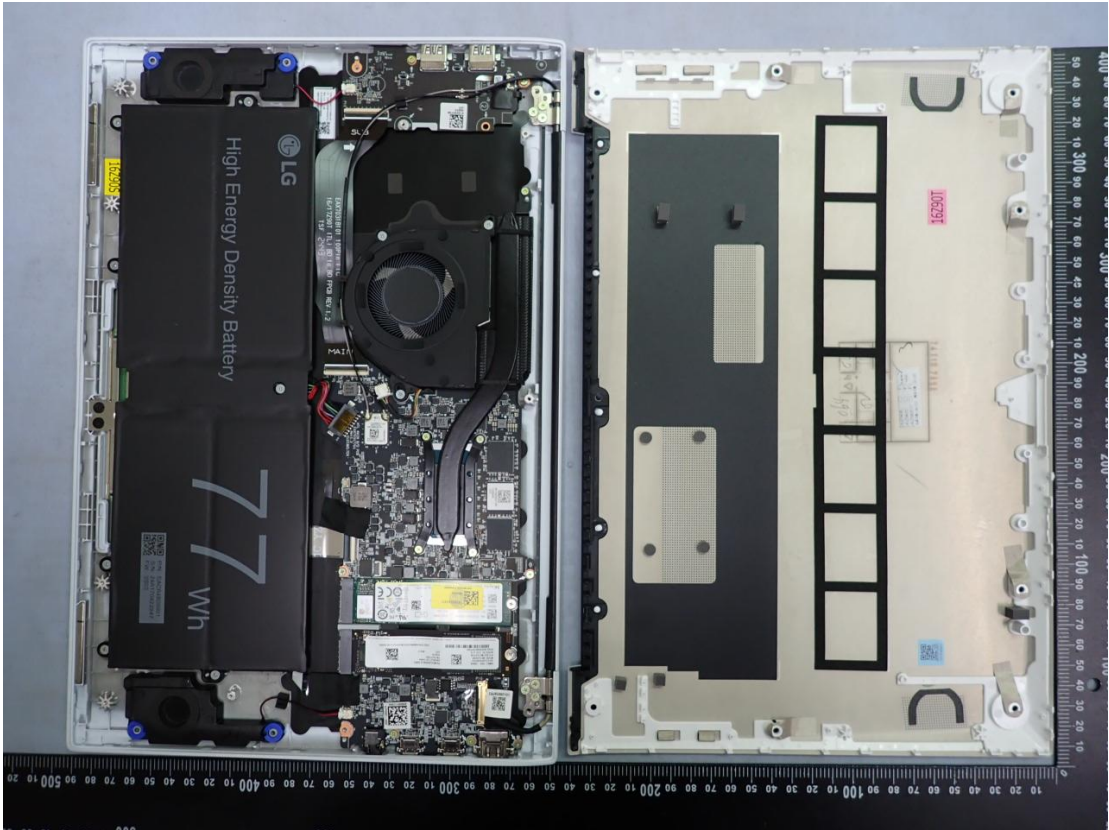
Figure 32 Internal View
