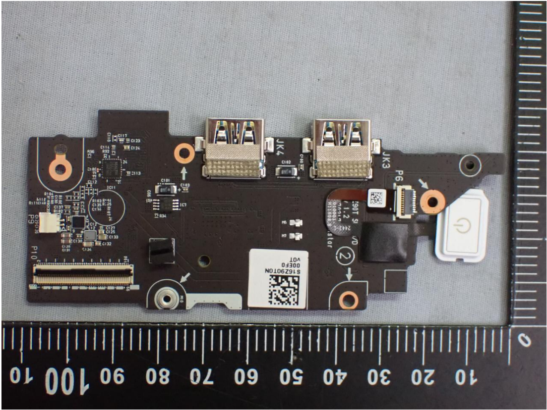
Figure 34 SUB Board, Front View
