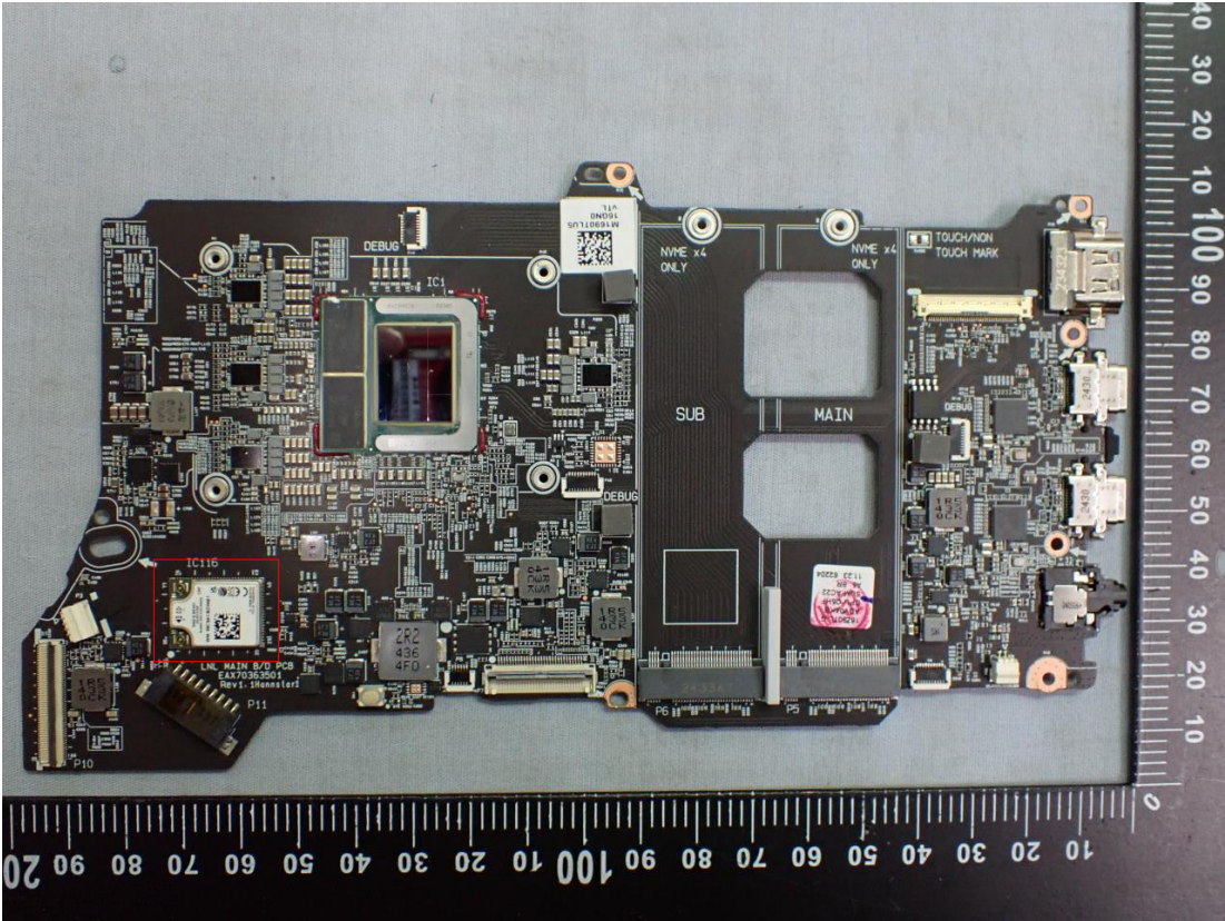
Figure 44 Main Board, Front View
