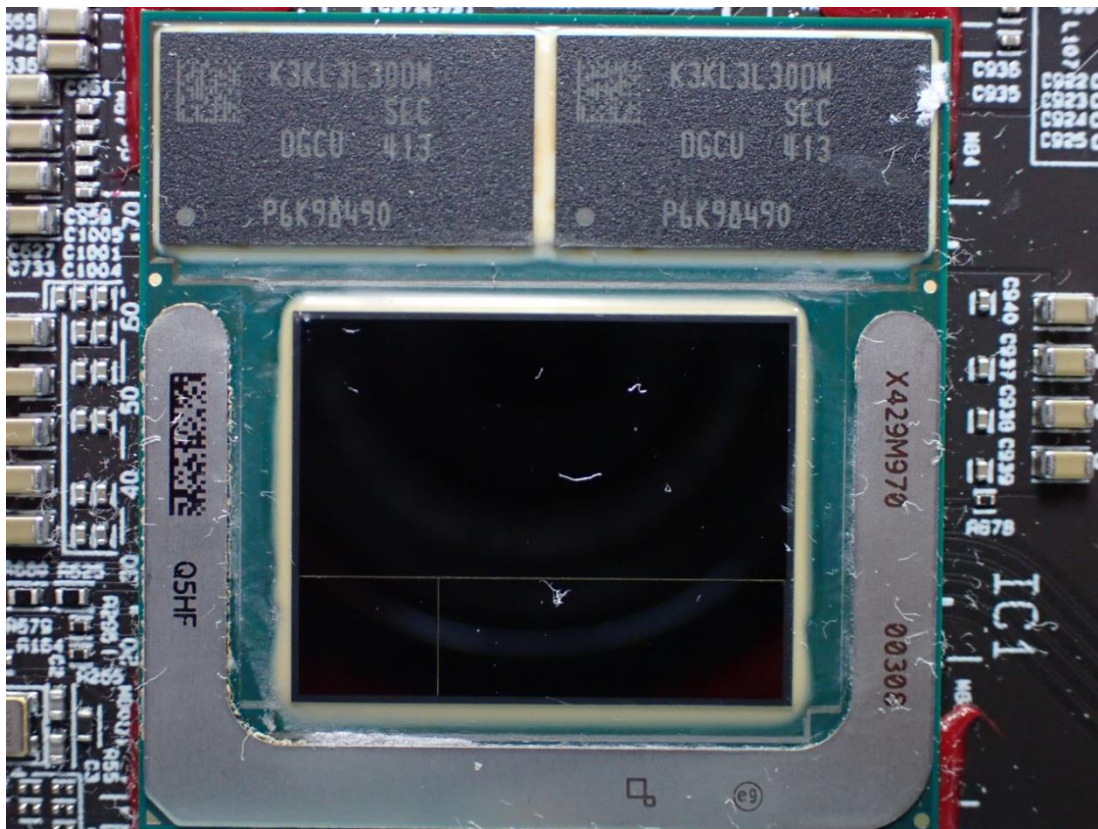
Figure 62 CPU +RAM View
