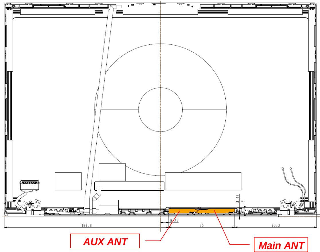
Figure 49 WLAN Combo Antenna Position with LUXSHARE L1LRF017-CS-H
