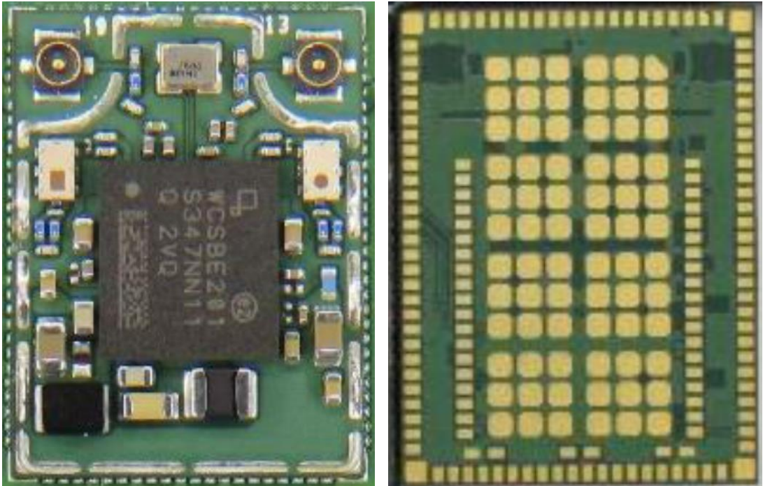
Figure 47 WLAN Combo Card, Without Shield and Back View
