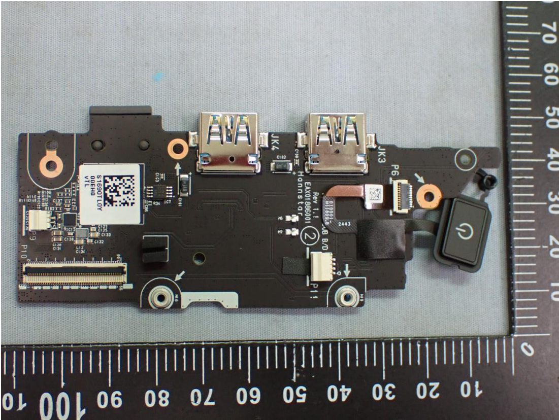
Figure 42 SUB Board, Front View
