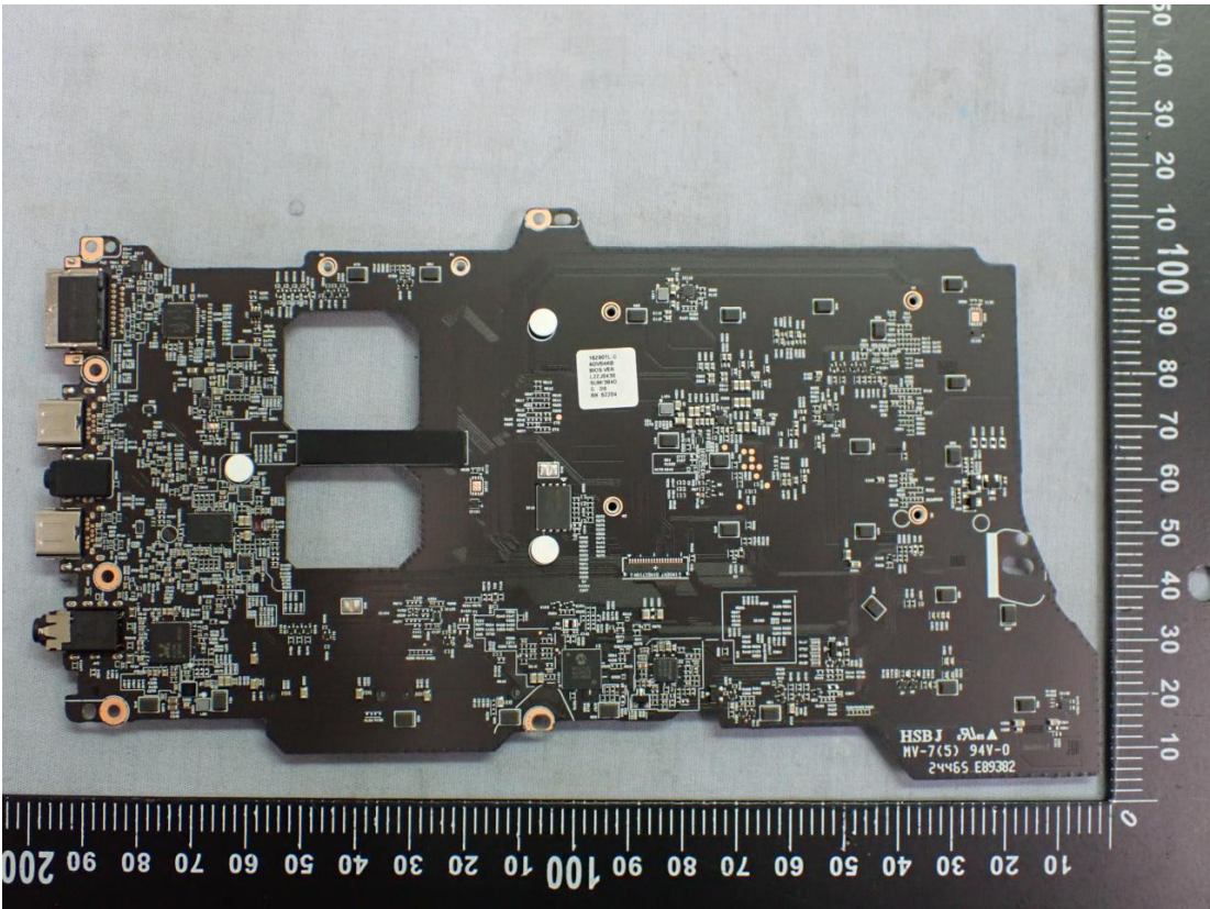
Figure 45 Main Board, Back View
