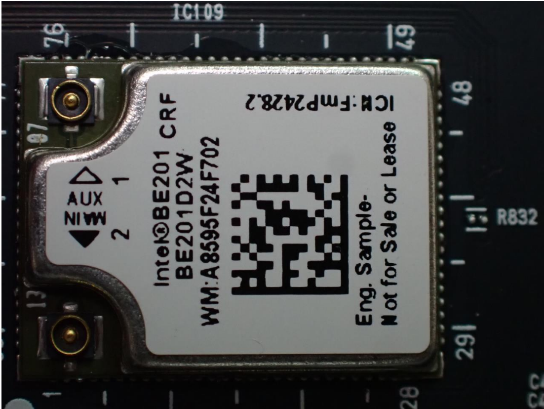
Figure 46 WLAN Combo Card View
