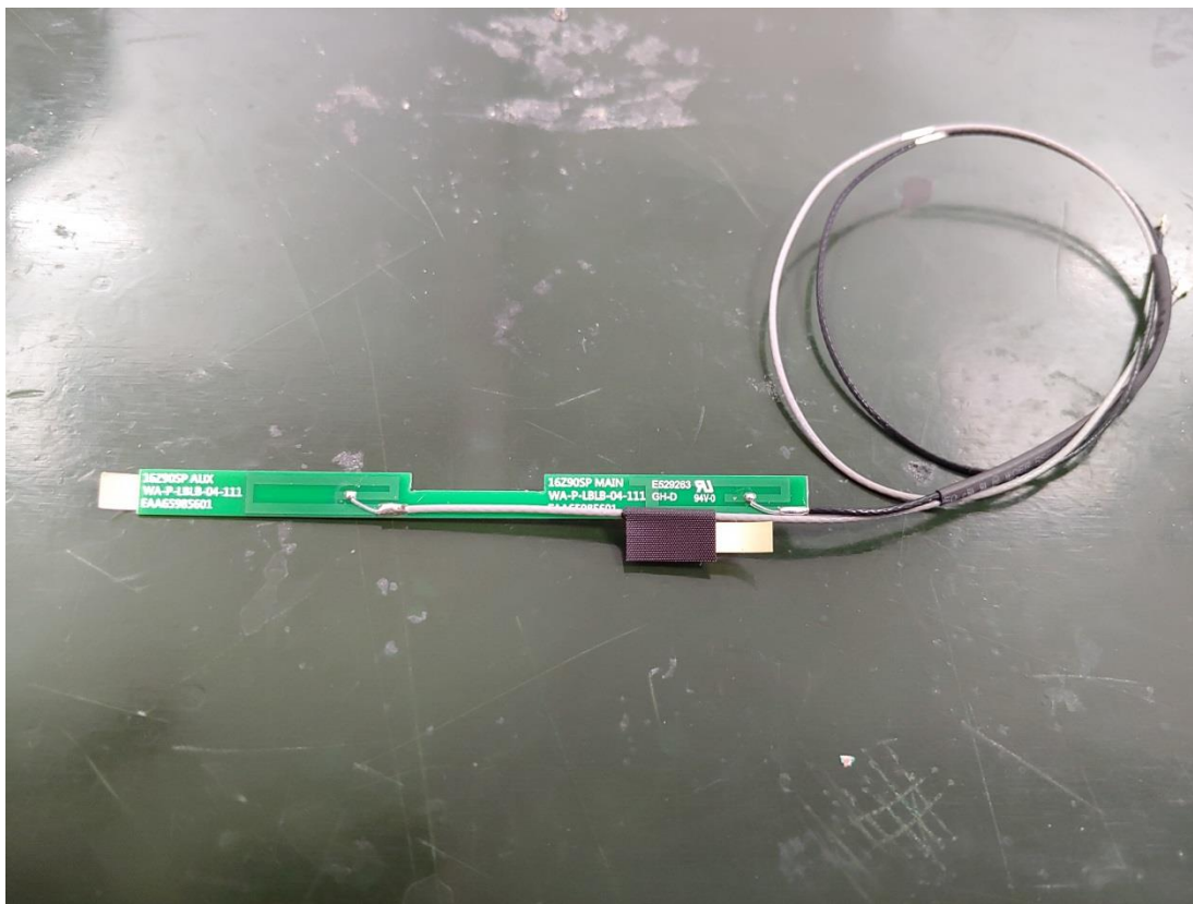
Figure 41 WLAN Combo Antenna, Front View
