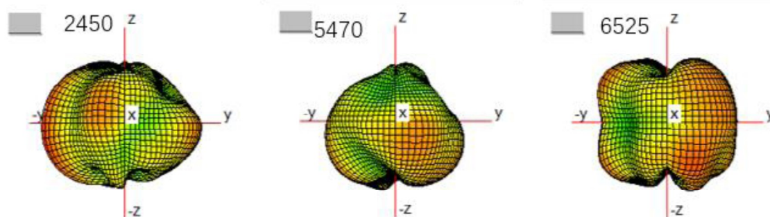
Main Antenna-2
