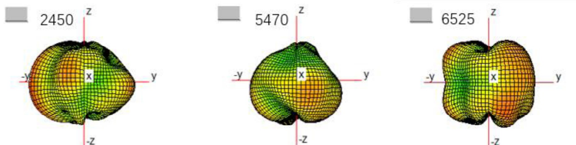
Main Antenna-2
