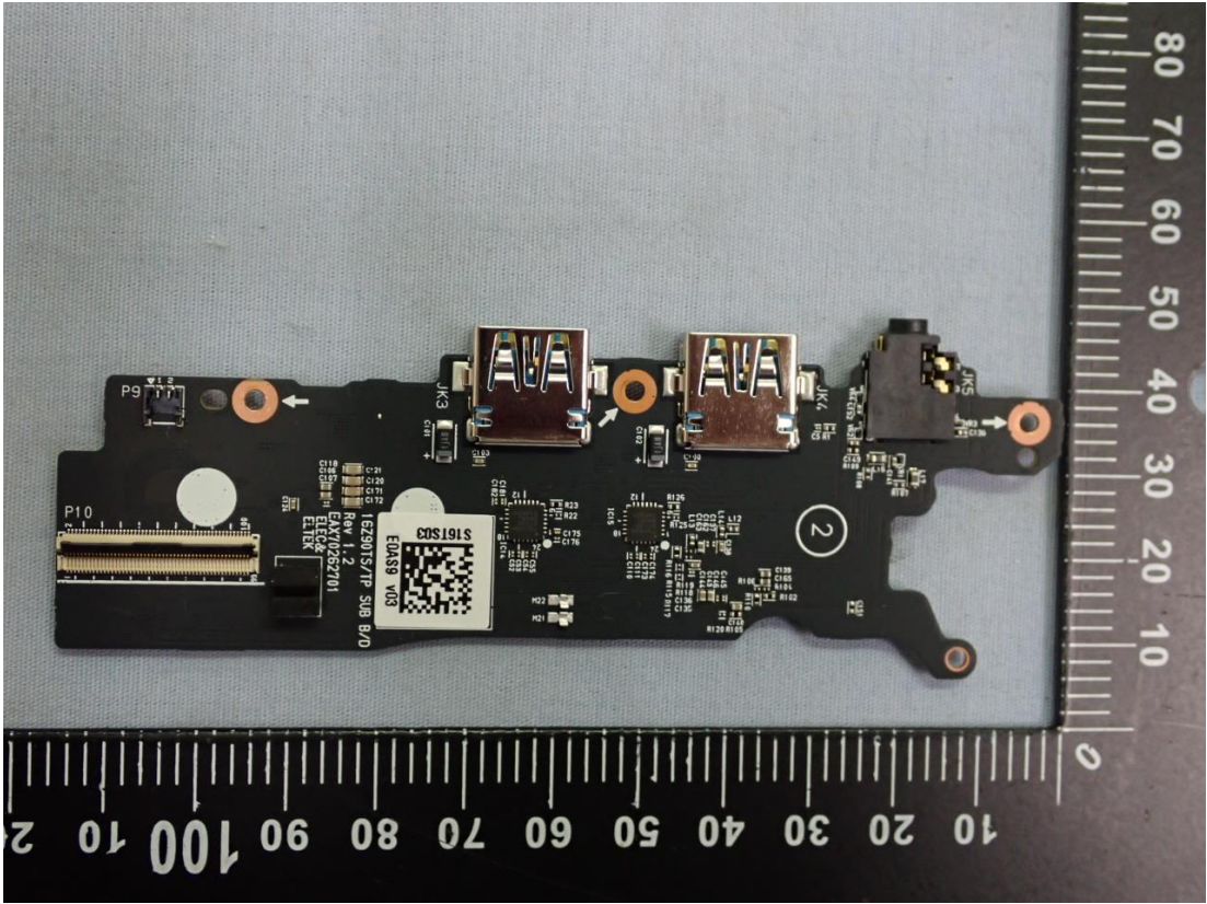
Figure 28 SUB Board, Front View
