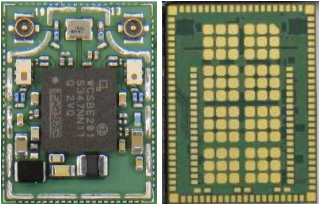
Figure 33 WLAN Combo Card, Without Shield and Back View
