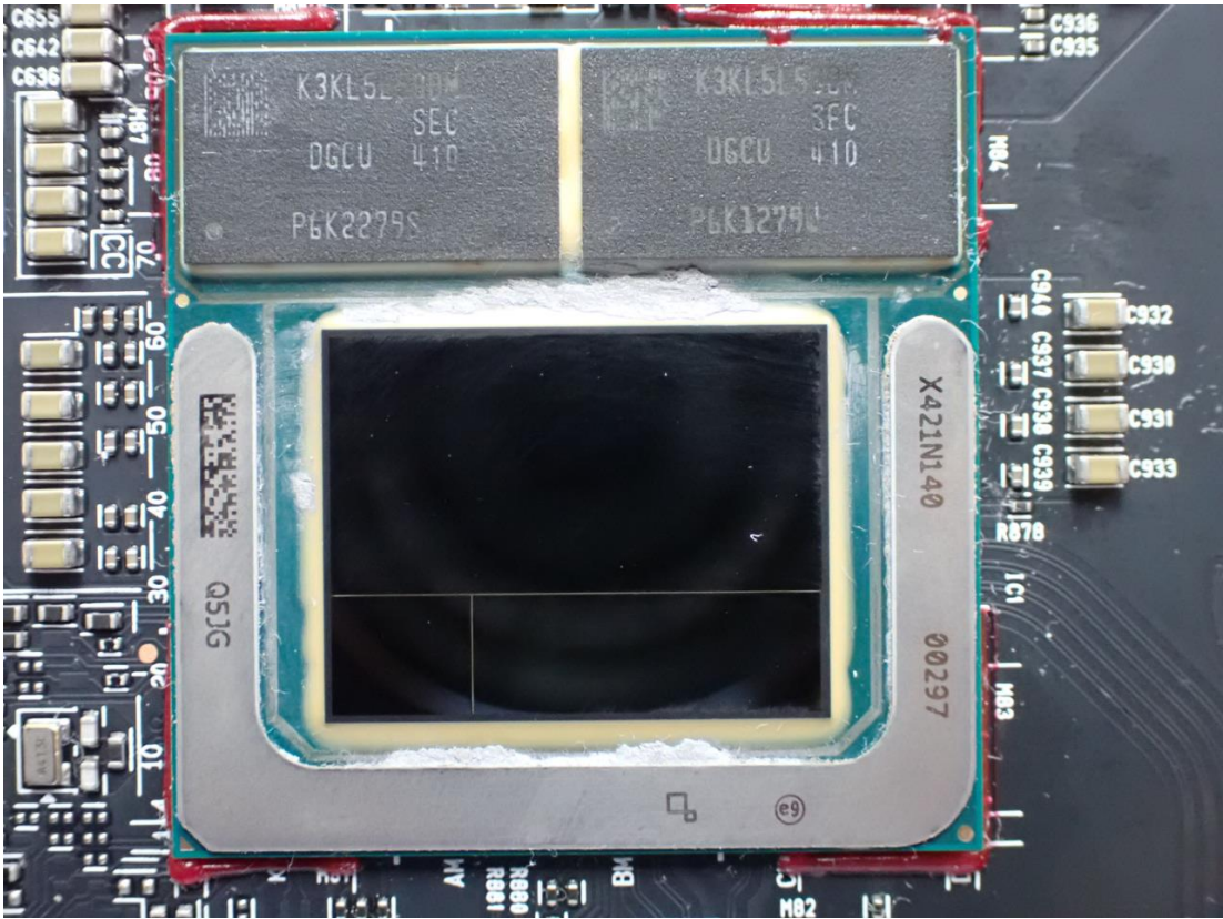
Figure 42 CPU+RAM View
