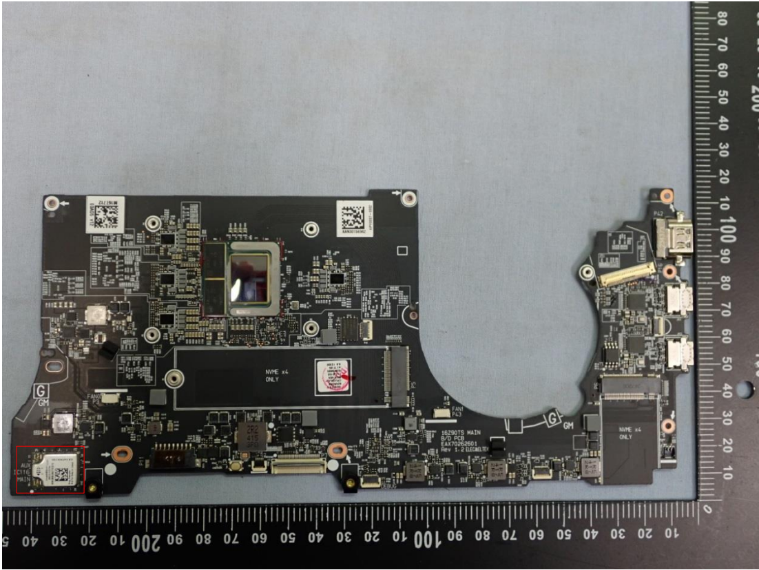
Figure 30 Main Board, Front View
