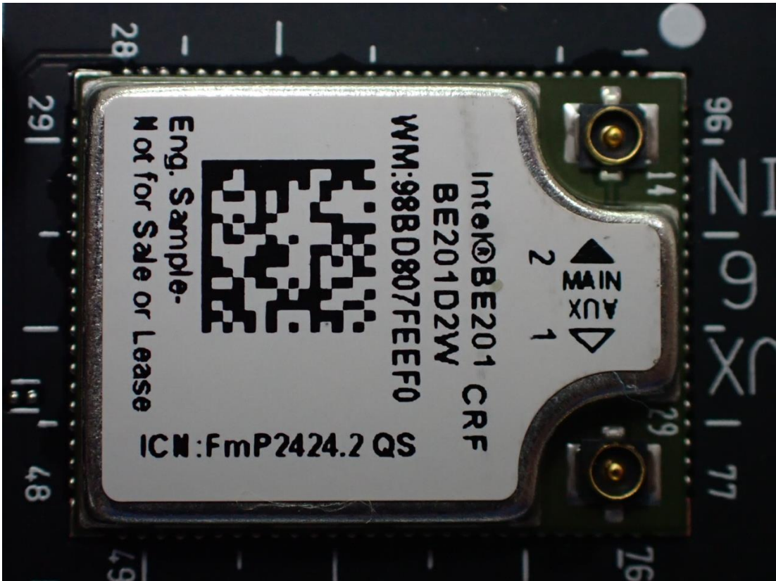
Figure 32 WLAN Combo Card View
