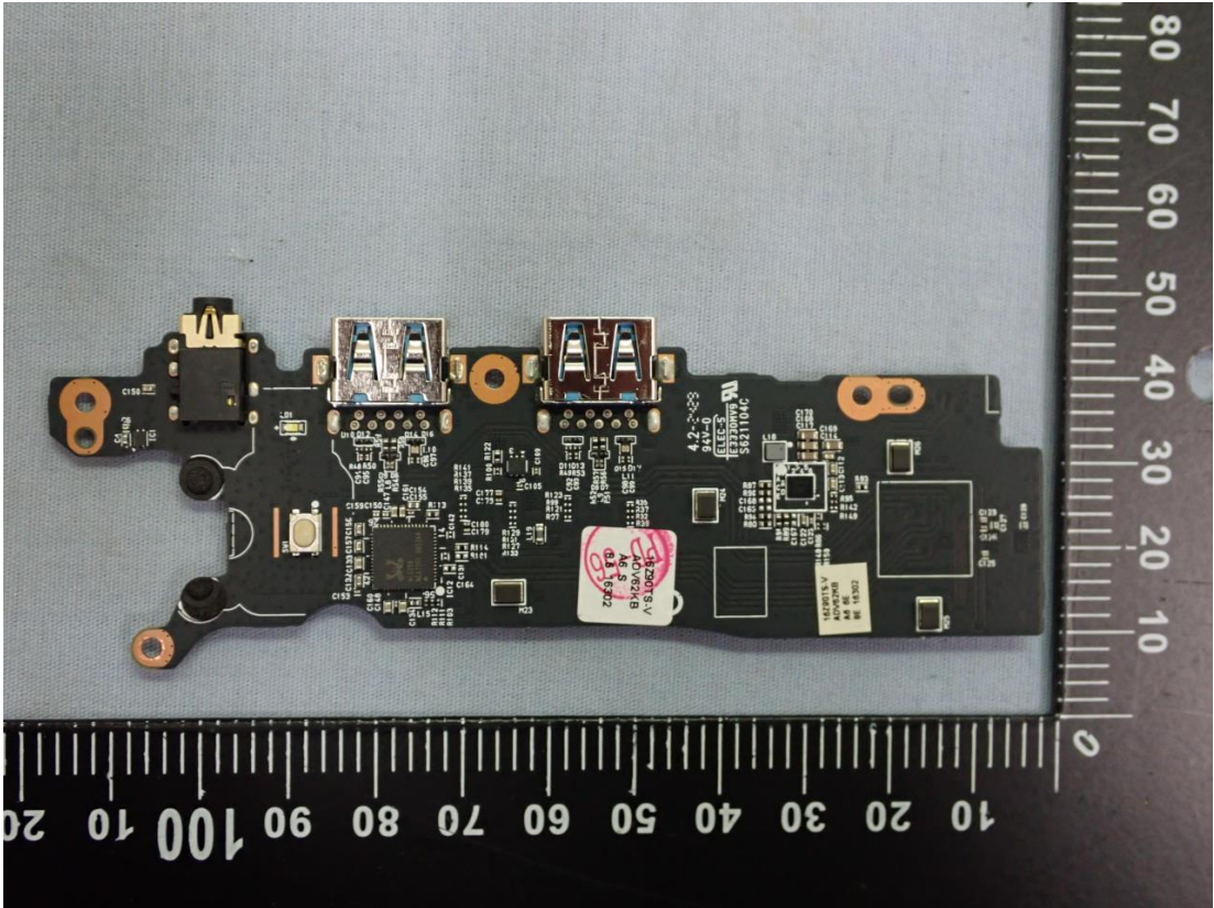
Figure 29 SUB Board, Back View
