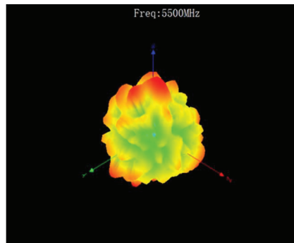
Main Antenna 1
