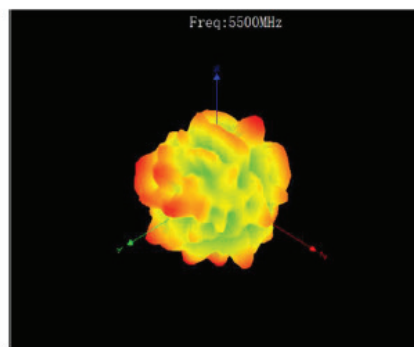
AUX Antenna 1
