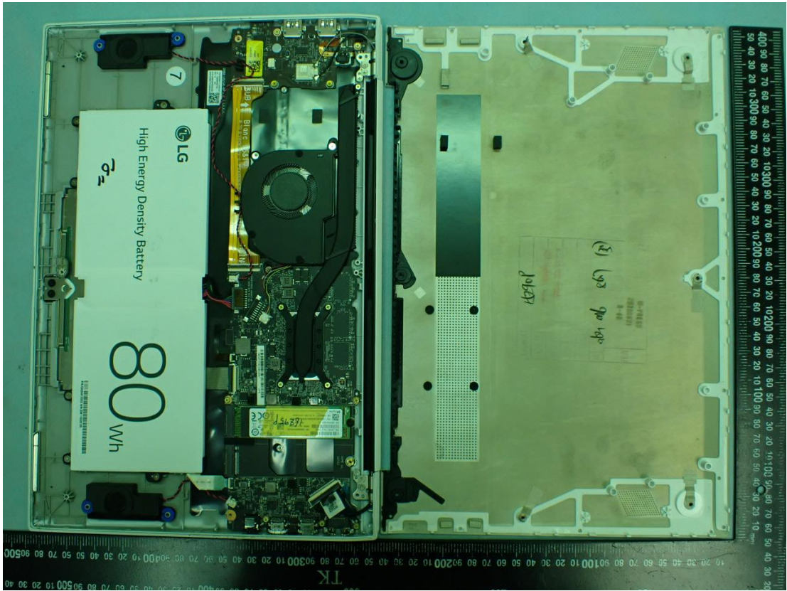
Figure 15 Internal View
