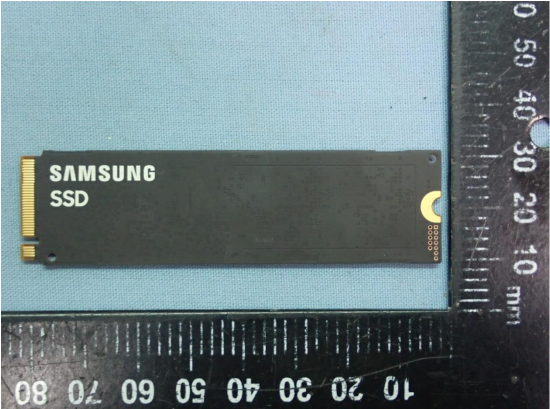
Figure 6 SAMSUNG, SSD (2TB), Back View
