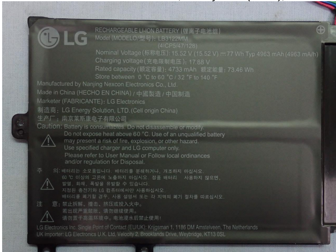
Figure 25 This Time add, Battery Pack (77Wh), Label View
