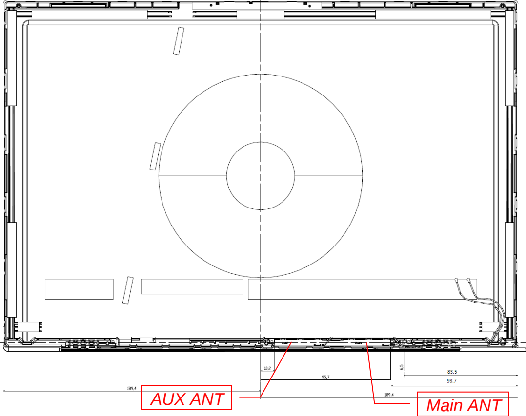
Figure 34 WA-P-LBLB-04-108 WLAN Combo Antenna Position
