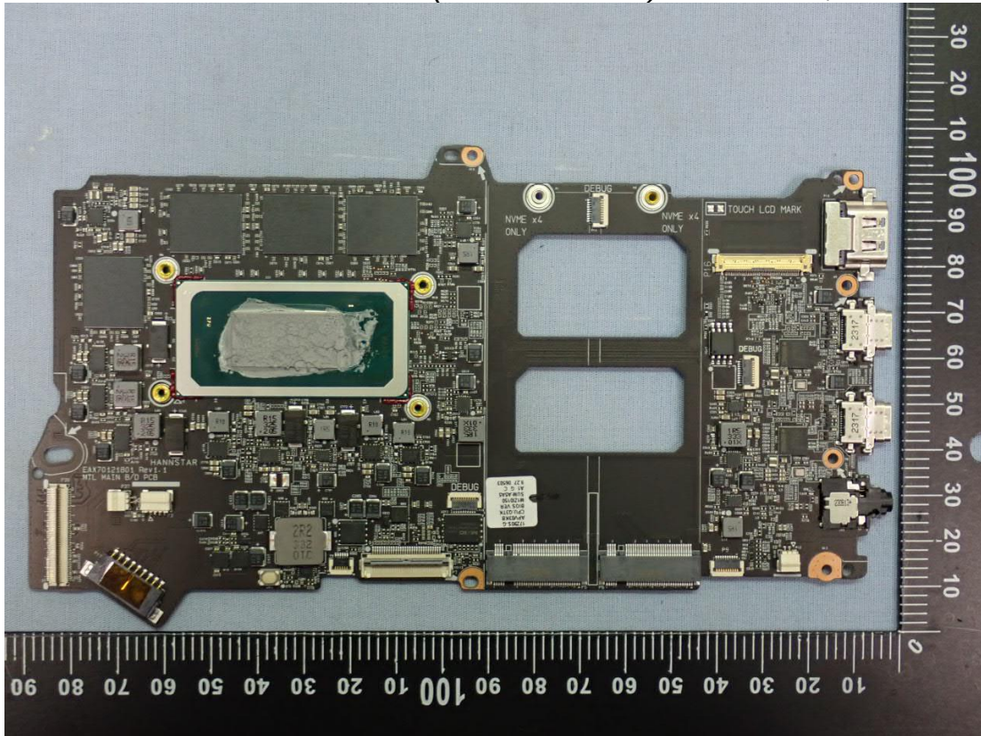
Figure 17 This Time add (MTL MAIN B/D) Main Board, Front View
