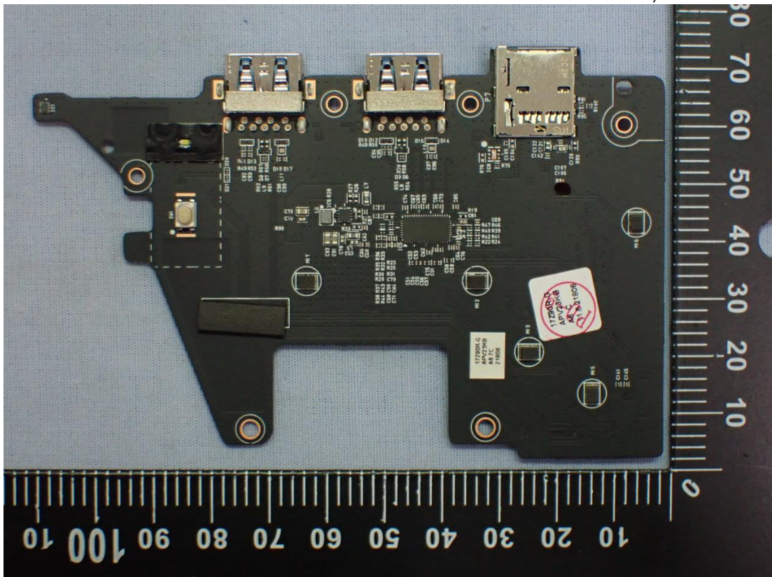
Figure 20 WLAN SUB Board, Back View
