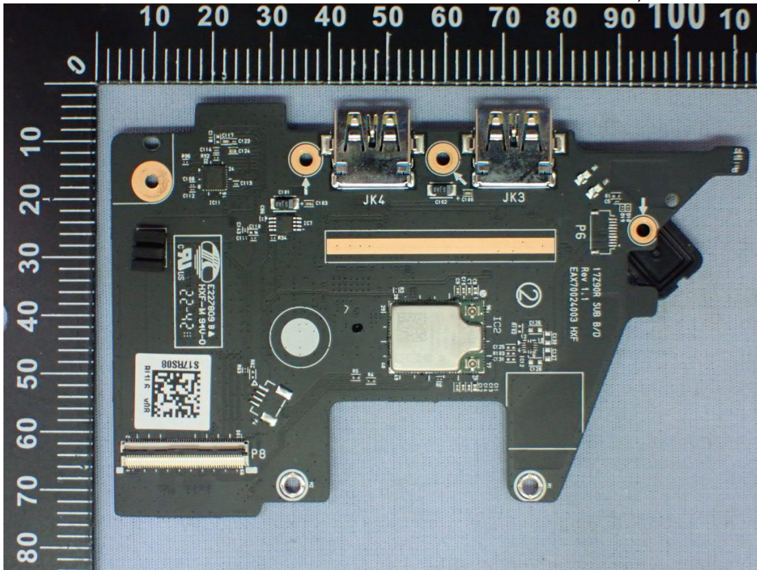
Figure 19 WLAN SUB Board, Front View
