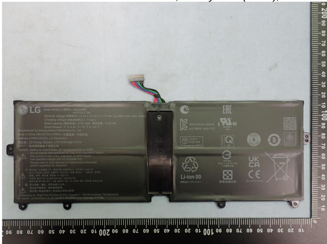
Figure 24 This Time add, Battery Pack (77Wh), Back View
