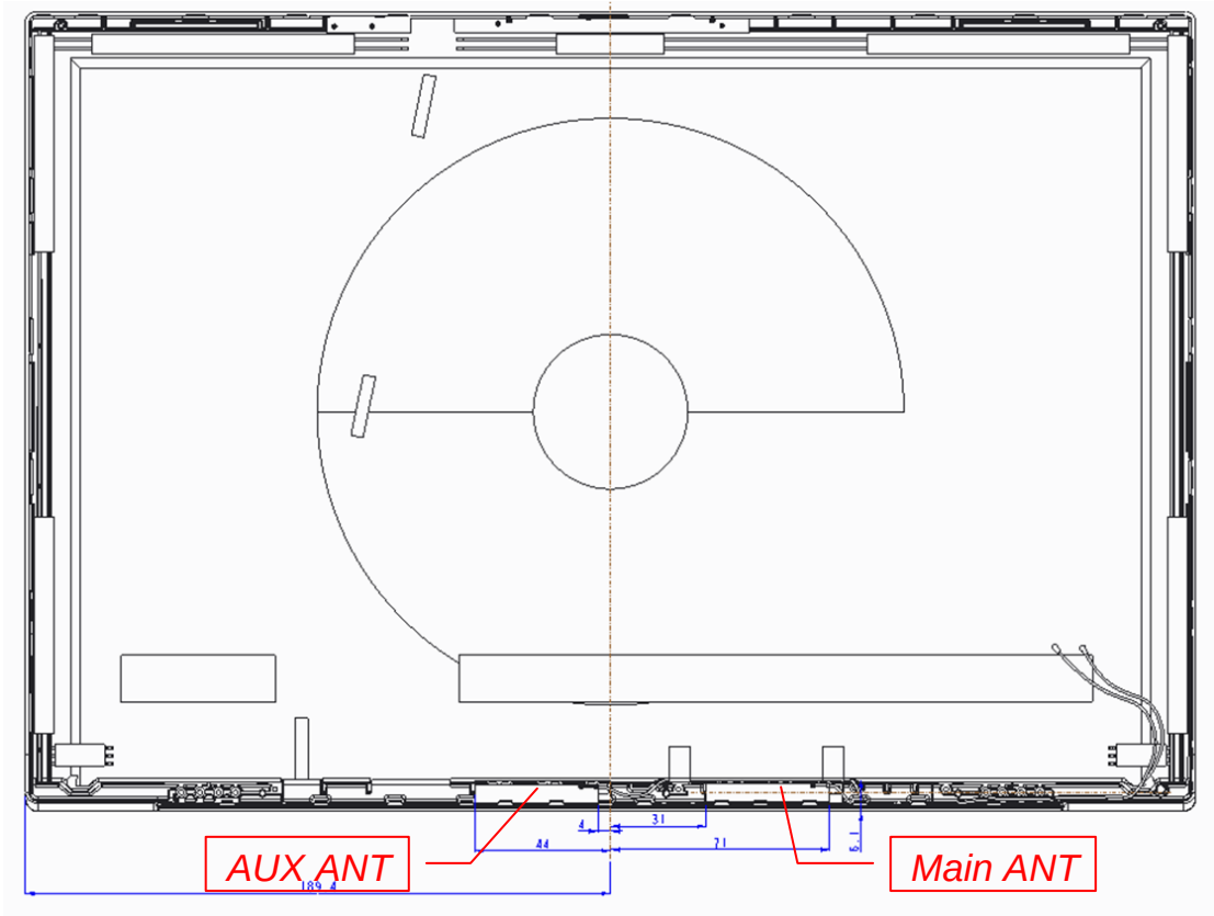
Figure 28 WA-P-LELE-04-011, WLAN Combo Antenna Position
