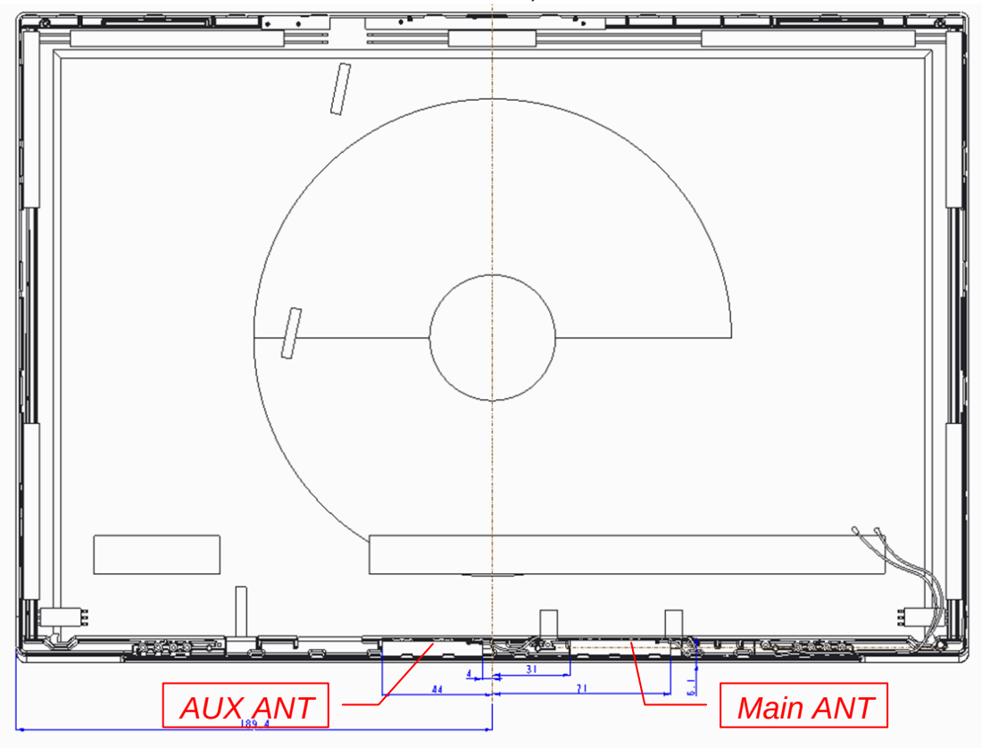
Figure 30 L1LRF009-CS-H, WLAN Combo Antenna Position
