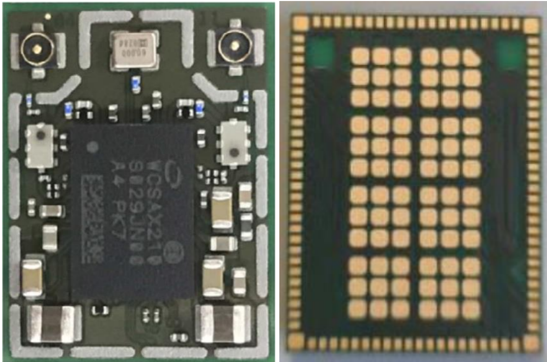
Figure 22 WLAN Combo Card, Without Shield and Back View
