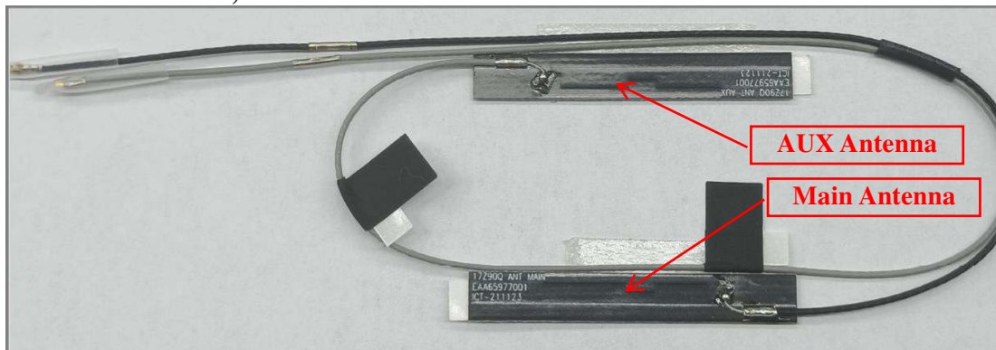
L1LRF009-CS-H, Antenna View
