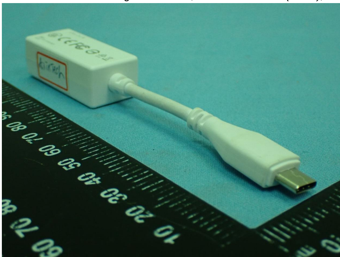
Figure 14 100 Megabit Ethernet, LAN Gender View (White), Back View
