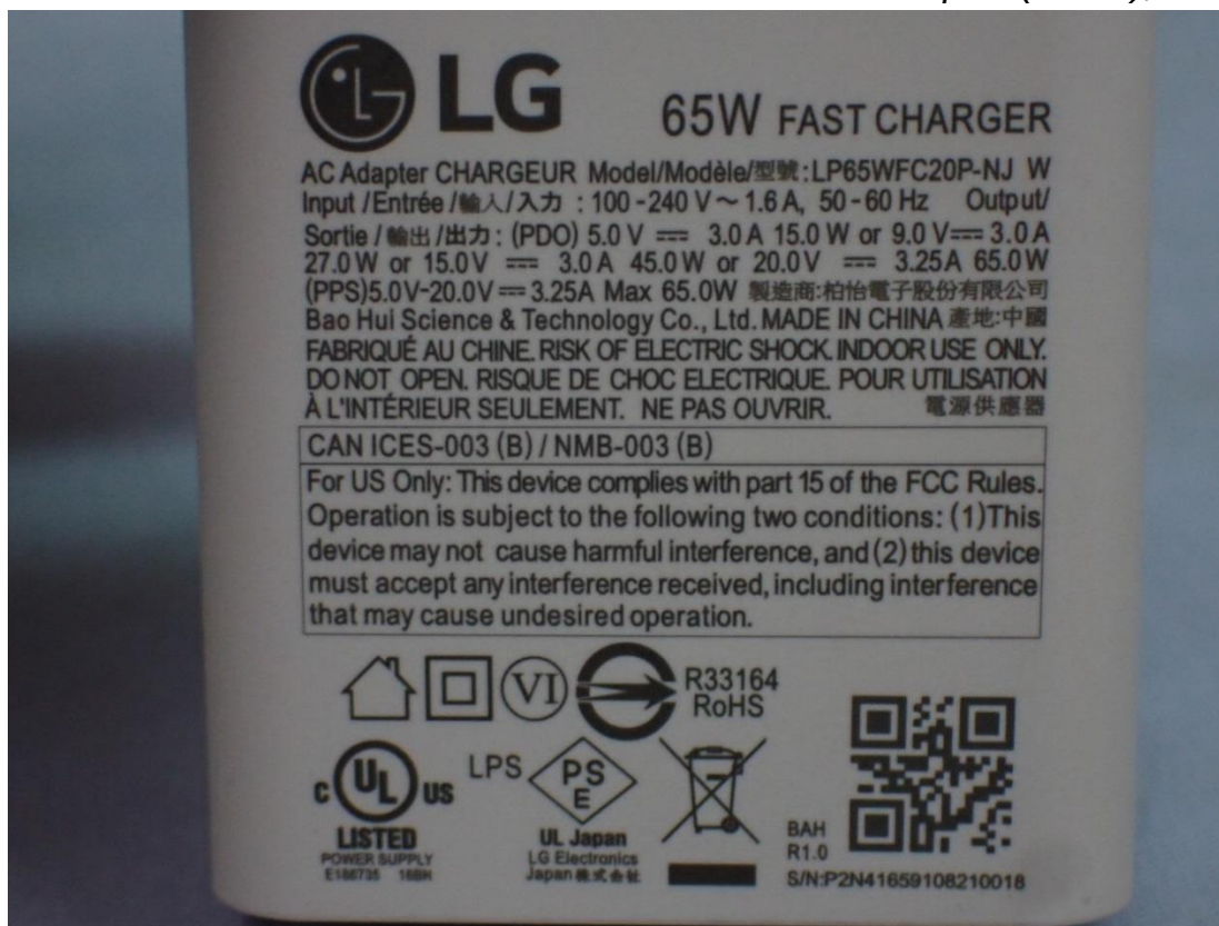
Figure 25 AC Adapter (White), Label View
