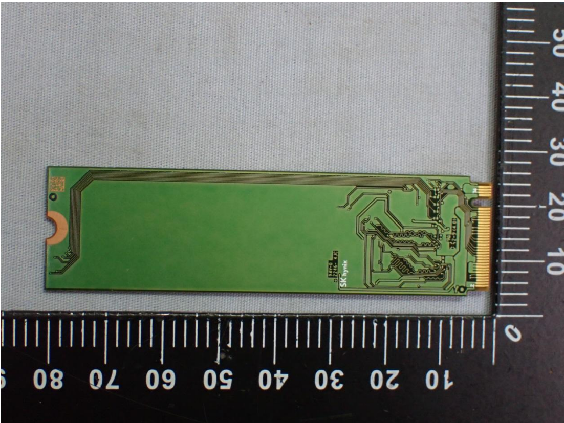
Figure 53 Worse SSD#1 View
