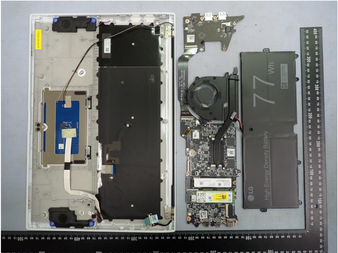
Figure 33 Internal View (Removed Components)
