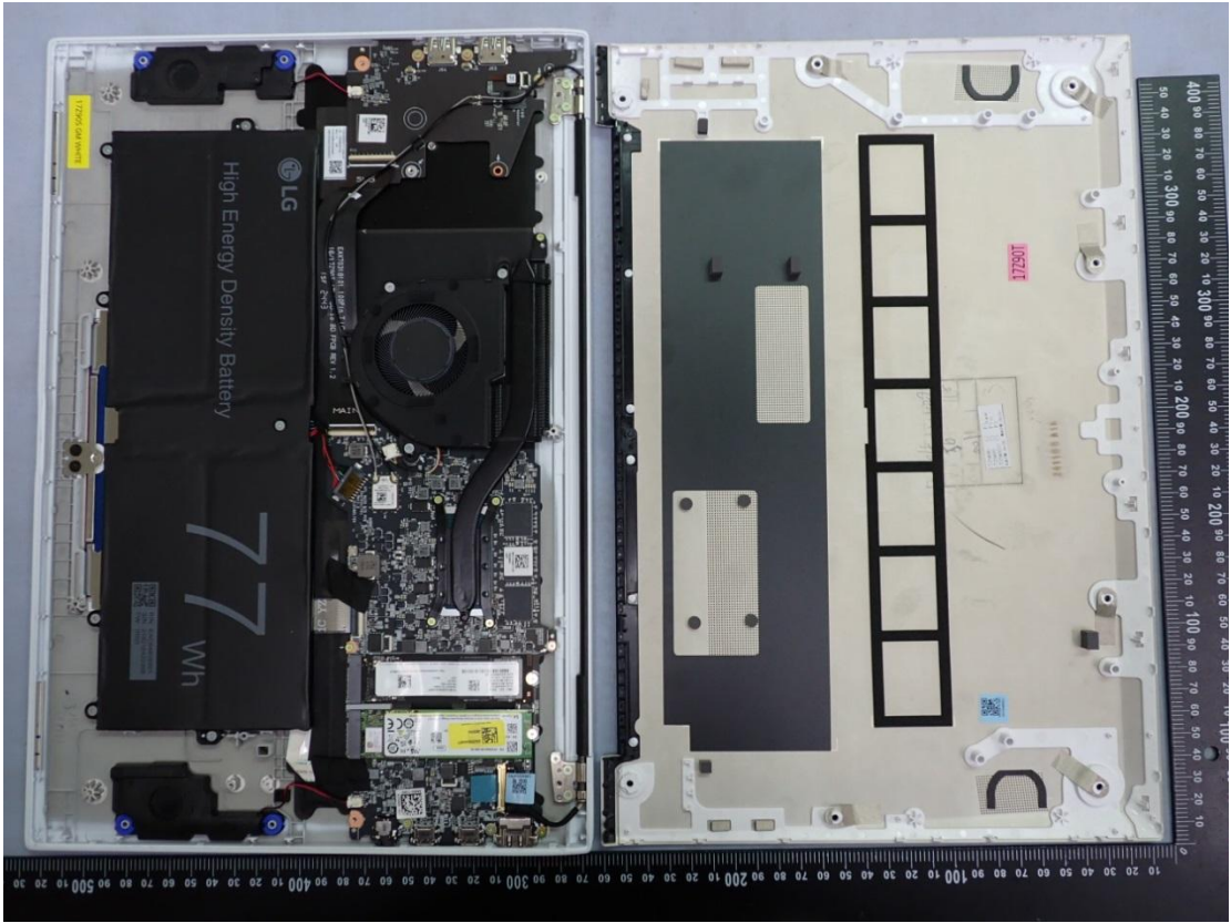
Figure 32 Internal View
