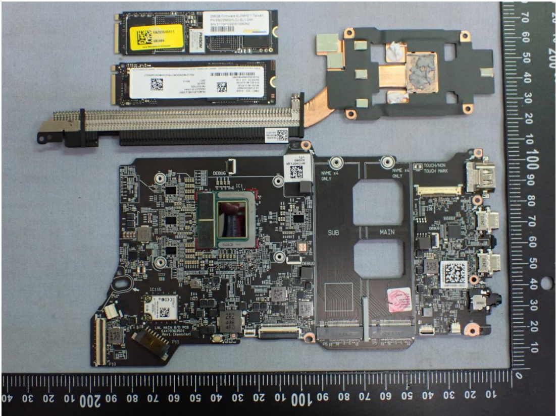
Figure 41 Internal View
