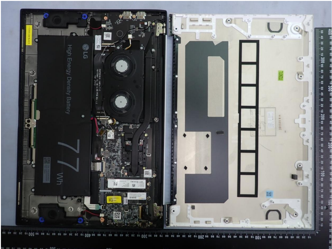
Figure 39 Internal View
