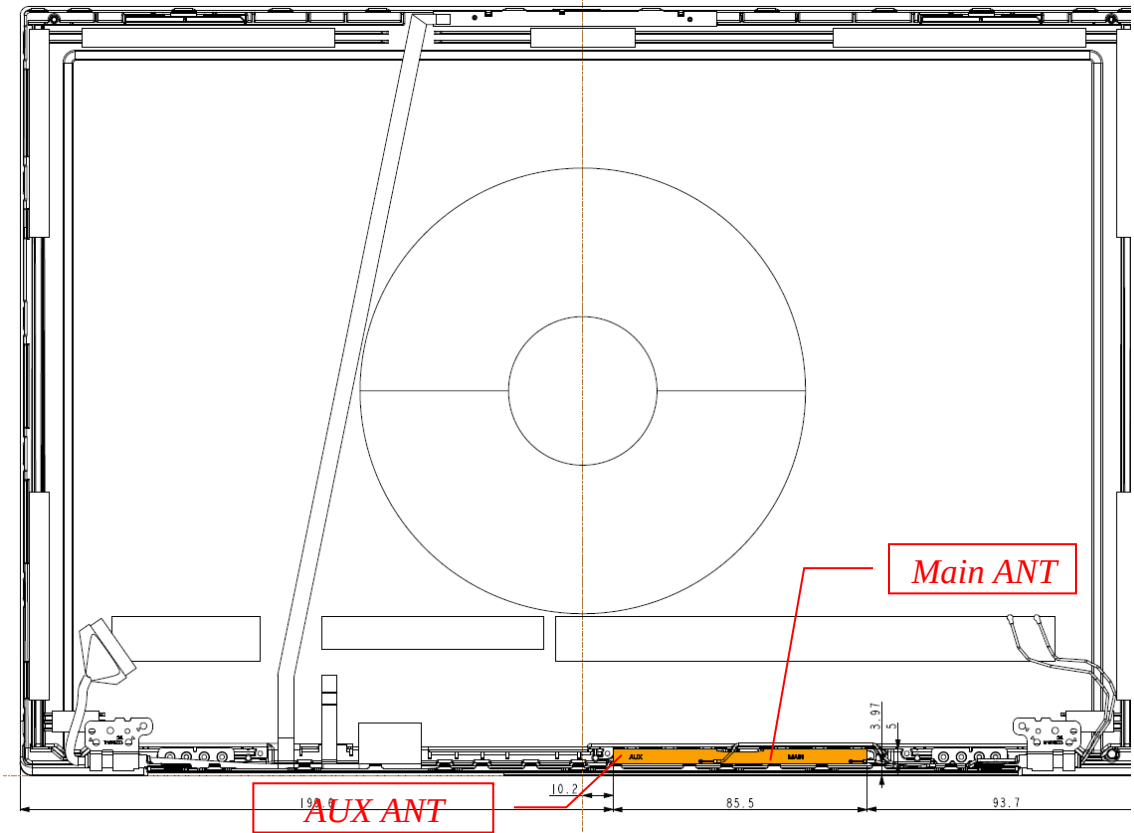
Figure 50 INPPAQ WLAN Combo Antenna Position
