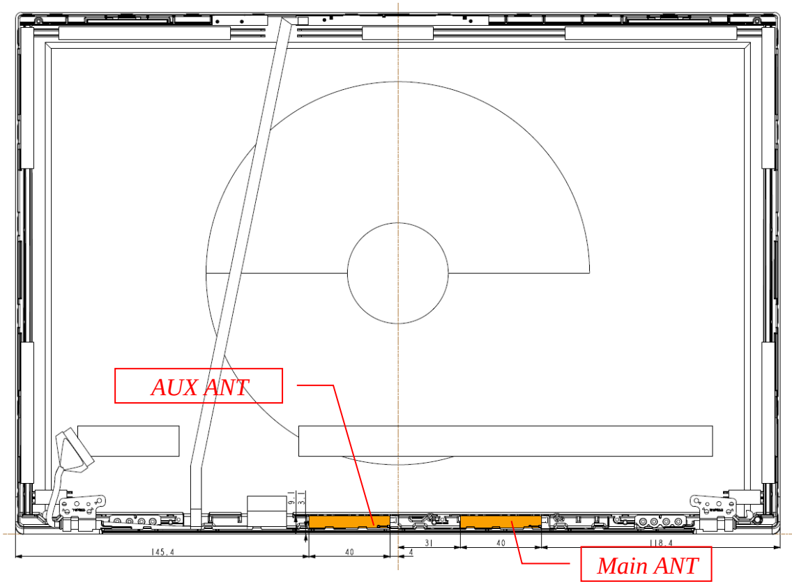
Figure 48 LUXSHARE-ICT WLAN Combo Antenna Position
