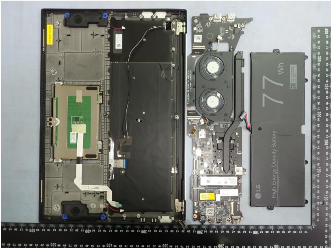
Figure 40 Internal View
