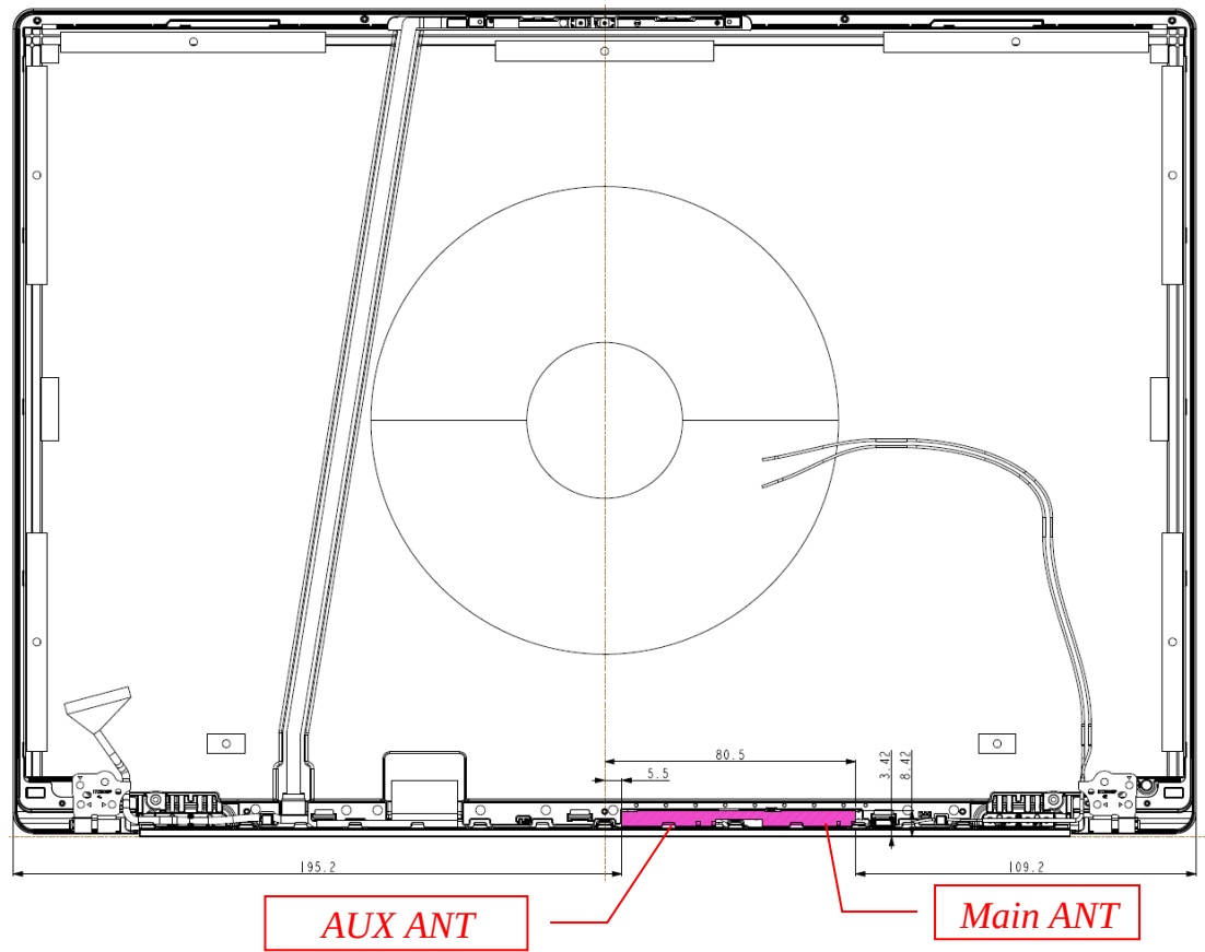
Figure 40 WLAN Combo Antenna Position
