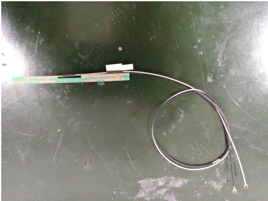
Figure 42 WLAN Combo Antenna, Back View
