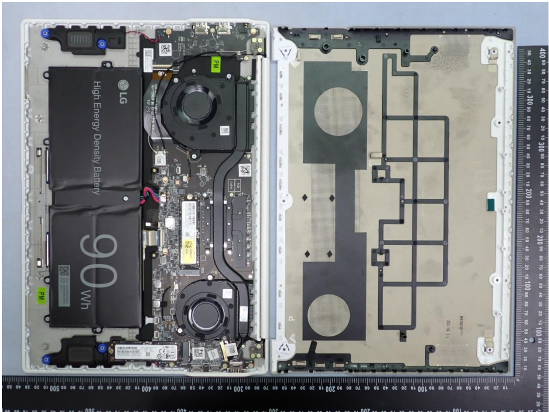
Figure 32 Internal View
