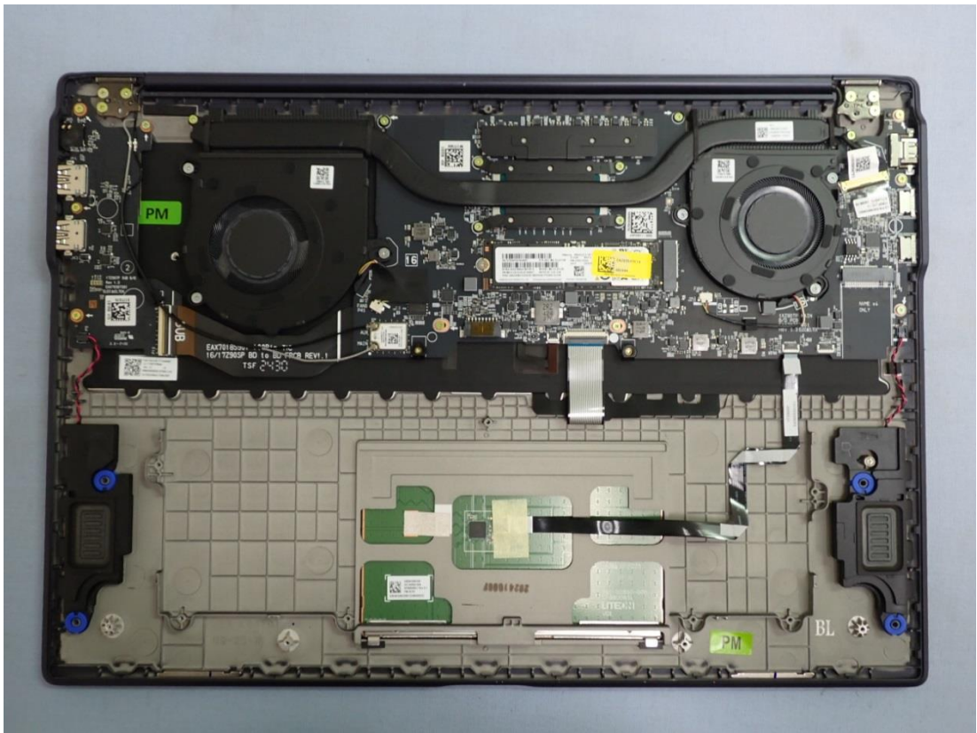
Figure 33 Internal View
