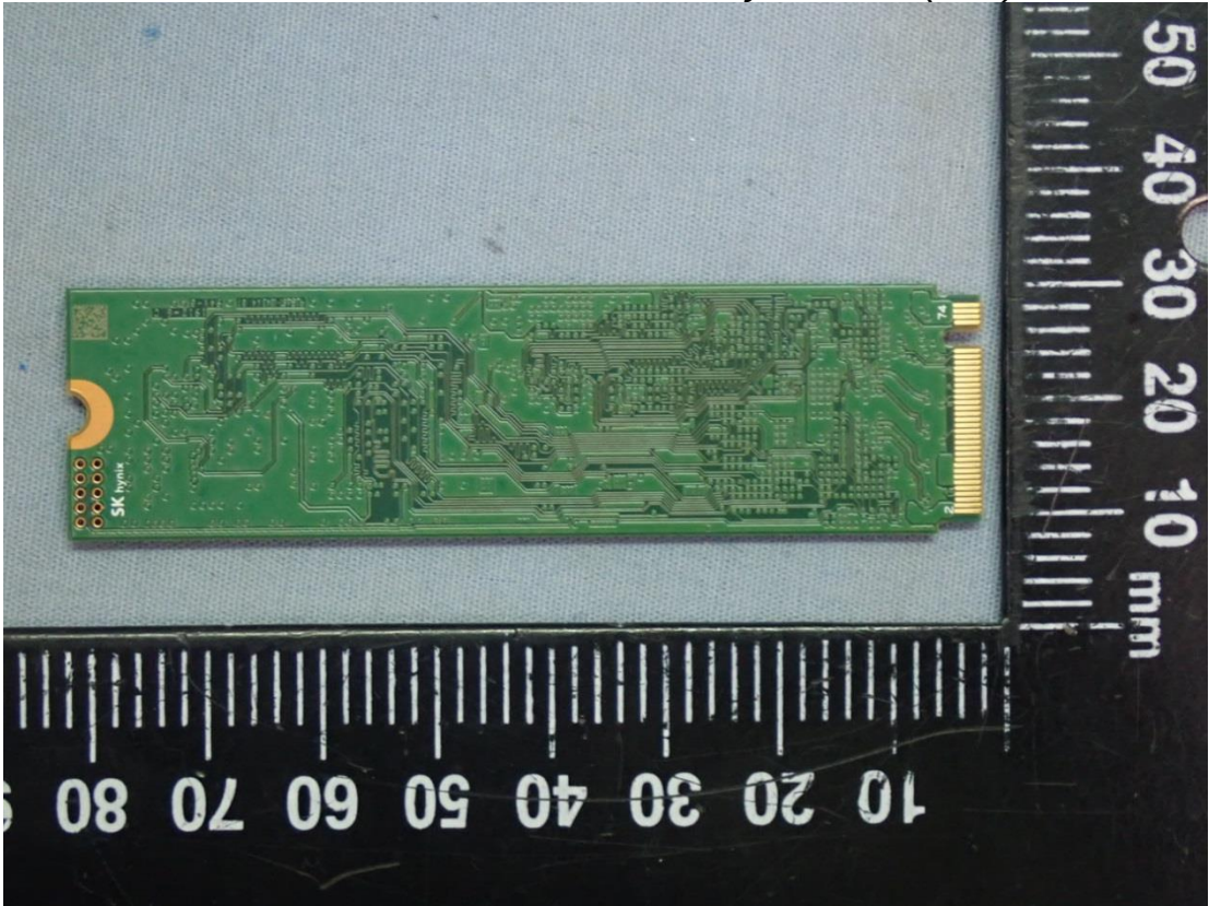
Figure 65 SK hynix, SSD (1TB), Back View
