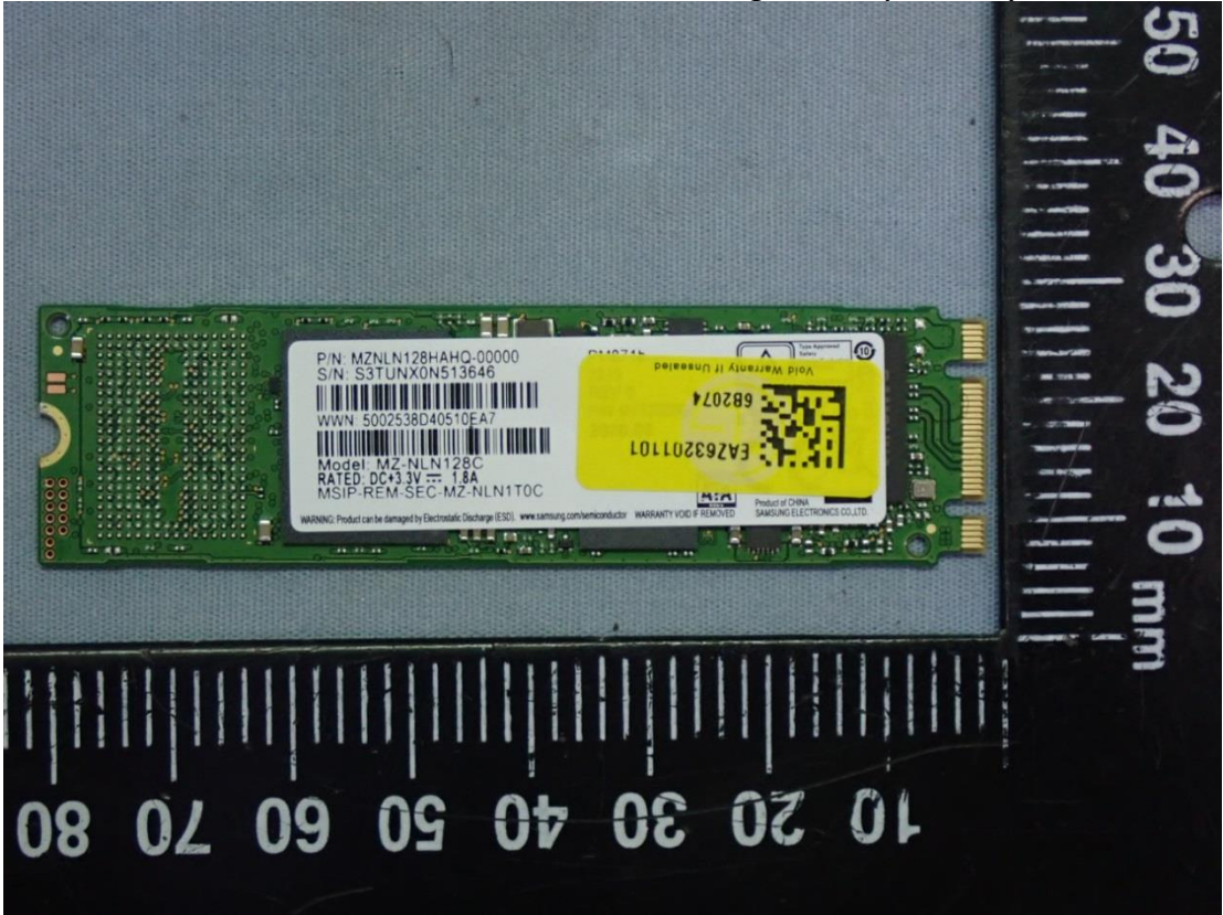
Figure 58 Samsung, SSD (128GB), Front View
