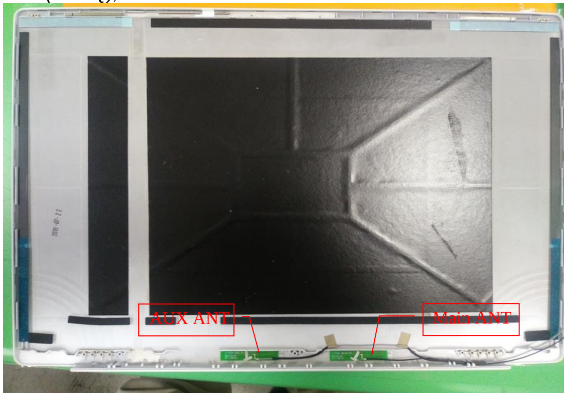
Figure 52 LG (INPAQ), M/N WA-P-LBLB-04-068 WLAN Combo Antenna Position
