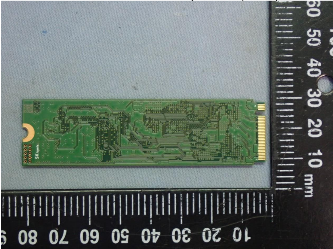
Figure 61 SK hynix, SSD (256GB), Back View
