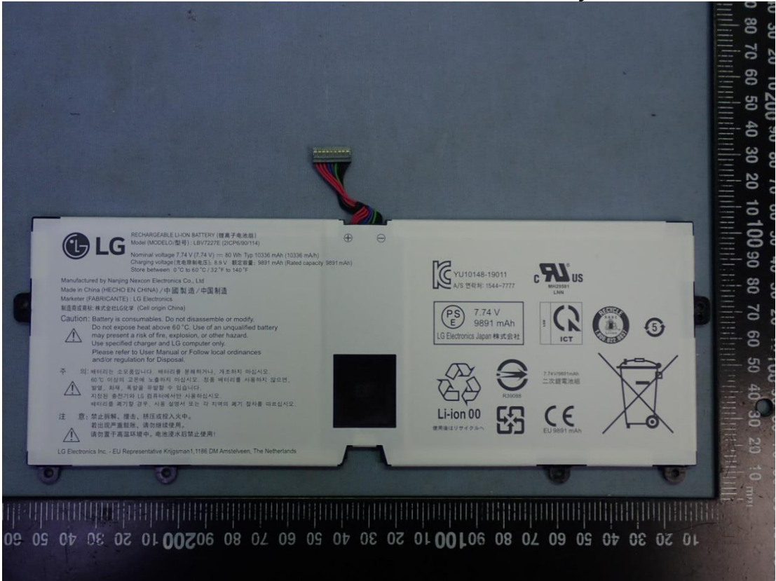
Figure 57 Battery Pack, Back View
