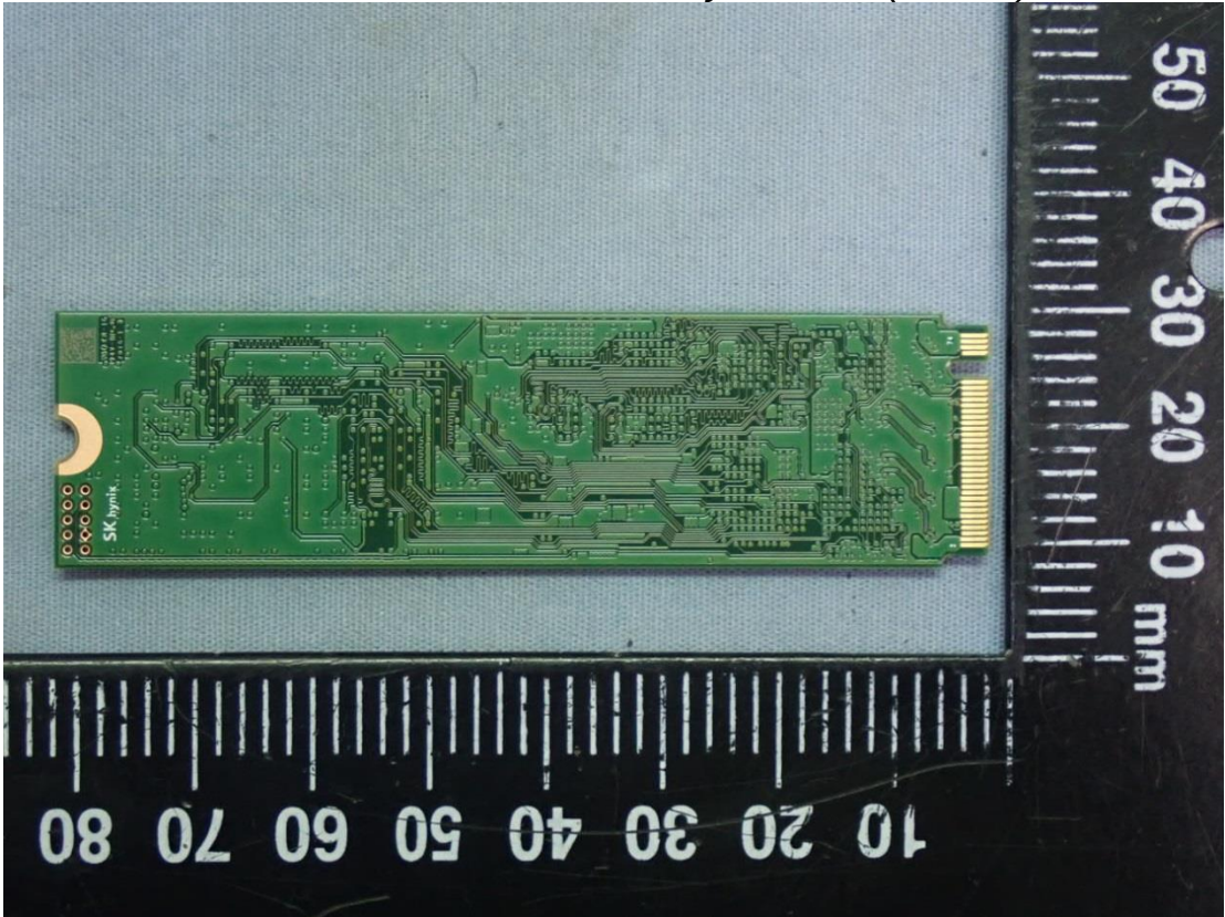
Figure 63 SK hynix, SSD (512GB), Back View
