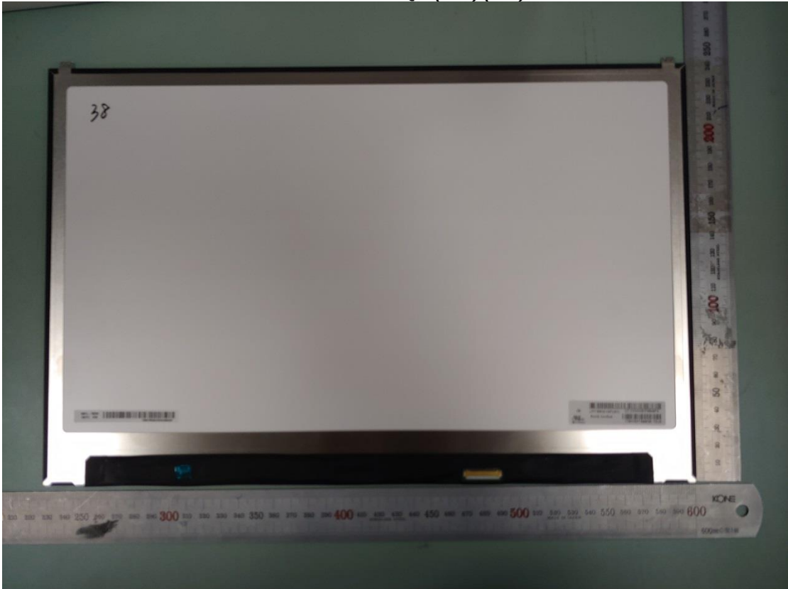
Figure 50 LGD, M/N LP170WQ1(SP)(A1), LCD Panel, Back View
