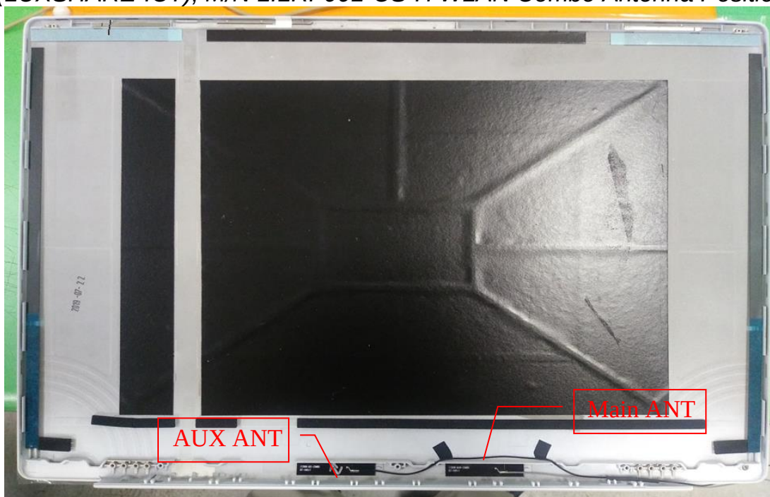
Figure 54 LG (LUXSHARE-ICT), M/N LILRF001-CS-H WLAN Combo Antenna Position
