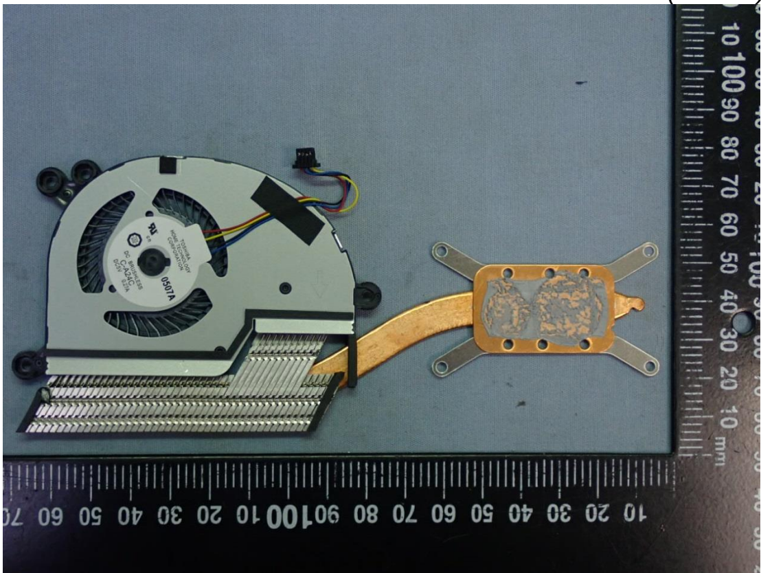
Figure 48 Internal View (DC Fan)
